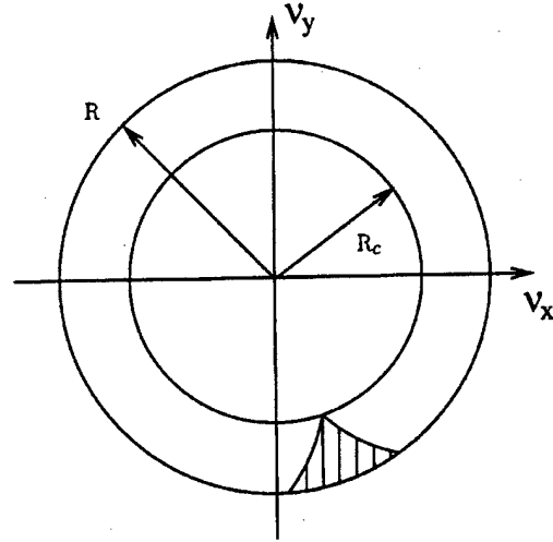
Fig. 3. The 2-D Fourier space coverage of the scattering object that is obtained by varying \phi from 0 to \Phi^c . The disk of Fourier space coverage with radius R = \nu_0\sqrt{1+1/\chi^2} is incomplete, with the shaded region denoting the missing data. However, the coverage corresponding to the disk of radius R_c , which is defined by (5), is completely specified. In generating the figure, \Phi^c = 230^\circ and \chi = 1 were utilized.
