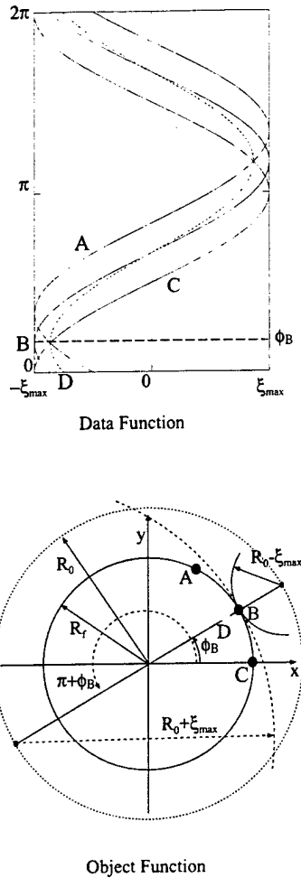
Fig. 1. Schematic of data function (top) and two-dimensional object function (bottom) for the heuristic potato peeler perspective. Points A , B , and C lie on the outermost ring of the object support, and their loci in the data space are also shown. The illustrated integration arcs from opposing views \phi_B and \phi_B + \pi intersect the support disk at B . When the outermost ring along with points A , B and C are removed, D becomes a point on the outermost edge.
