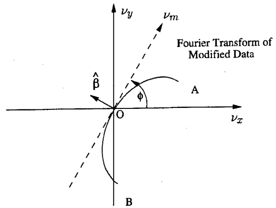
Fig. 2. The fan-beam FDP theorem states that M(v_m, \phi) is equal to the 2D Fourier transform of a(\mathbf{r}) along the semielliptical arc AOB that has semi-axes equal to v_0 and v_0/\chi .
