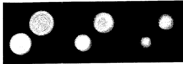
Fig. 4. Transverse slices reconstructed from the spherical-wave data function ( \chi = 0.7 ) using a plane-wave DT reconstruction algorithm. As expected, the images contain distortions.
