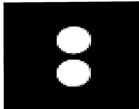
Figure 8. The geometry of the two component scattering object. We considered the cases where the refractive index of the uniform cylinders took the values n(\vec{r}) = 1.01, 1.05, \text{ and } 1.08 .
