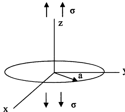
Figure 2.5: Flat, internal penny-shaped crack subjected to remote tension.
