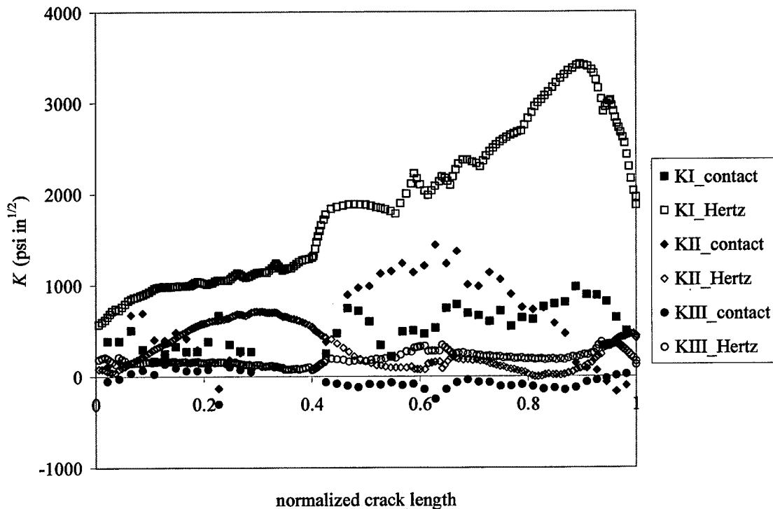
Figure 3.9: Comparison of mode I, II and III SIFs calculated by three-dimensional finite element contact analysis and finite element analysis with Hertz contact loads for a pinion with crack #2 and at a double tooth contact configuration.
