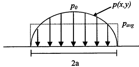
Figure 2.1: Representation of Hertz stress over an elliptical area.
