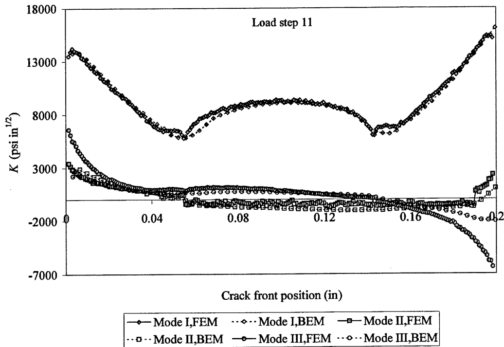
Figure 2.17: Comparison of initial Mode I, II and III SIFs computed by the FEM and the BEM for load step 11.
