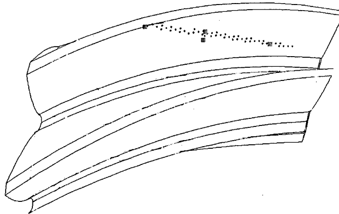
Figure 3.6: Comparison of location of contact loads by Hertzian analysis and FE contact analysis for double-tooth contact at initial crack. Hertzian load on tooth 1 corresponds to load step 11.
