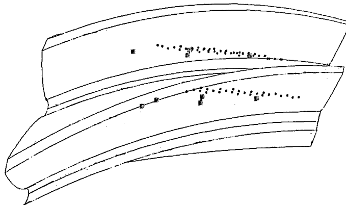
Figure 3.5: Comparison of location of contact loads by Hertzian analysis and FE contact analysis for double-tooth contact at initial crack. Hertzian loads on tooth 1 and tooth 2 correspond to load step 3 and load step 13, respectively.
