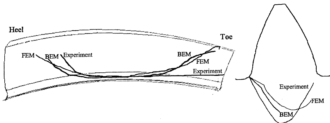
Figure 2.20: Comparison of crack trajectory predicted by the BEM, the FEM and an experiment on the tooth surface and tooth cross section at the midpoint of crack.
