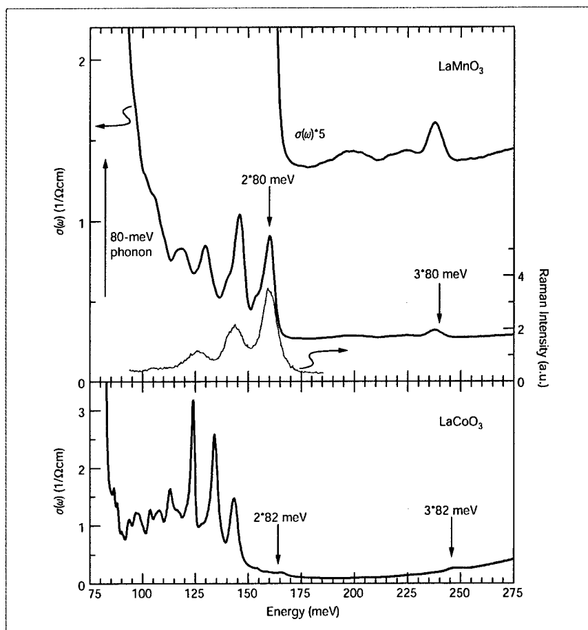
Figure 1 Optical conductivity \sigma(\omega) of LaMnO 3 and LaCoO 3 , and Raman measurements on LaMnO 3 , at a temperature of 4 K. Top, comparison of \sigma(\omega) (thick blue line) and Raman intensity (from Saitoh et al. 1 ; thin yellow line) of LaMnO 3 , reveals a close similarity between the two spectra. In \sigma(\omega) the highest peaks of single-, two- and three-phonon absorption are observed at 80, 160 and 240 meV, respectively. Inset, enlargement of the three-phonon range of \sigma(\omega) . Bottom, \sigma(\omega) of LaCoO 3 , showing multiphonon peaks, for example at 2*82 and 3*82 meV.
