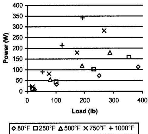
Figure 18 – Power consumption of C-core #2 at zero RPM.
