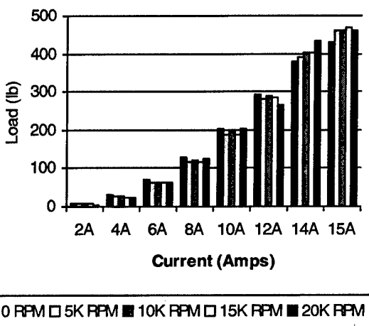
Figure 9 – C-core #1 load as a function of rotor speed for bearing currents up to 15 amps.
