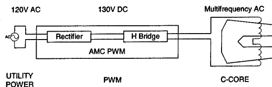
Figure 11 – Power system for one C-Core.
