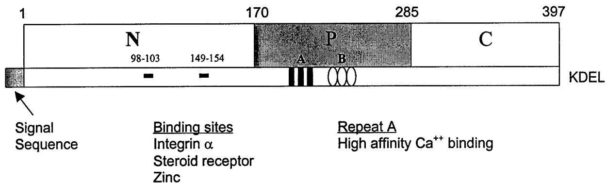
Fig. 1. The domain structure of calreticulin. (Baksh and Michalak, 1996). The N-domain (aa 1-170) of calreticulin is the most conserved domain in evolution and does not bind to Ca ++ . The N-domain forms a globular domain with 2 regions of short \alpha -helices at residues 98-103 and 149-154, which are responsible for the binding to integrin \alpha and the DNA binding domain of steroid receptors. The P-domain (aa 171-285) is proline-rich and contains two sets of repeats (Repeat A and Repeat B). Repeat A consists of three repeats of aa sequence PXXIXDPDAXKPEDWDE and is believed to be responsible for high affinity (Kd = 1.6 \mu M) and low capacity (1 Ca ++ /protein) Ca ++ binding to calreticulin. Repeat B consists of three aa sequence GXWXPPXIXNPXYX and is predicted to have a rigid turn structure separating the globular head of the protein from the acidic tail. The C-domain (aa 286-397) is highly acidic and negatively charged. This large stretch of negatively charged residues binds Ca ++ with low affinity (Kd = 0.3-0.2 mM) and high capacity (~25 Ca ++ /protein). These high capacity low affinity Ca ++ binding sites have led to the hypothesis that calreticulin is involved in luminal Ca ++ storage. The C-domain in calreticulin has the most divergent aa sequence among different species.
