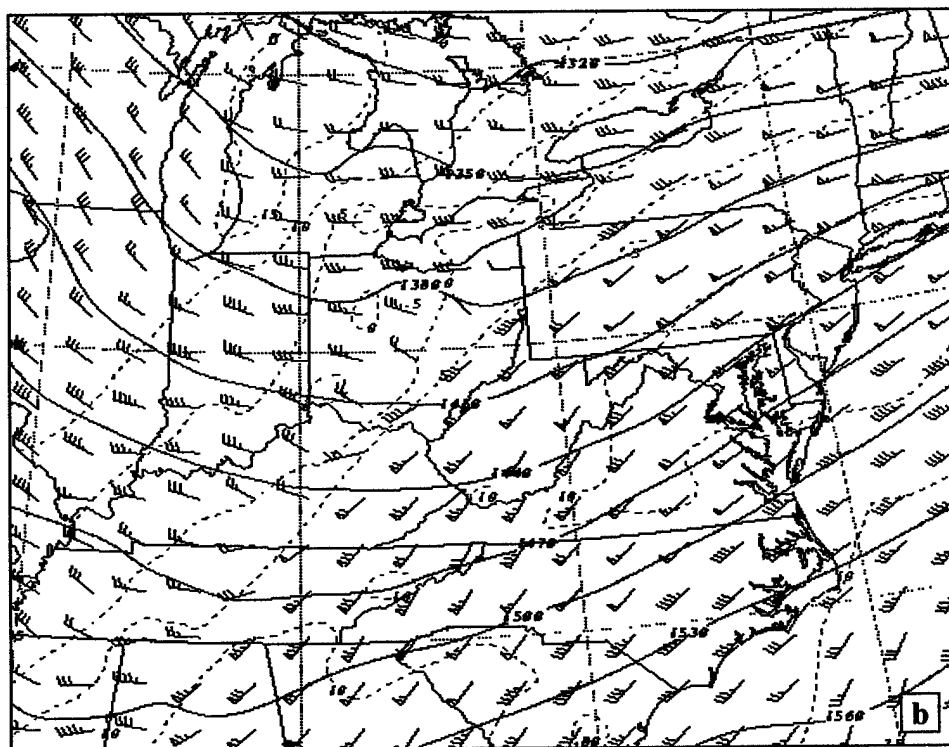
Figure 16. 850 hPa height (m), temperature ( ^{\circ}\text{C} ), and wind (kt) valid 1200 UTC 28 Dec 1988. (a) NWS analysis, (b) 30-km control simulation.
