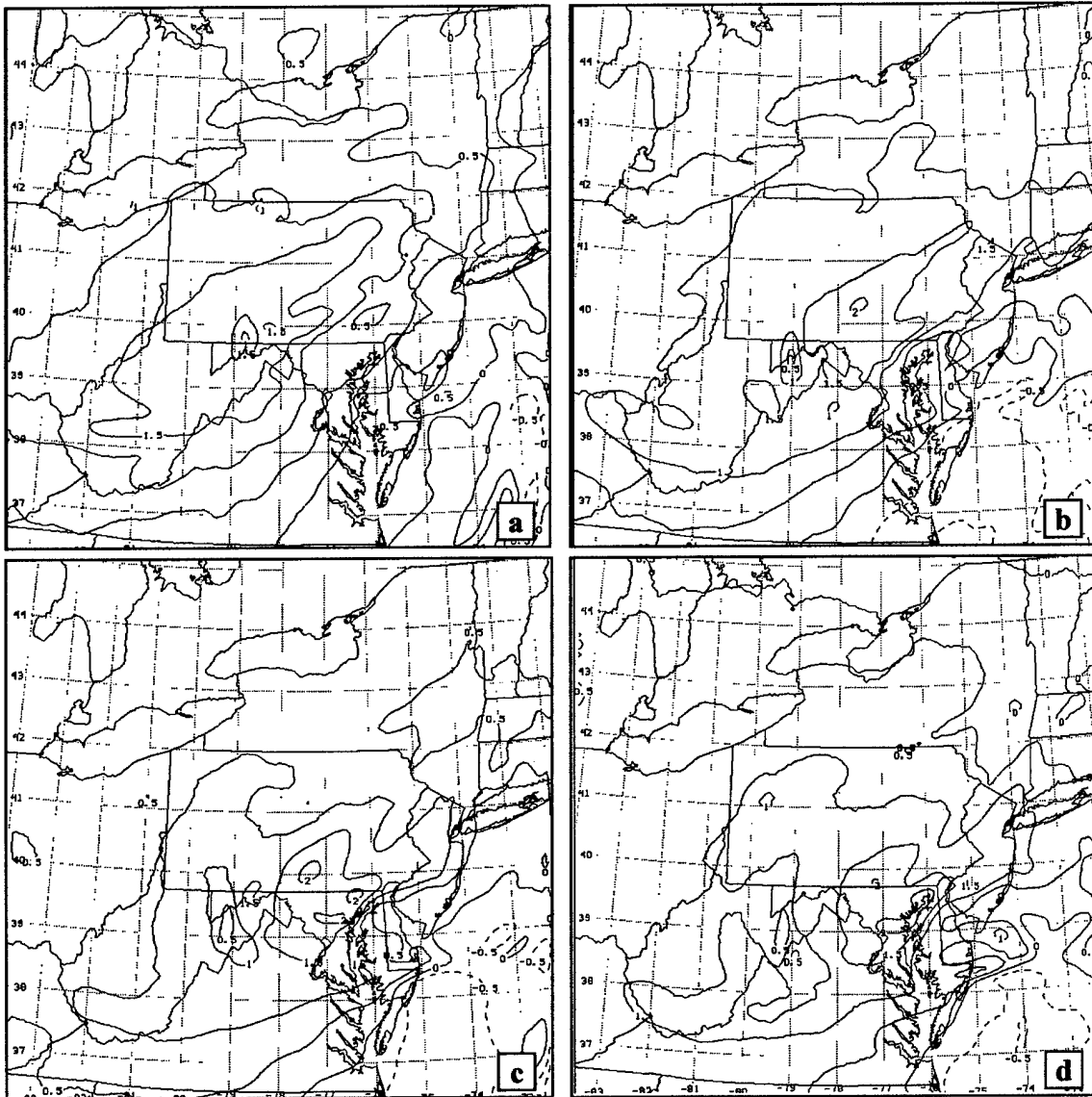
Figure 27. Simulated half-hour pressure changes valid 13 Jan 2000 (a) 1800-1830 UTC, (b) 1900-1930 UTC, (c) 1930-2000 UTC, (d) 2000-2030 UTC.
