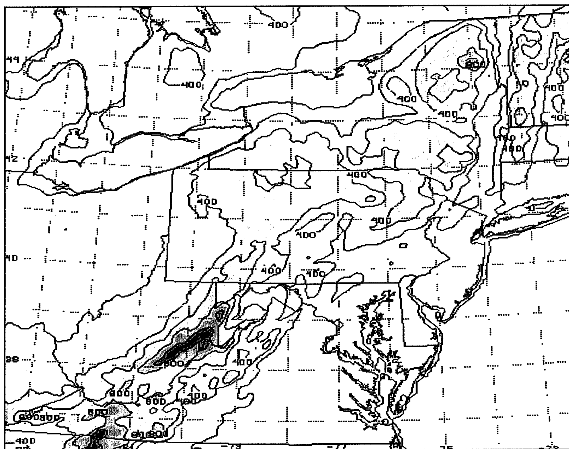
Figure 14. 6-km NHMASS terrain (m). Contours are 100m (filled) and 200m (lined).
