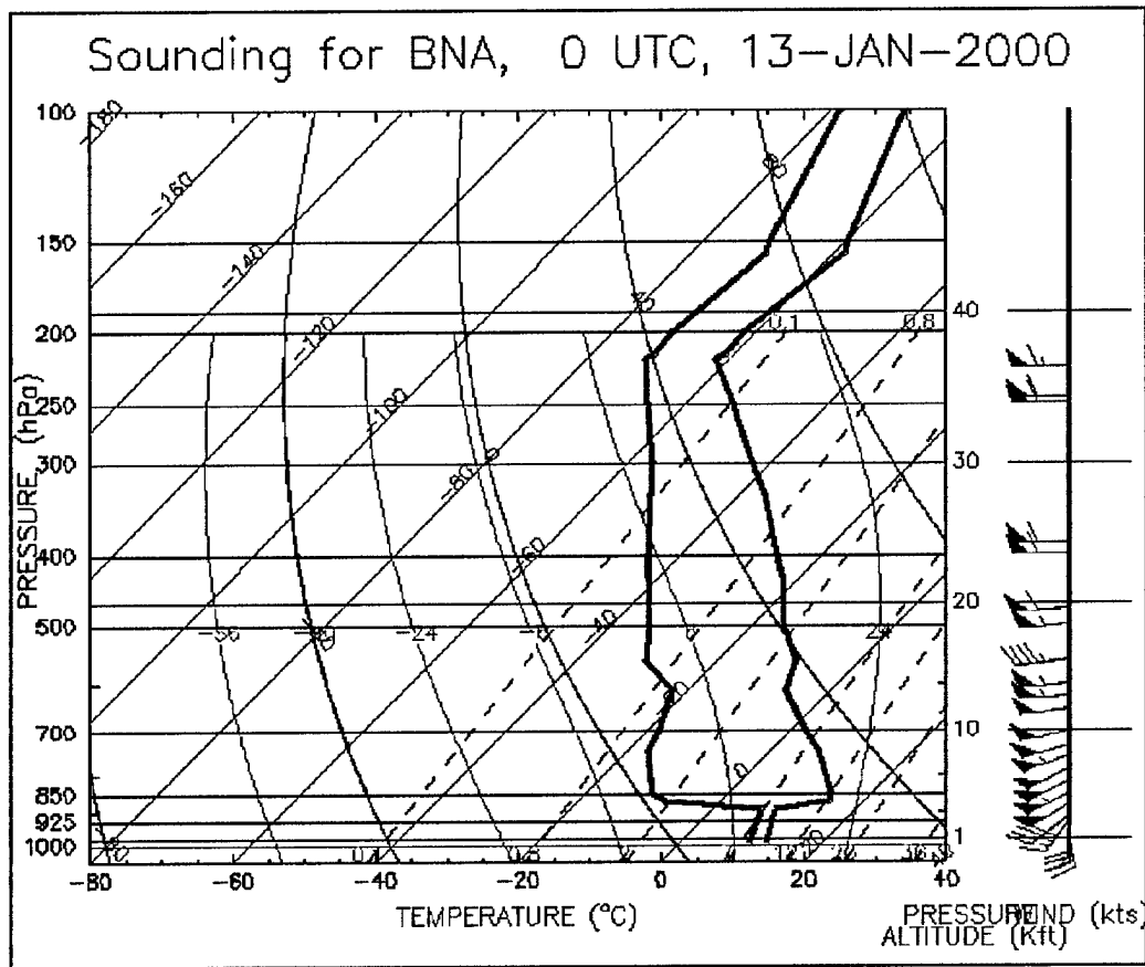
Figure 41. Nashville, TN Skew-T (KBNA) Valid 00 UTC 13 Jan 2000.
