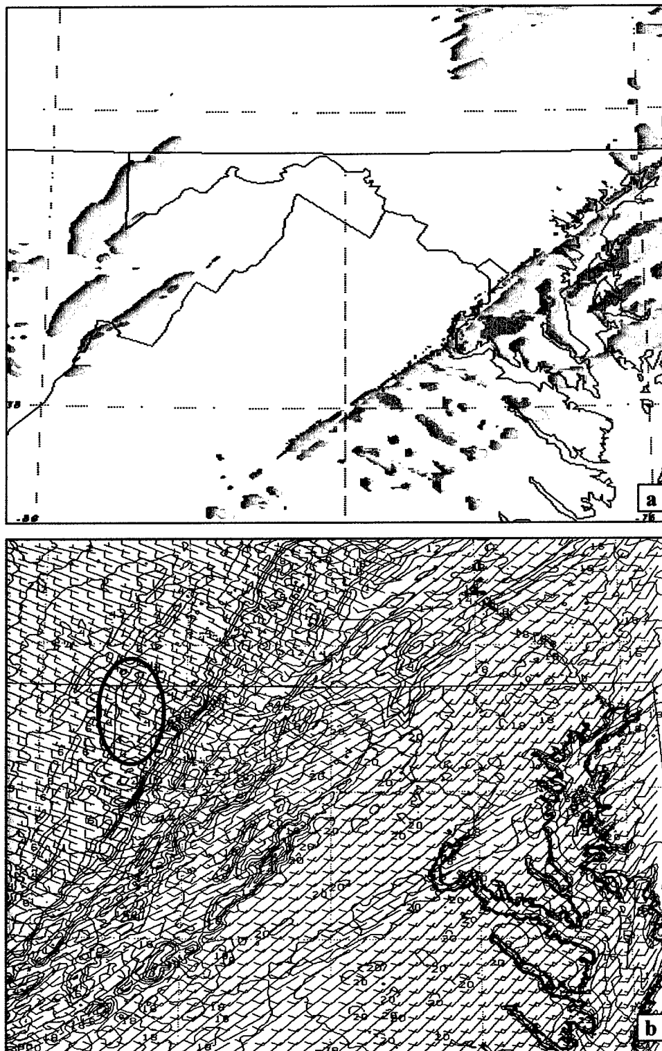
Figure 35. (a) Simulated precipitation (mm/hr) valid 1730 UTC 28 Dec 1988 and (b) simulated surface temperature ( ^{\circ}\text{C} ) and wind ( \text{ms}^{-1} ) valid 1730 UTC 28 Dec 1988. The 4 ^{\circ}\text{C} cool pool is encircled.
