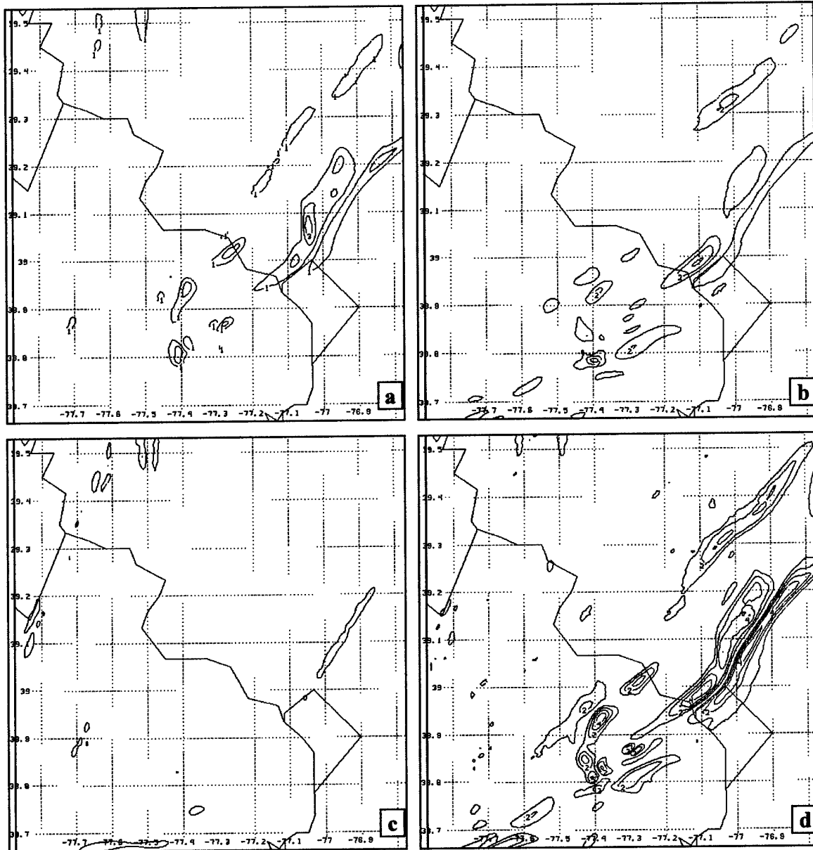
Figure 18. Valid 1930 UTC 28 Dec 1988. 500-m NHMASS (a) 2400m X-space vorticity tendency ( \times 10^{-5} \text{ s}^{-2} ), (b) 2400m Y-space vorticity tendency ( \times 10^{-5} \text{ s}^{-2} ), (c) 2400m Z-space vorticity tendency ( \times 10^{-5} \text{ s}^{-2} ), (d) 2400m total vorticity tendency ( \times 10^{-5} \text{ s}^{-2} ).
