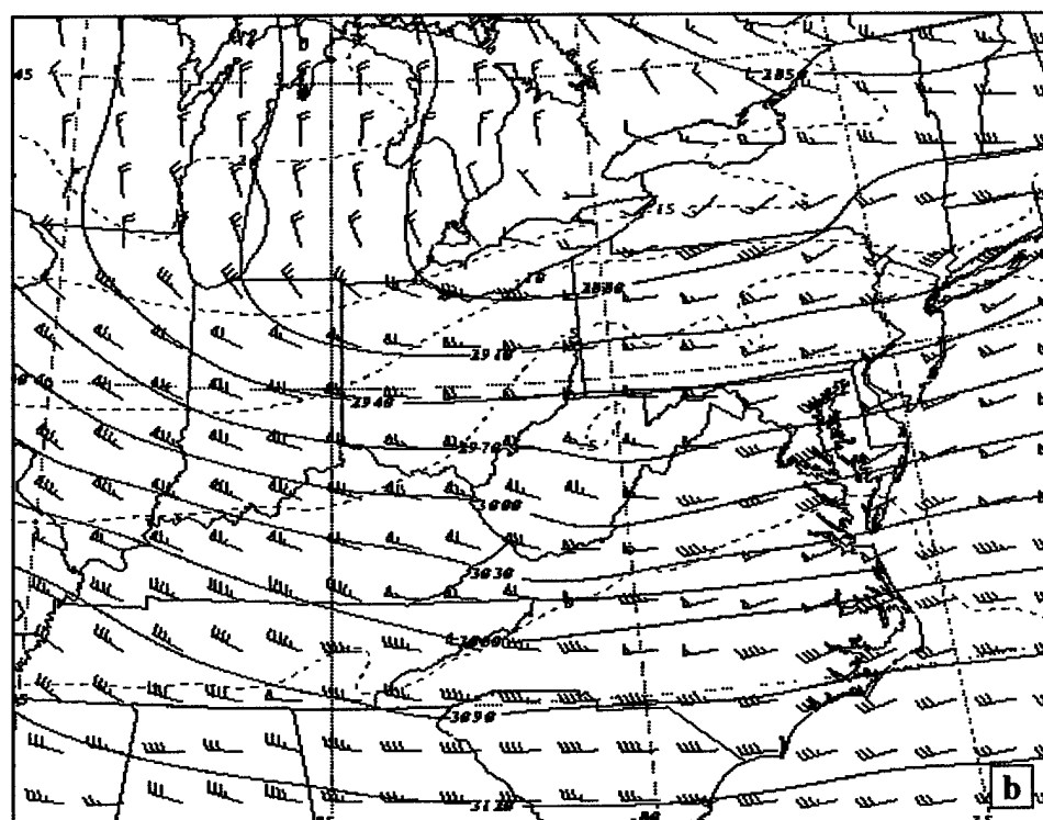
Figure 20. 700 hPa height (m), temperature ( ^{\circ} C), and wind (kt) valid 1200 UTC 13 Jan 2000. (a) NWS analysis, (b) 30-km control simulation.
