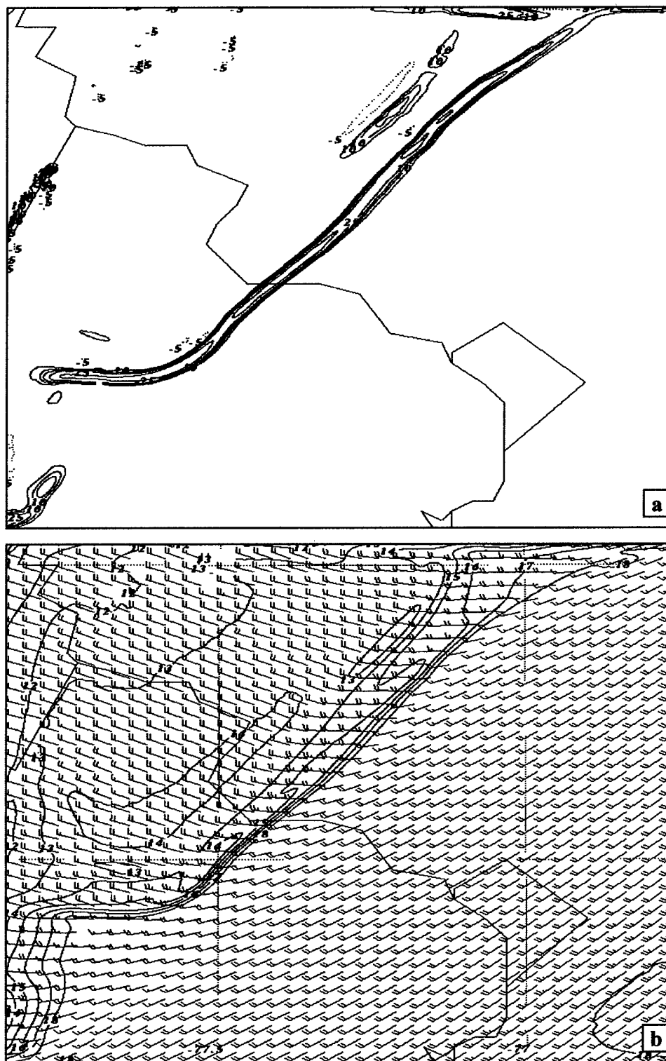
Figure 1. (a) 970 hPa frontogenesis (deg C/100km/3hr) valid 1900 UTC 28 Dec 1988, (b) 970 hPa temperature ( ^{\circ}\text{C} ) contoured every degree and wind ( \text{ms}^{-1} ) valid 1900 UTC 28 Dec 1988.
