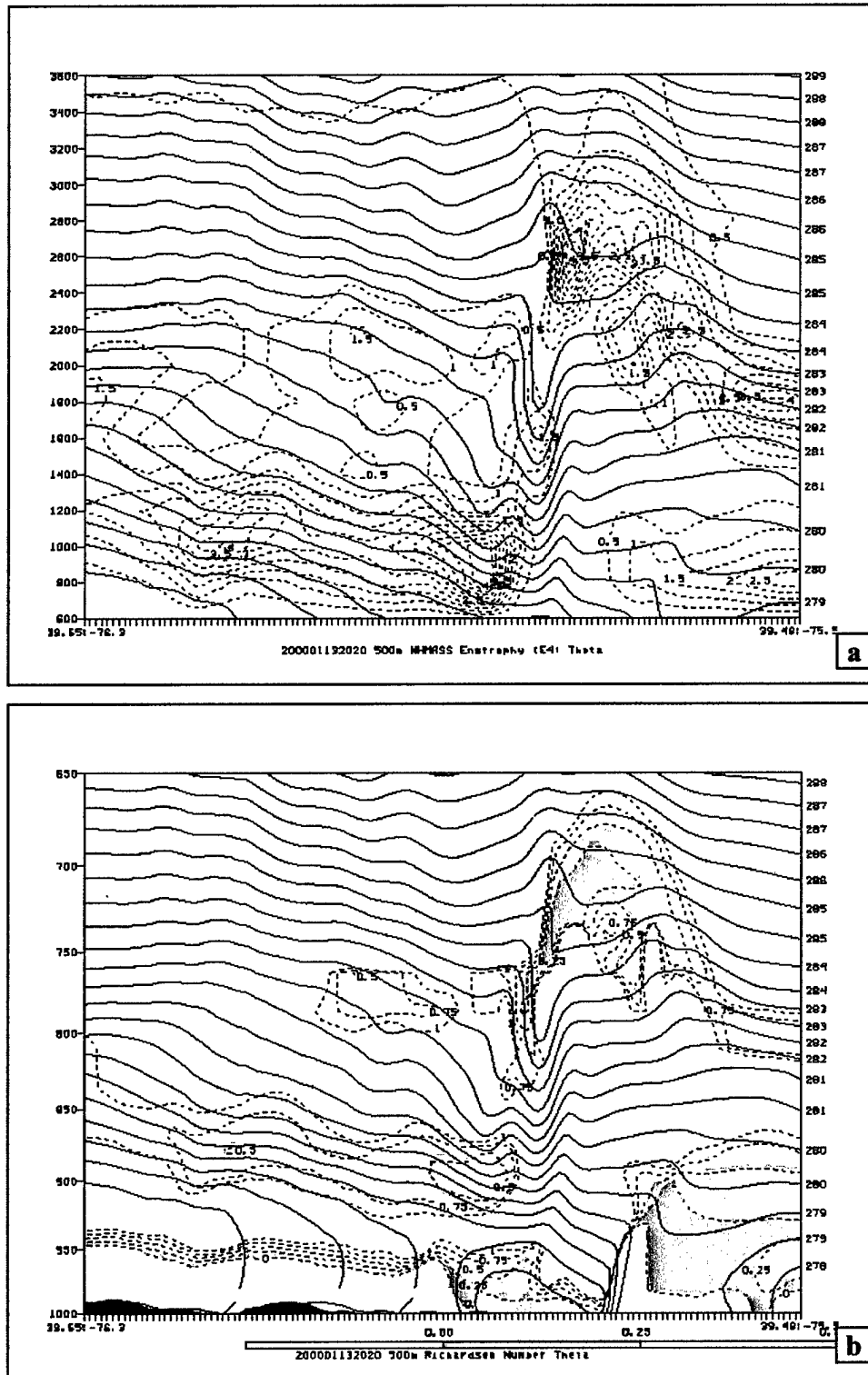
Figure 35. (a) Enstrophy ( \times 10^{-4} \text{s}^{-2} ), (b) Richardson number. Valid 2020 UTC 13 Jan 2000, (c) Enstrophy ( \times 10^{-4} \text{s}^{-2} ), (d) Richardson number. Valid 1930 UTC 28 Dec 1988. Enstrophy > 2 and \text{Ri} < 0.5 shaded.
