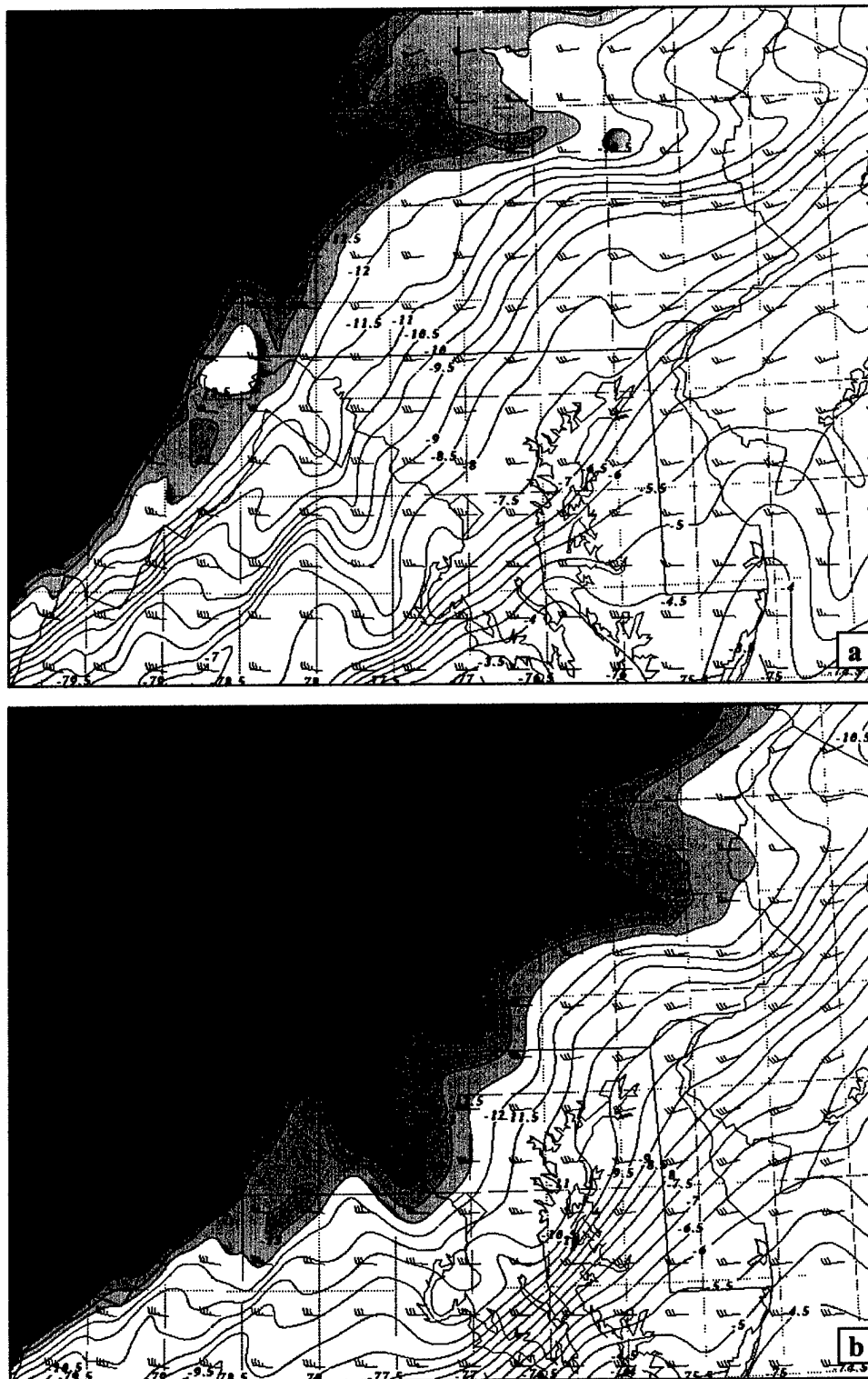
Figure 4. Simulated 700 hPa temperature ( ^{\circ}\text{C} ) and wind ( \text{ms}^{-1} ) valid (a) 1700 UTC 13 Jan 2000, (b) 1800 UTC 13 Jan 2000.
