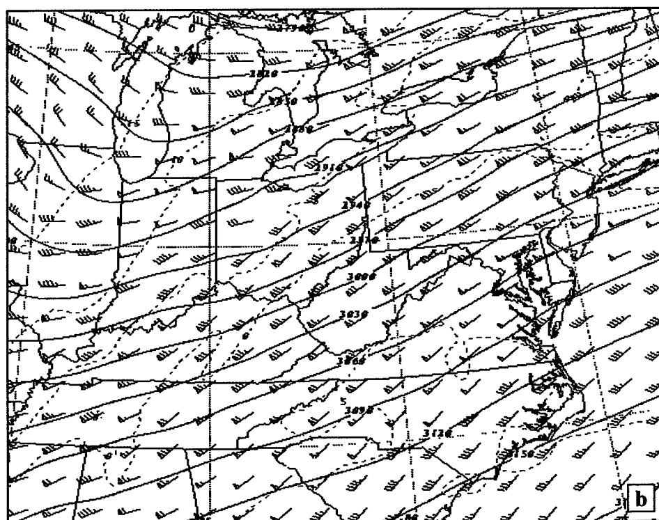
Figure 17. 700 hPa height (m), temperature ( ^{\circ}\text{C} ), and wind (kt) valid 1200 UTC 28 Dec 1988. (a) NWS analysis, (b) 30-km control simulation.
