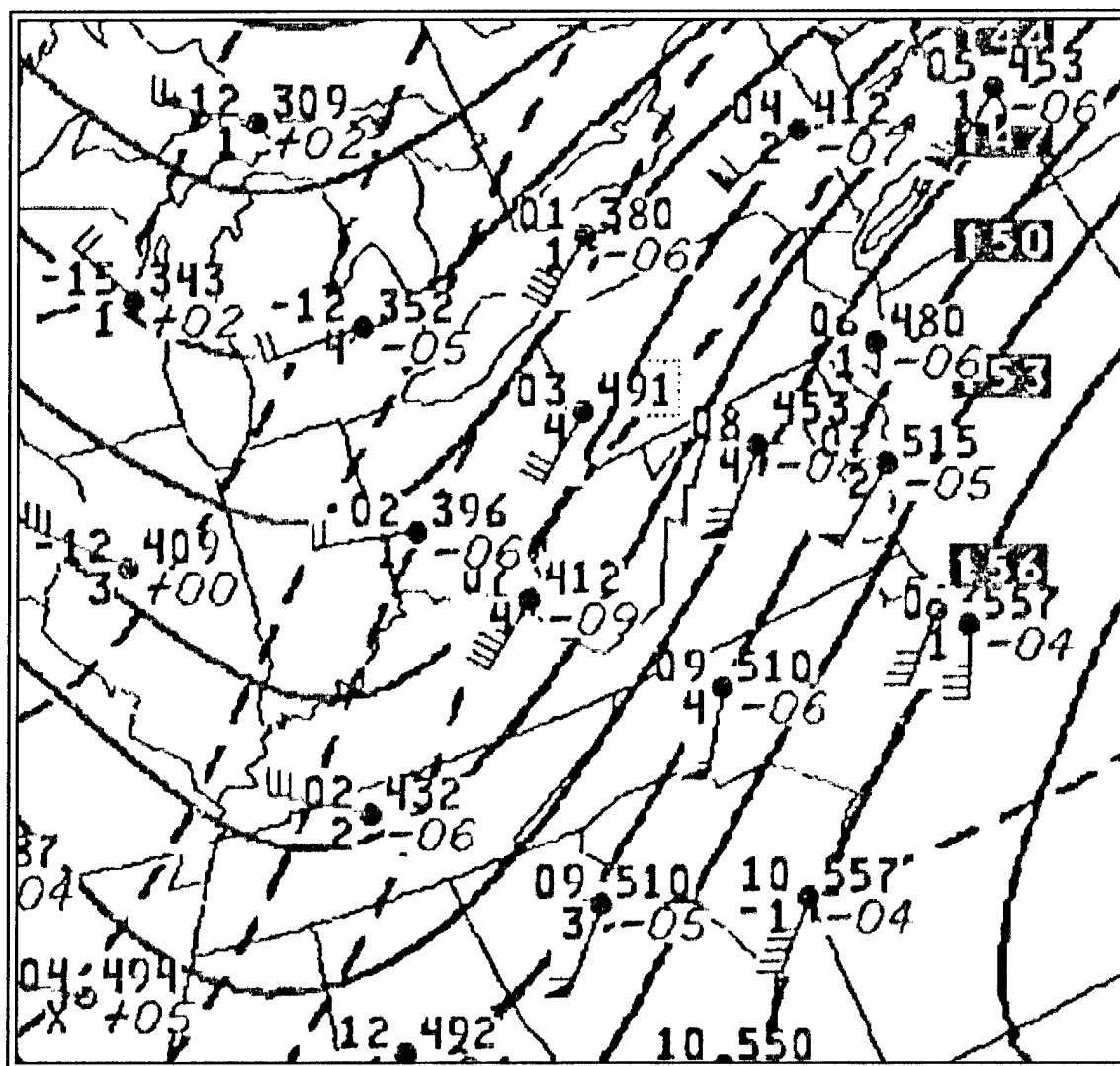
Figure 4. NWS 850 hPa analysis valid 1200 UTC 28 Dec 1988.
