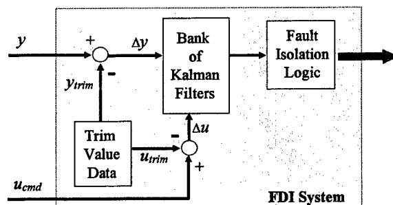
Figure 7. Structure of the FDI System
