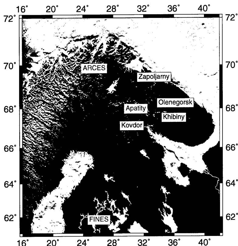
Fig. 6.2.1. Locations of the mining regions in NW Russia for which ground truth information is provided by KRSC. Also shown are the locations of the seismic arrays in the region (ARCES, Apatity and FINES).
