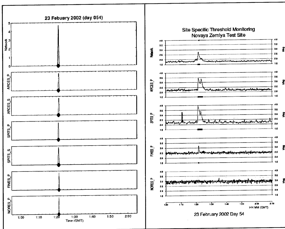
Fig. 6.3.3. SSGBF and SSTM for 23 February 2002, 01:00 - 02:00 GMT. See Fig. 6.3.2 for details. Notice the triangular shape of the SSGBF weight functions.
