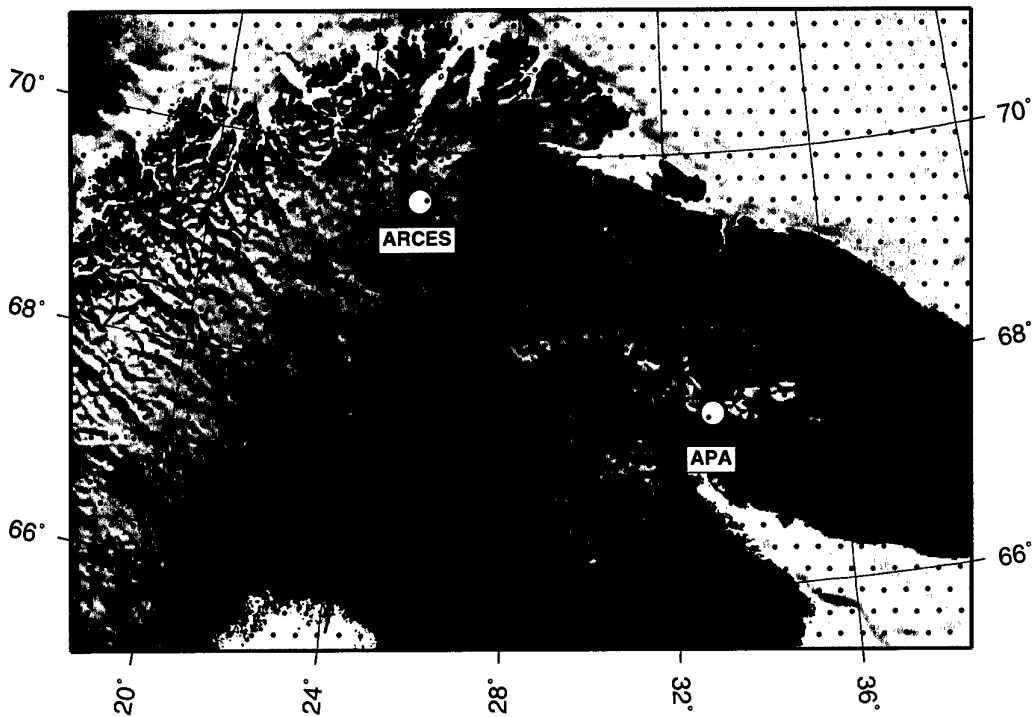
Fig. 6.5.2. Grid points used for regional threshold monitoring of the Kola Peninsula. The grid spacing is 0.2 degrees.
