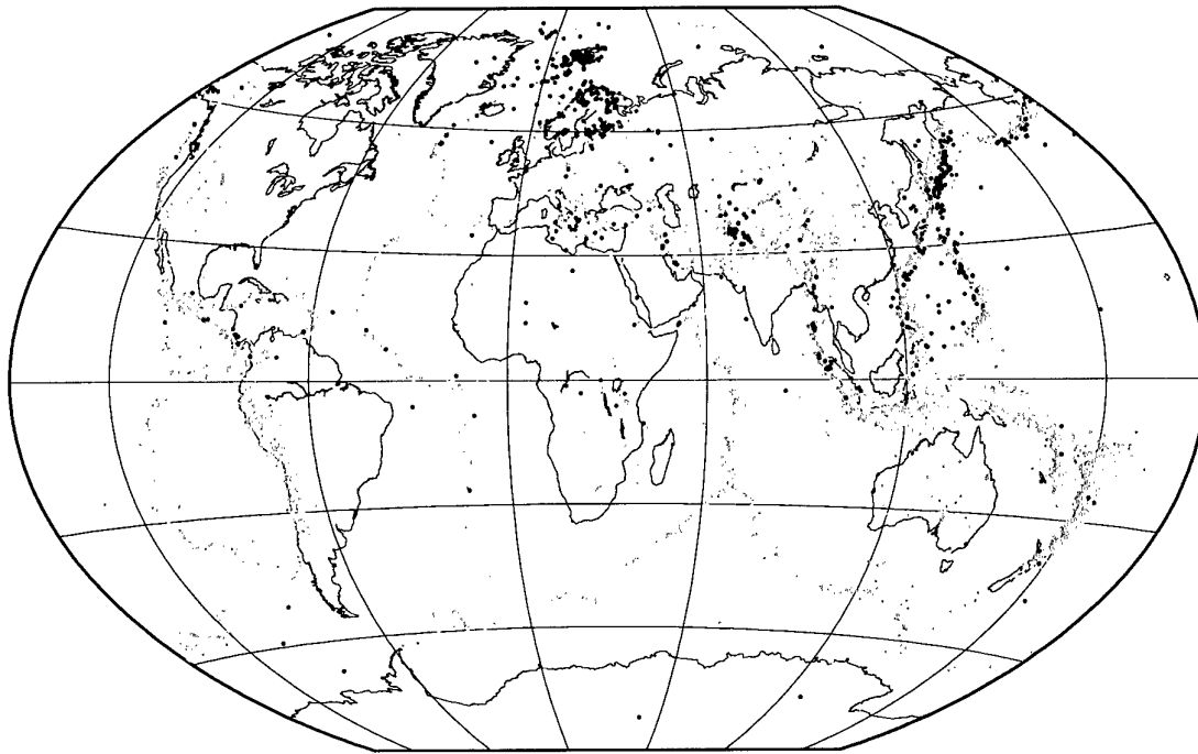
Fig. 4.4.1. Map with all 1220 NEWS locations (red) between 16 June and 31 December 2002 on top of all 10796 events (grey) as listed in the REBs of the same period.
