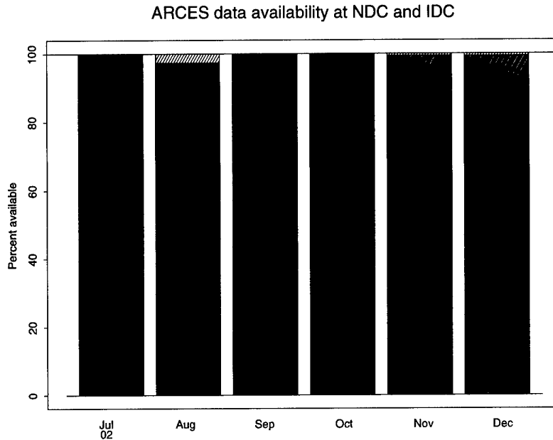
Fig. 4.2.2. The figure shows the monthly availability of ARCES array data for the period July - December 2002 at NOR_NDC and the IDC. See the text for explanation of differences in definition of the term "data availability" between the two centers. The higher values (hatched bars) represent the NOR_NDC data availability.
