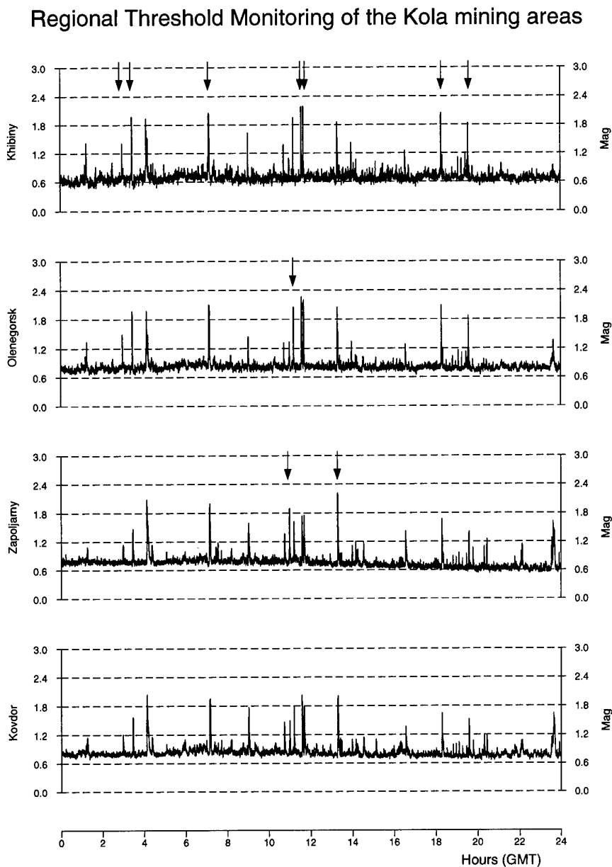
Fig. 6.5.9. Network magnitude thresholds for the grid points closest to the four mining areas Khibiny, Olenegorsk, Zapoljarny and Kovdor for 12 April 2002. During this day 10 events are found which are located in three of these mining areas, of which 6 are confirmed by KRSC. The corresponding mines and threshold peaks are indicated by red arrows.
