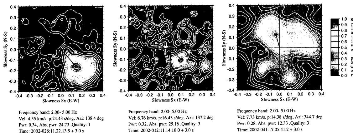
Fig. 6.2.6. Results of fk-analysis for the Sn time window for three events which passed the first two tests as indicated in Figure 6.2.4.
