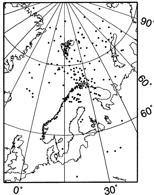
Fig. 6.1.6. As Fig. 6.1.5, now showing the 186 events located by the GBF system applying the new ARCES recipes but not located by the old recipes (see Table 6.1.3).
