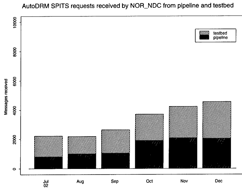
Fig. 4.2.4. The figure shows the monthly number of requests received by NOR_NDC from the IDC for SPITS waveform segments during July - December 2002.
