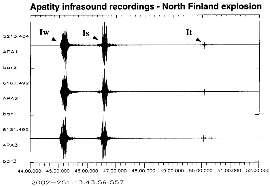
Fig. 6.4.5. Infrasound recordings of an ammunition demolition explosion in northern Finland at 300 km distance. Data are filtered 2-6 Hz. Three distinct infrasonic phases are indicated.
