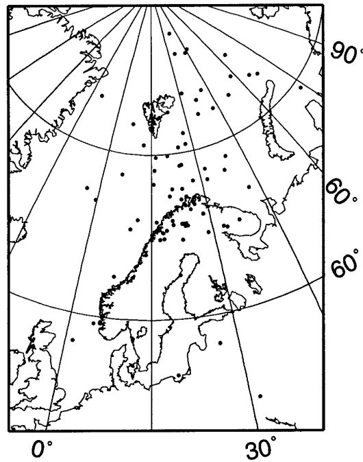
Fig. 6.1.5. Events located by GBF with at least 2 P onsets at 2 different stations and 1P + 1 S onsets as defining observation at one station using the old ARCES processing results; here are only shown the 88 events, which were not in the GBF bulletins using the new ARCES recipes (see Table 6.1.3).
