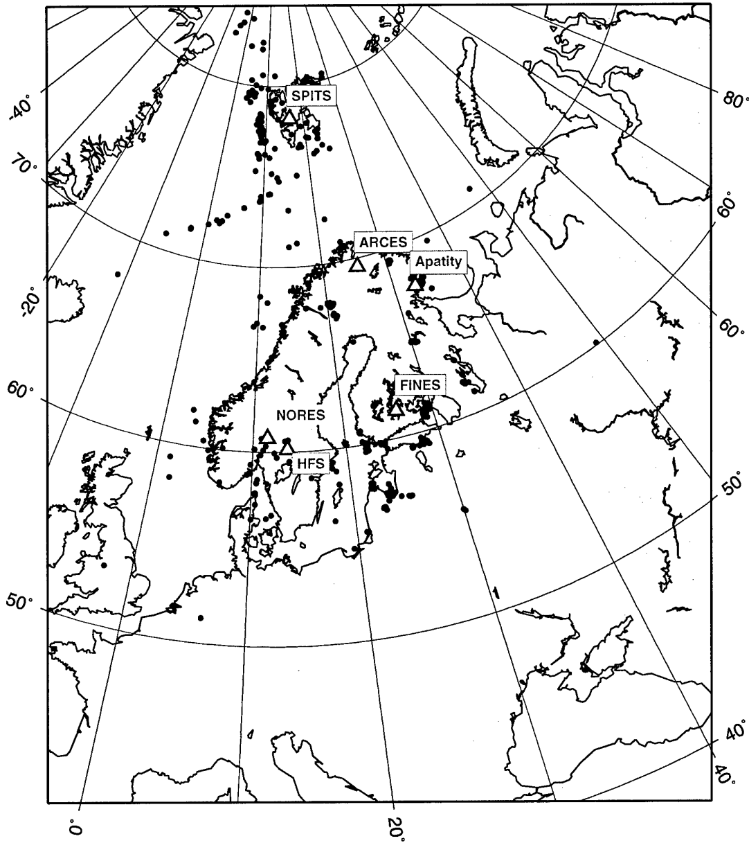
Fig. 4.2.5. The map shows the 456 events in and around Norway contributed by NOR_NDC during July - December 2002 as supplementary (Gamma) events to the IDC, as part of the Nordic supplementary data compiled by the Finnish NDC. The map also shows the seismic stations used in the data analysis to define these events.
