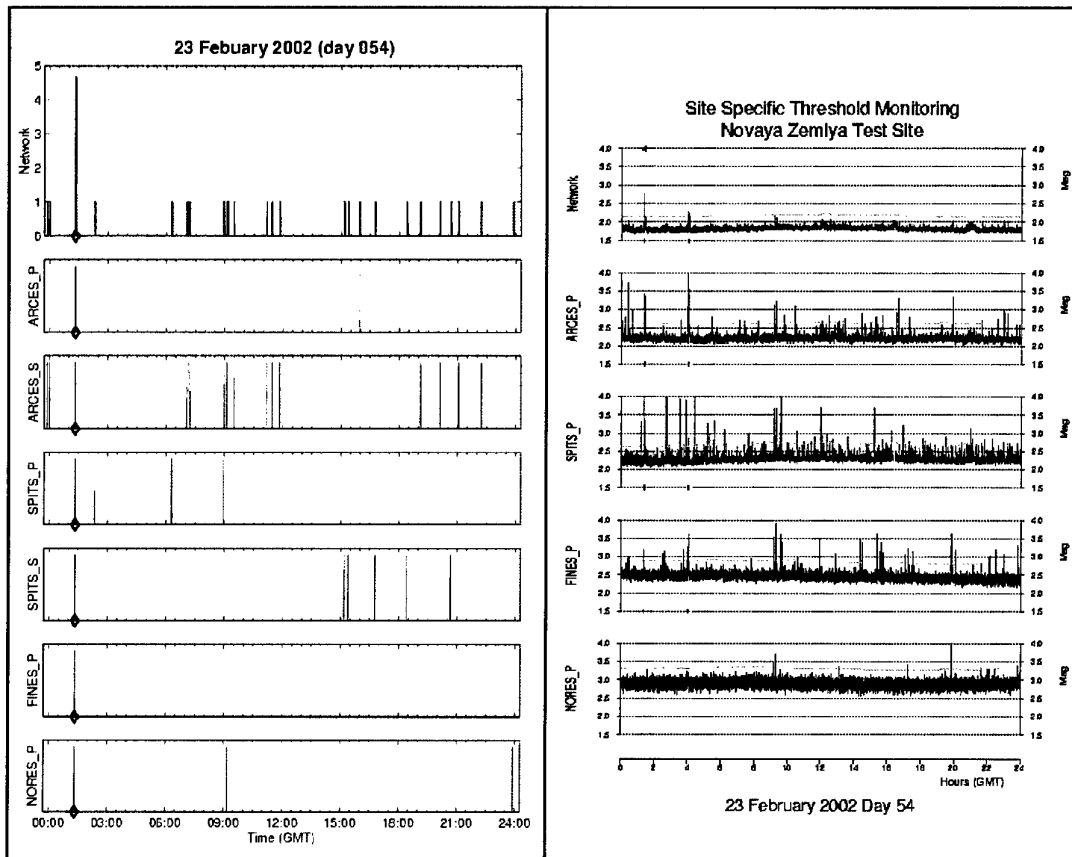
Fig. 6.3.2. SSGBF traces for 23 February 2002 are shown in the left part of the figure. The peaks of the panels for each phase represent detections that fall within the NZ azimuth and slowness ranges given in Table 6.3.1. To align the detections we have subtracted the phase travel-time from NZ to the respective arrays. The network trace on top is calculated by adding “triangular” functions surrounding each detection, using the six phases given in Table 6.3.1. Alerts (red diamonds) are declared when the network trace (the full network) has a value of at least two. The corresponding SSTM traces are shown in the right part of the figure. For detailed information on SSTM we refer to Kværna et. al., 2002b.
