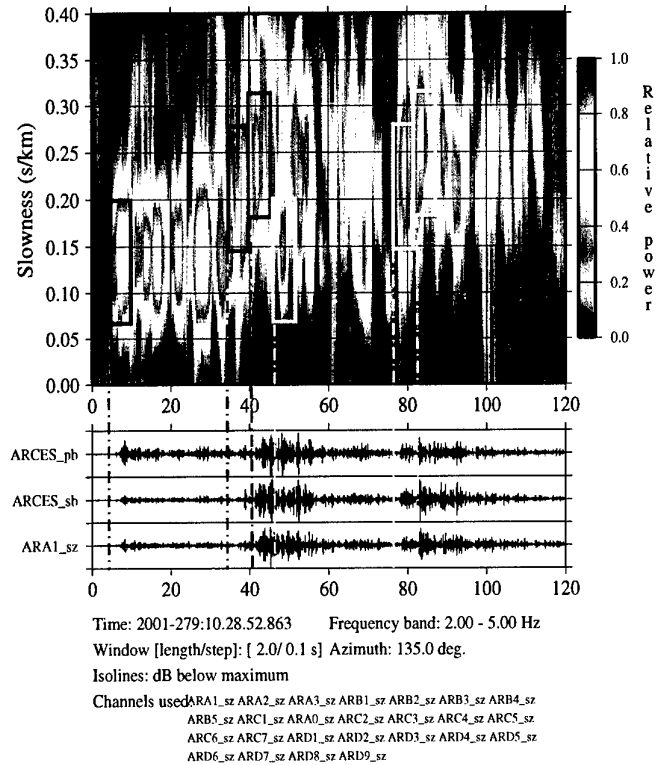
Fig. 6.2.2. Vespagram of the 2001-279 event for the frequency band 2.0-5.0 Hz and constant azimuth 135°. ARCES_pb and ARCES_sb are beams with azimuth 135° and apparent velocity 8.0 kms -1 and 4.0 kms -1 respectively.
