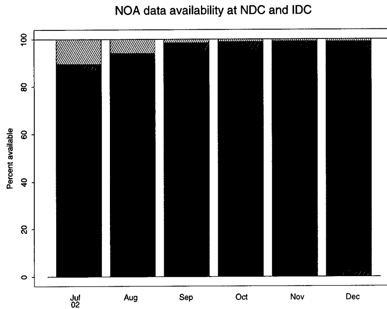
Fig. 4.2.3. The figure shows the monthly availability of NORSAR array data for the period July - December 2002 at NOR_NDC and the IDC. See the text for explanation of differences in definition of the term "data availability" between the two centers. The higher values (hatched bars) represent the NOR_NDC data availability.
