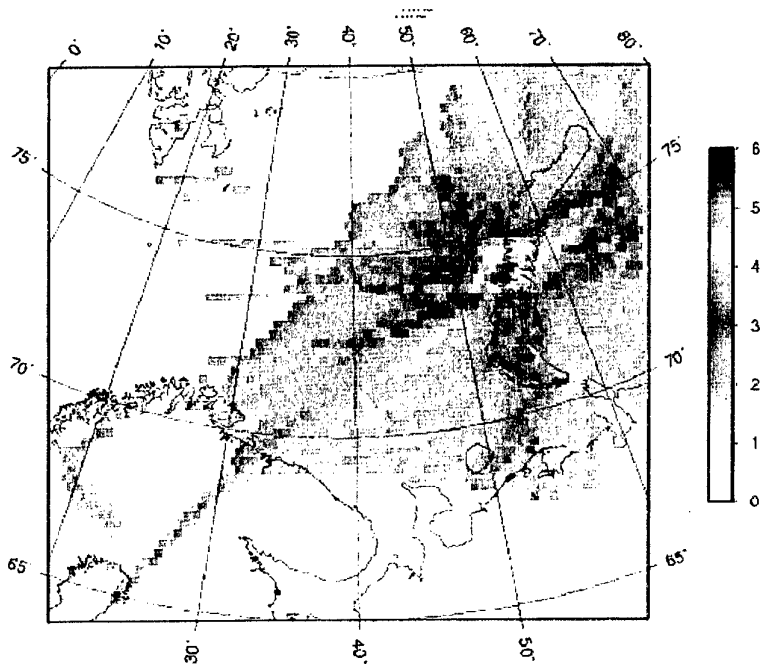
Fig. 6.3.7. Regional GBF results for 23 February 2002, 01:00-02:00 GMT. See Fig. 6.3.3 for comparison with the SSGBF and SSTM results.
