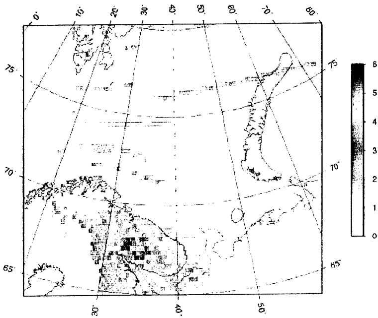
Fig. 6.3.8. Regional GBF results for the one-hour time interval 04:00-05:00 GMT on 23 February 2002. At 04:00:37 there was an 76 ton underground explosion in one of the mines in the Khibiny Massif on Kola.
