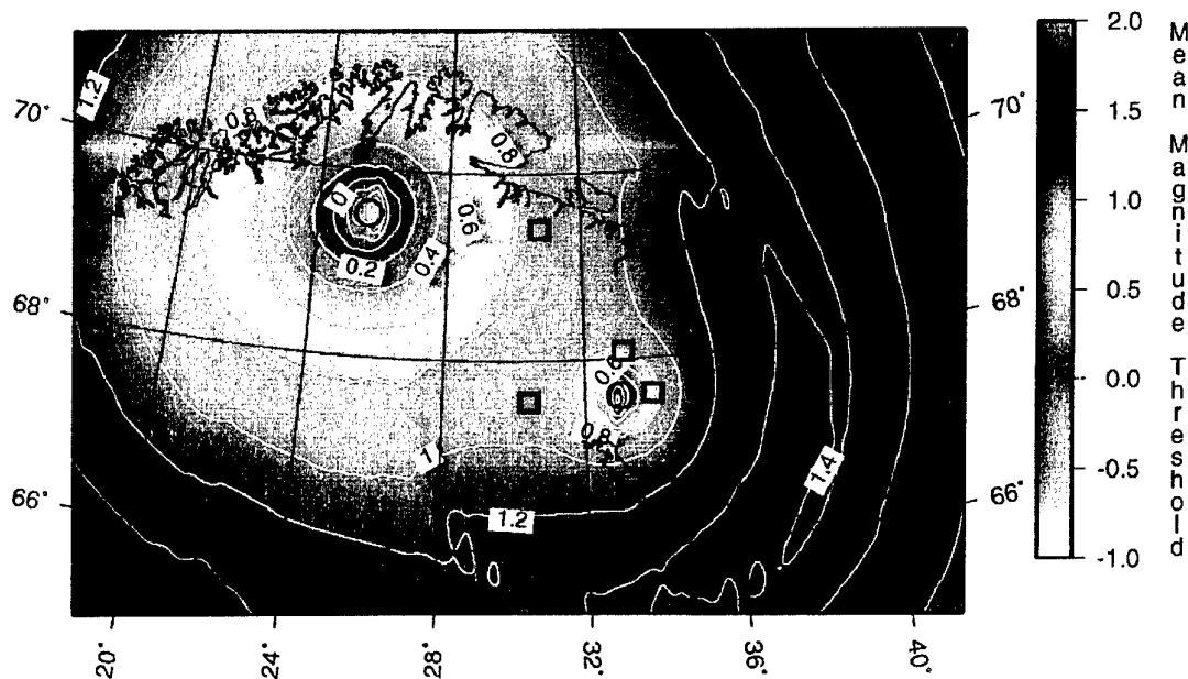
Fig. 6.5.6. Mean network magnitude thresholds for a 2-hour time interval starting 2002-102:10:00.
