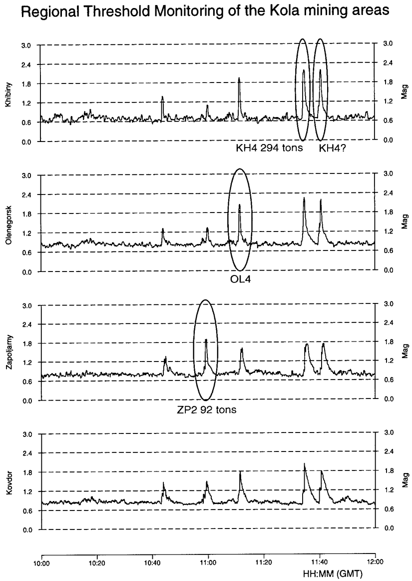
Fig. 6.5.7. Network magnitude thresholds for the grid points closest to the four mining areas shown in Fig. 6.5.1, for the 2-hour time interval starting 2002-102:10.00. Five significant threshold peaks are seen during this time interval, of which three are mining explosions reported by the KRSC. The last peak at 11:40 is believed to be an additional explosion at the Central Khibiny mine KH4. The first peak at 10:44 is caused by an event located approximately 70 km south-west of the Apatity array.
