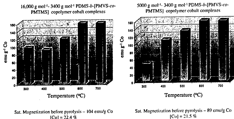
Figure 10. The saturation magnetizations of the co balt after heat treatment at 600 or 700 °C approach that of bulk cobalt.
