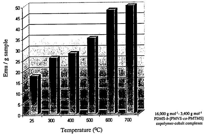
Figure 9. The saturation magnetization of the cobalt -copolysiloxane complexes increases with annealing temperature.
