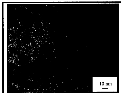
Figure 3. Cobalt nanoparticles coated with a 16,000\text{ g mol}^{-1} PDMS- 3900\text{ g mol}^{-1} PMVS-co-PMTMS copolymer. The PMTMS block anchors to the cobalt surface and the PDMS tail block provides dispersion stability in the toluene reaction solvent.
