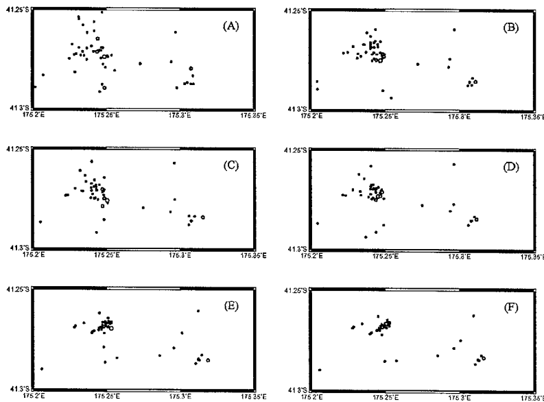
Figure 2. Locations of 53 earthquakes near lake Wairarapa, NZ. (A) Before relocation; (B) relocated with catalog differential travel times; (C) relocated with CC differential travel times chosen with the threshold criterion; (D) relocated with CC differential travel times verified with the bispectrum method; (E) relocated with both catalog and threshold-chosen CC differential travel times; (F) relocated with both catalog and bispectrum-verified CC differential travel times.
