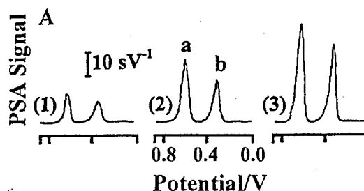
Fig. 4 (A) Chronopotentiometric signals for mixtures containing increasing levels of the E908X-WT and 1675delA-WT targets: (1) 100, (2) 300 and (3) 500 \text{ ng ml}^{-1} . (B) The resulting calibration plots, as well as the response for a sample containing 10 \text{ ng ml}^{-1} of the E908X-WT and 1675delA-WT targets. Other conditions, as in Fig. 2.
