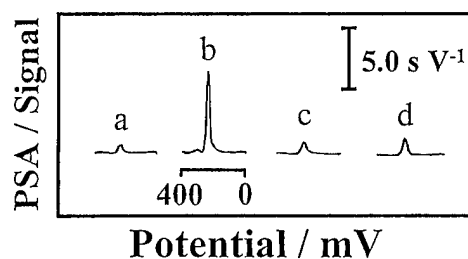
Fig. 2. Chronopotentiometric stripping hybridization response to: (a) 0 \mu g/ml of E908X-WT complementary target; (b) 1 \mu g/ml of E908X-WT complementary target; (c) 20 \mu g/ml of noncomplementary target; (d) 100 \mu g/ml of noncomplementary target. Conditions: hybridization time, 30 min in a 0.05 M phosphate-buffer solution; stripping current, +3.0 \mu A; deposition at -0.5 V for 1 min using a 0.1 M HNO 3 /0.1 M KNO 3 medium; SPEs pretreated at +1.2 V for 3 min.
