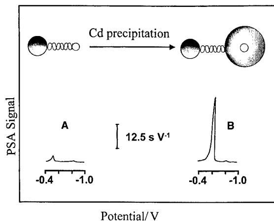
Fig. 4. Stripping potentiograms for 0.4 \text{ mg l}^{-1} target, without (A) and with (B) catalytic enhancement with 30 \mu\text{l} of 10 \text{ mM Cd(NO}_3)_2 and 30 \mu\text{l} of 0.05 \text{ M} hydroquinone. Other conditions, as Fig. 2.
