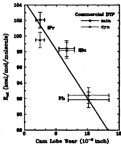
Figure 2: Correlation of SAM adsorption energy with wear in engine wear tests for commercial DTP molecules. The error in the adsorption energy is 1 kcal/mol/molecule. The straight line is the least-square fit to the results of both minimization and dynamics simulation.
