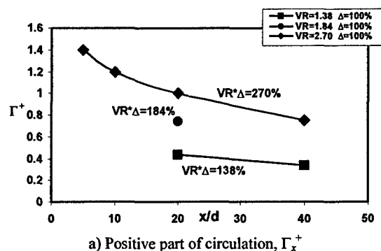
Figure 14: Effect of blowing rate on longitudinal circulation.
