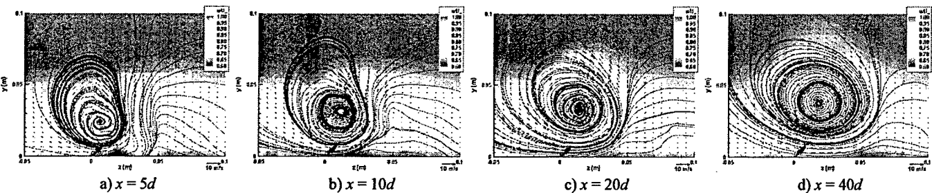
Figure 25: Longitudinal velocity contours & secondary streamlines. f=15\text{Hz} ( F_x^+/\ell = 0.5/\text{m} ); VR=2.76 ; \Delta=50\% .
