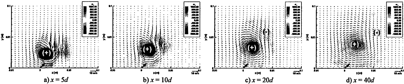
Figure 24: Longitudinal vorticity contours & secondary flow vectors. f=15\text{Hz} ( F_x^+/\ell = 0.5/\text{m} ); VR=2.76 ; \Delta=50\% .
