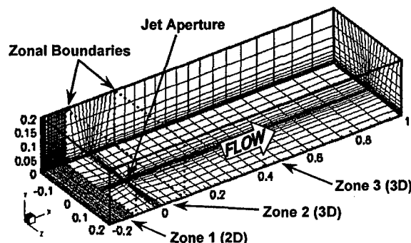
Figure 4: Grid features for numerical simulations.
