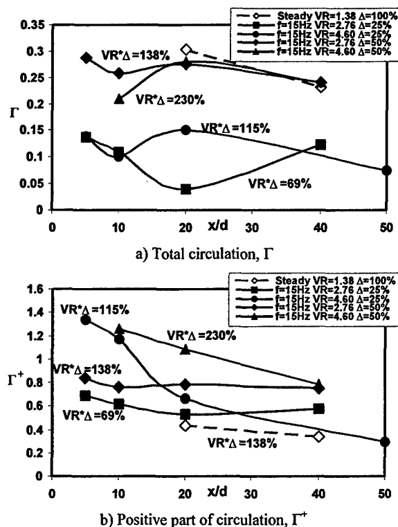
Figure 21: Longitudinal trend in total longitudinal circulation. f=15\text{Hz} ( F_x^+/\ell = 0.5/\text{m} )
