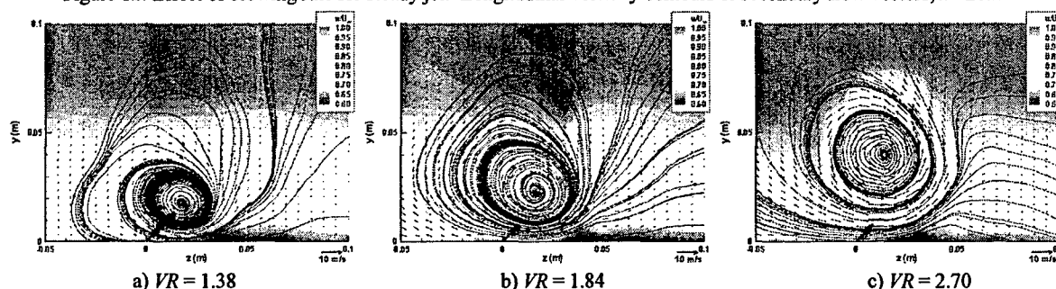
Figure 13: Effect of blowing rate for steady jet. Longitudinal velocity contours & secondary streamlines, x=20d .
