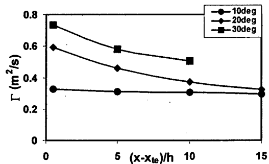
Figure 10: Trend in total longitudinal circulation for a 30\text{mm} \times 70\text{mm} delta-vane vortex generator.
