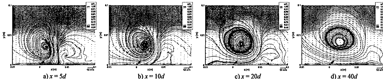
Figure 20: Longitudinal velocity contours, secondary streamlines. f=15\text{Hz} ( F_x^+/\ell = 0.5/\text{m} ); VR=2.76 ; \Delta=25\% .
