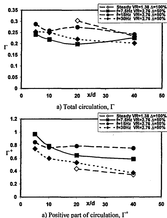
Figure 28: Effect of frequency on longitudinal circulation.
