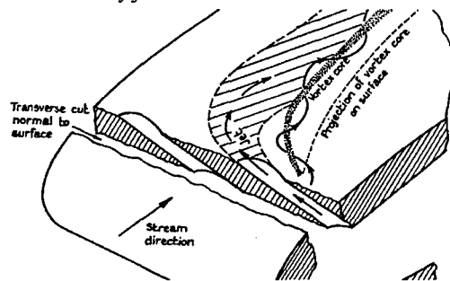
Figure 16: Sketch of steady VGJ flowfield (from reference 3).
