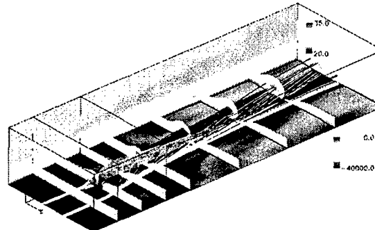
Figure 16: Sketch of steady VGJ flowfield (from reference 3).
