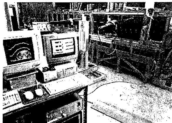
Figure 3: DERA Bedford Boundary Layer Wind Tunnel
