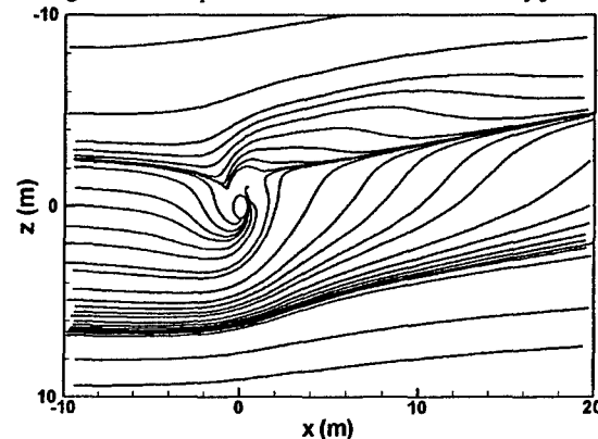
Figure 18: Computed surface limited streamlines (surface flow). VR=2.7 steady jet.
