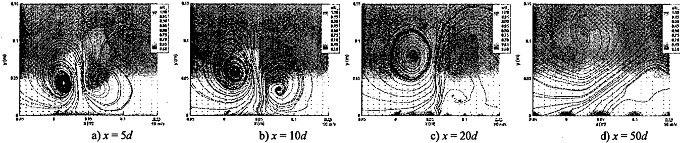
Figure 23: Longitudinal velocity contours & secondary streamlines. f=15\text{Hz} ( F_x^+/\ell = 0.5/\text{m} ); VR=4.60 ; \Delta=25\% .
