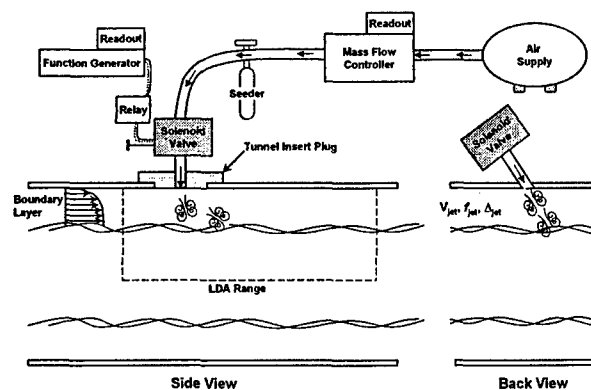
Figure 1: Schematic of experimental hardware setup.
