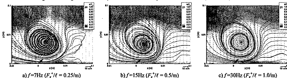
Figure 27: Longitudinal velocity contours, secondary streamlines. x=20d ; VR=2.76 ; \Delta=50\% .
