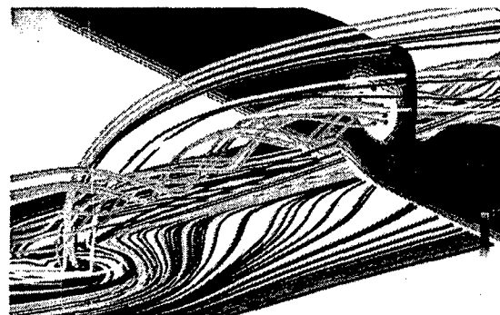
Figure 17: Computed flowfield for VR=2.7 steady jet.
