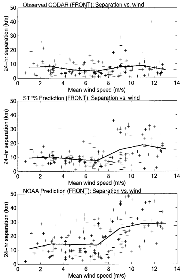
Figure 16: Block Island Region 24-hour Separation versus Wind.
