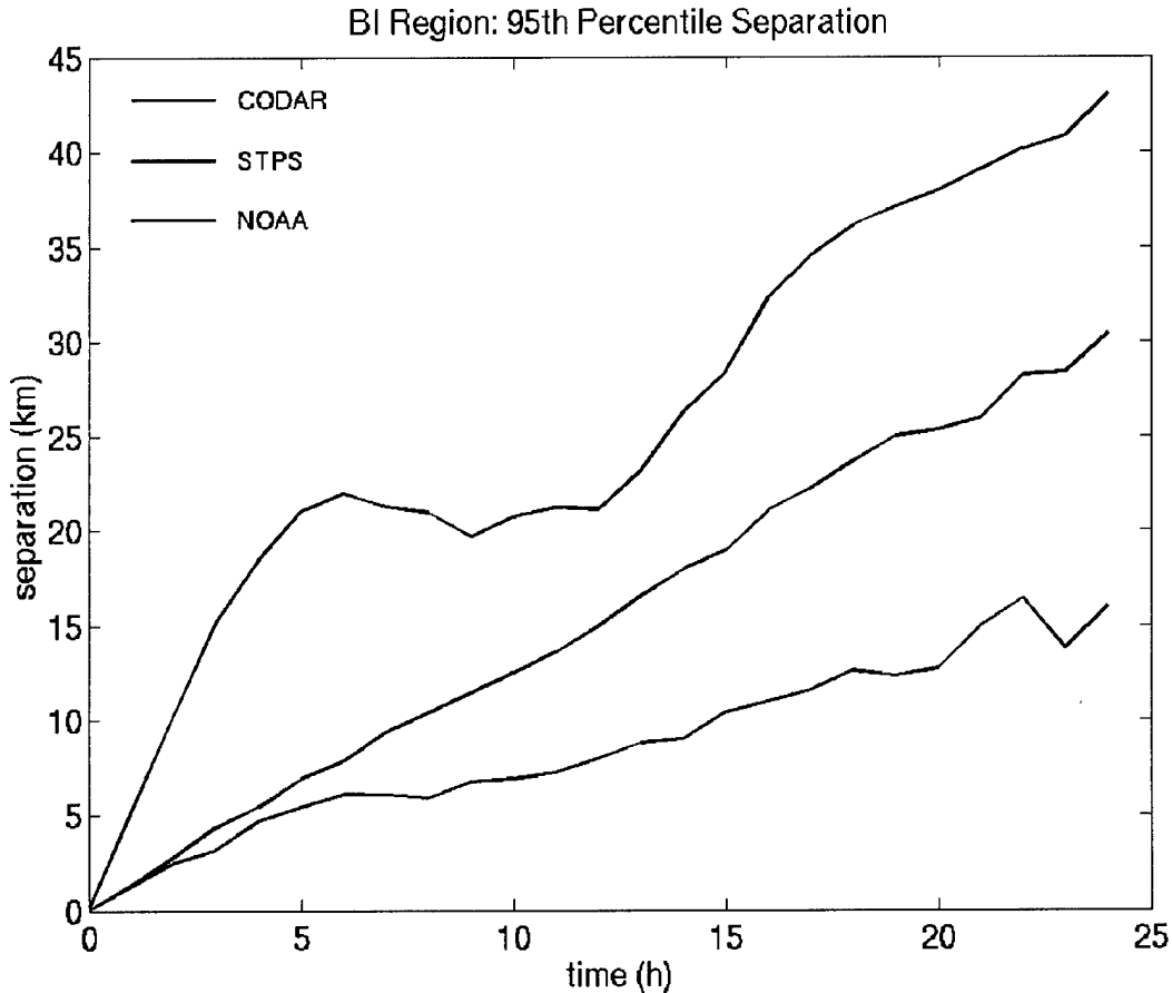
Figure 13: Block Island Region 95 th Percentile Separation.
