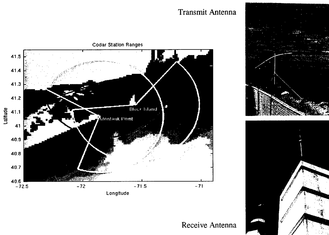
Figure 2: Block Island Sound CODAR Installation.
