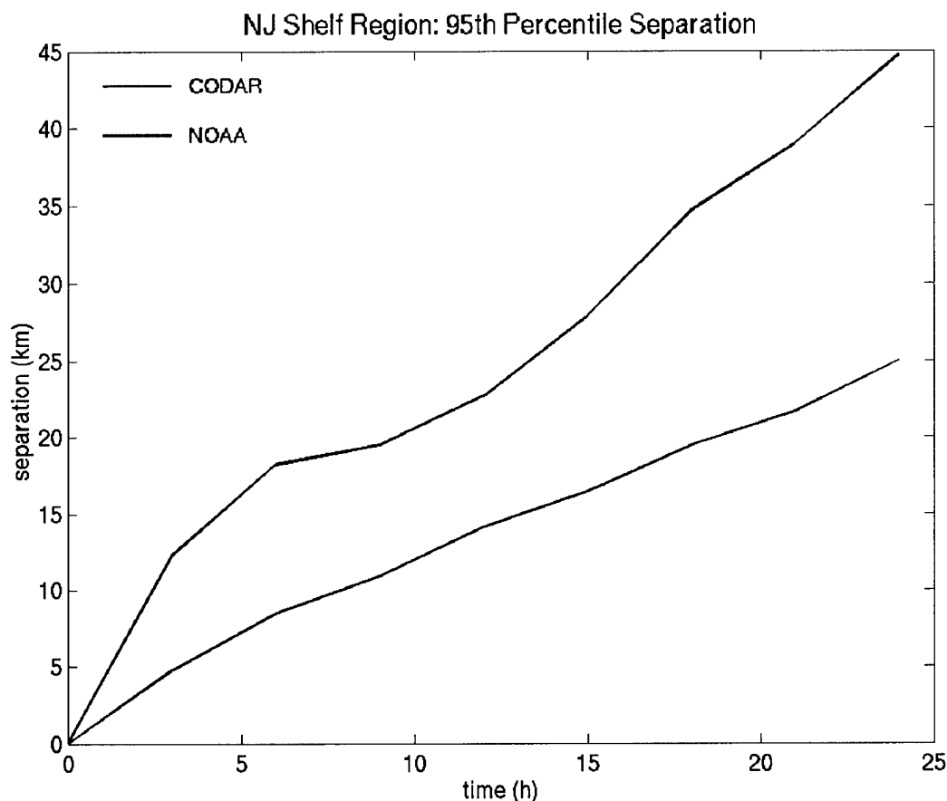
Figure 15: New Jersey Shelf Region 95 th Percentile Separation.
