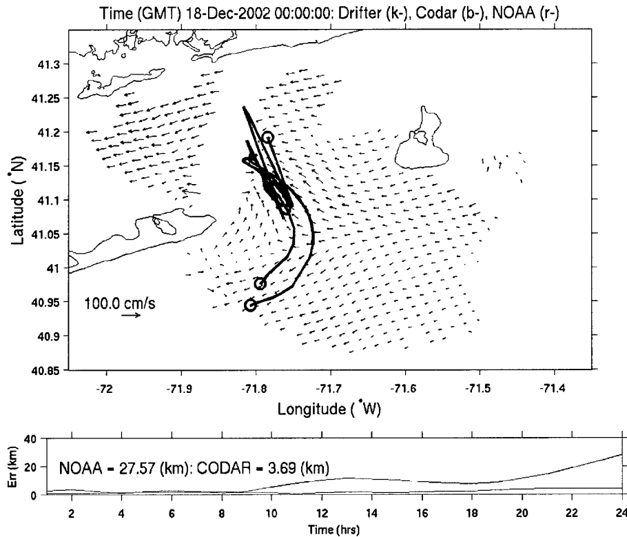
Figure 11: Sample Trajectory Predictions.
