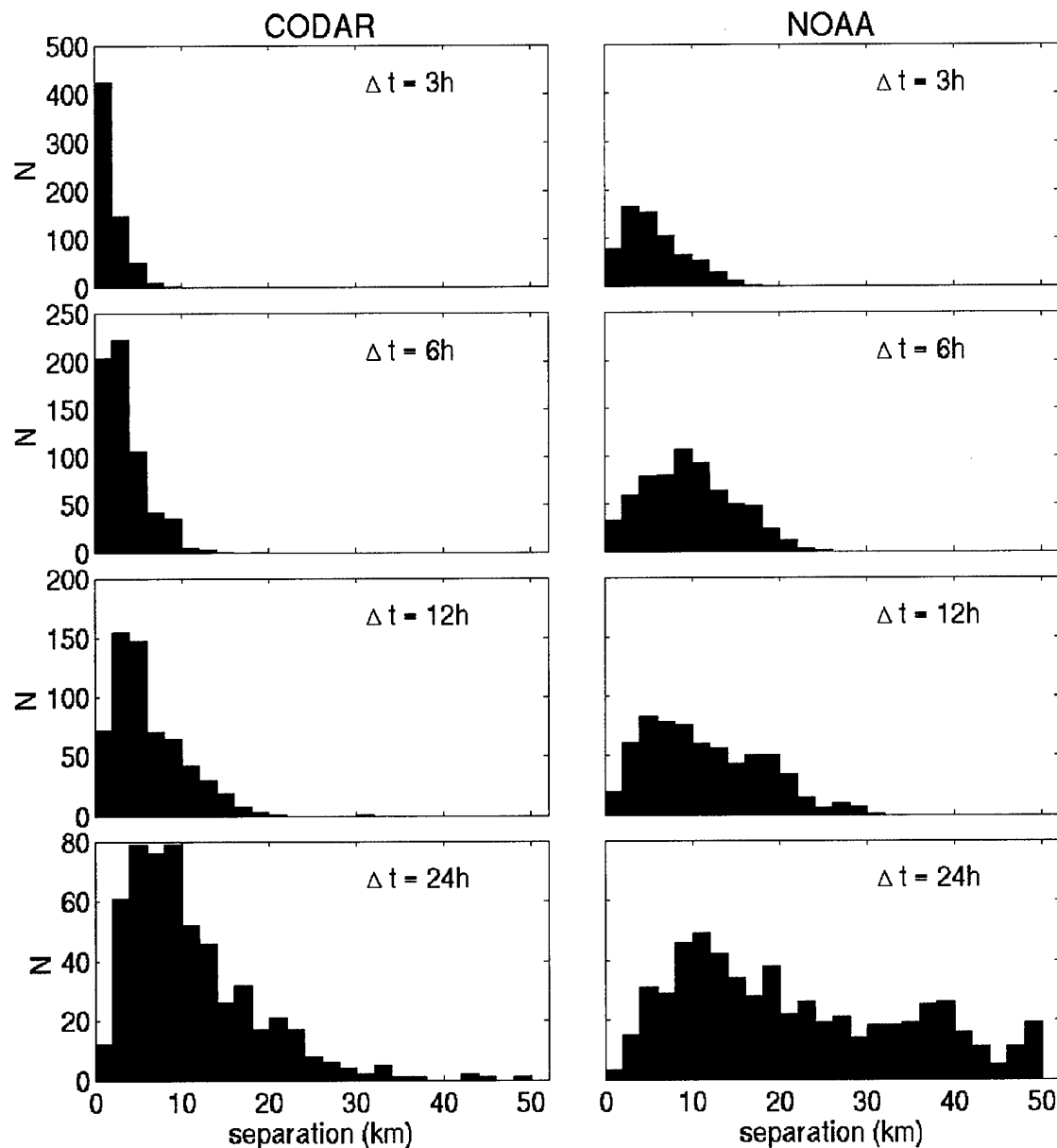
Figure 14: New Jersey Shelf Region Trajectory Error Histograms.
