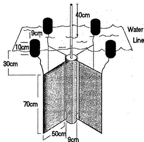
Figure 9: Self-Locating Datum Marker Buoy.
