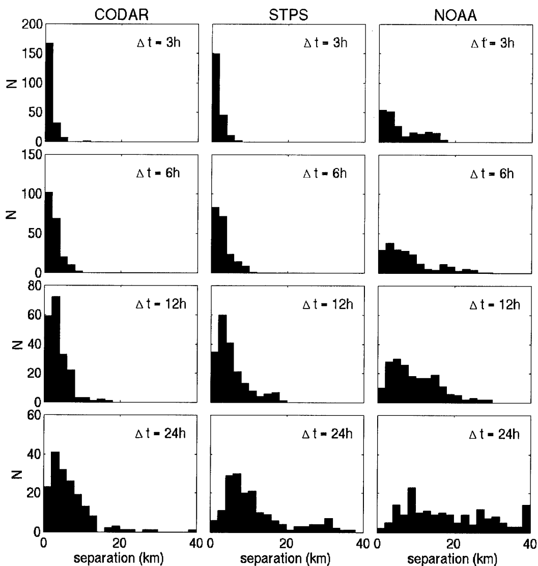
Figure 12: Block Island Region Trajectory Error Histograms.
