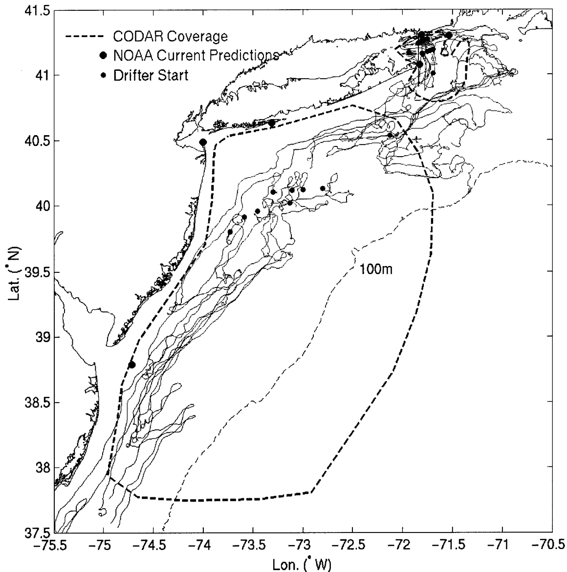
Figure 10: December 2002 and March 2003 SLDMB Deployments.
