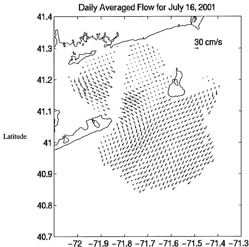
Figure 1: Complex Coastal Current Fields.
