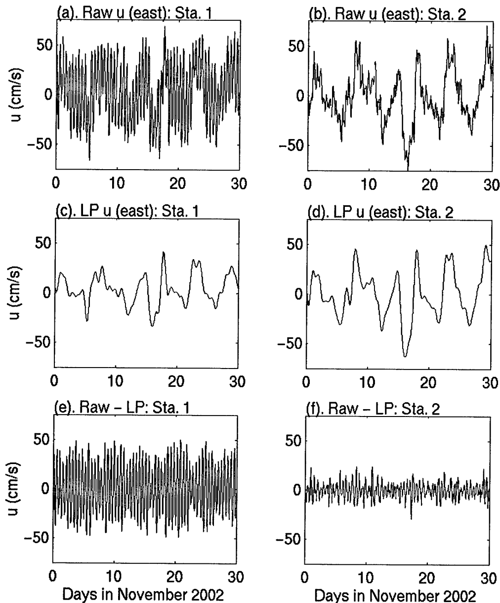
Figure 5: CODAR-derived Surface Current Time Series During November 2002.
