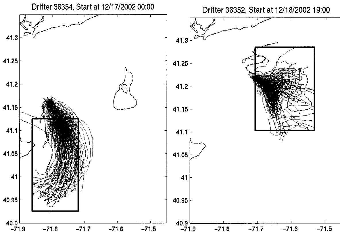
Figure 17: Simulations of SLDMB Trajectories.
