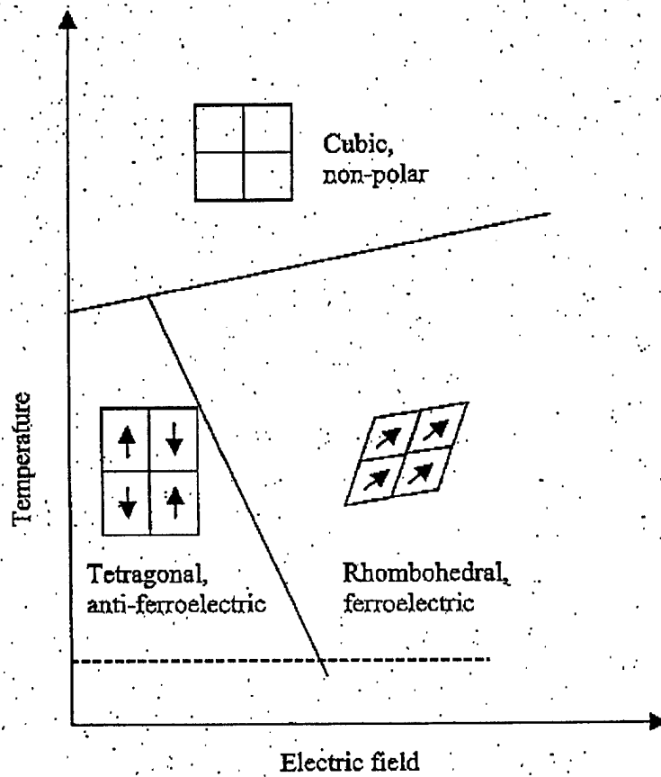
Figure 8: The temperature vs. electric field phase diagram for Lead Zirconate (PbZrO 3 )
