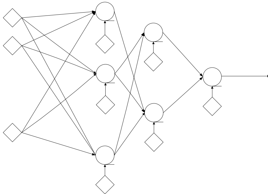
Figure 89 Architecture of a Multilayer Perceptron with Two Hidden Layers and a Single Output Neuron (After [9]).
