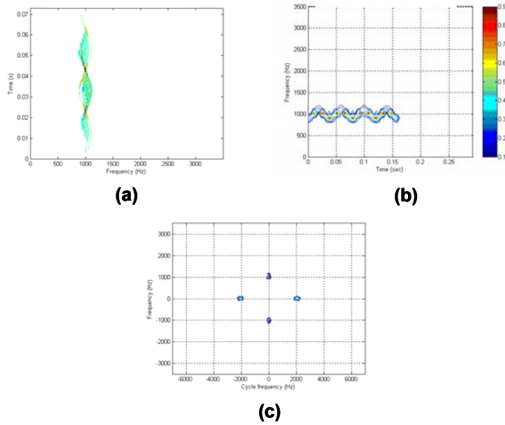
Figure 29 Illustration of the FMCW Signal when Processed Using the Three Different Detection Methods.
