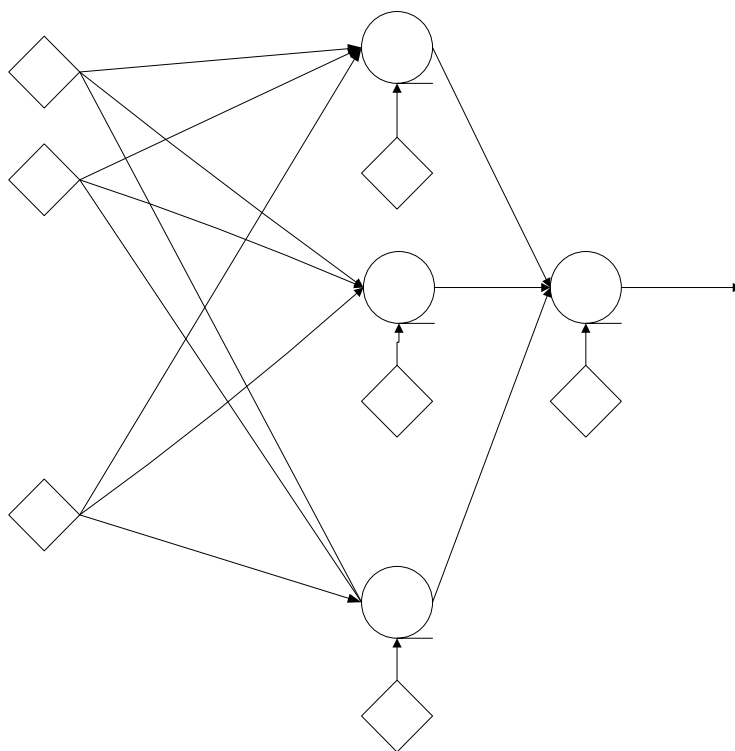
Figure 86 A Two-Layer Perceptron (After [9].).
