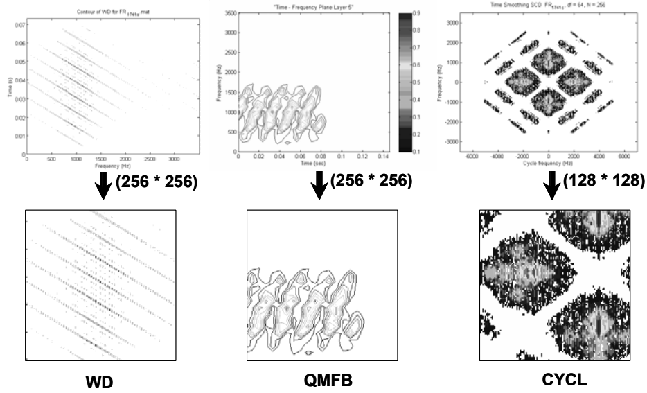
Figure 47 Adaptive Filtering of the FR_1_7_4_1_s Signal.
