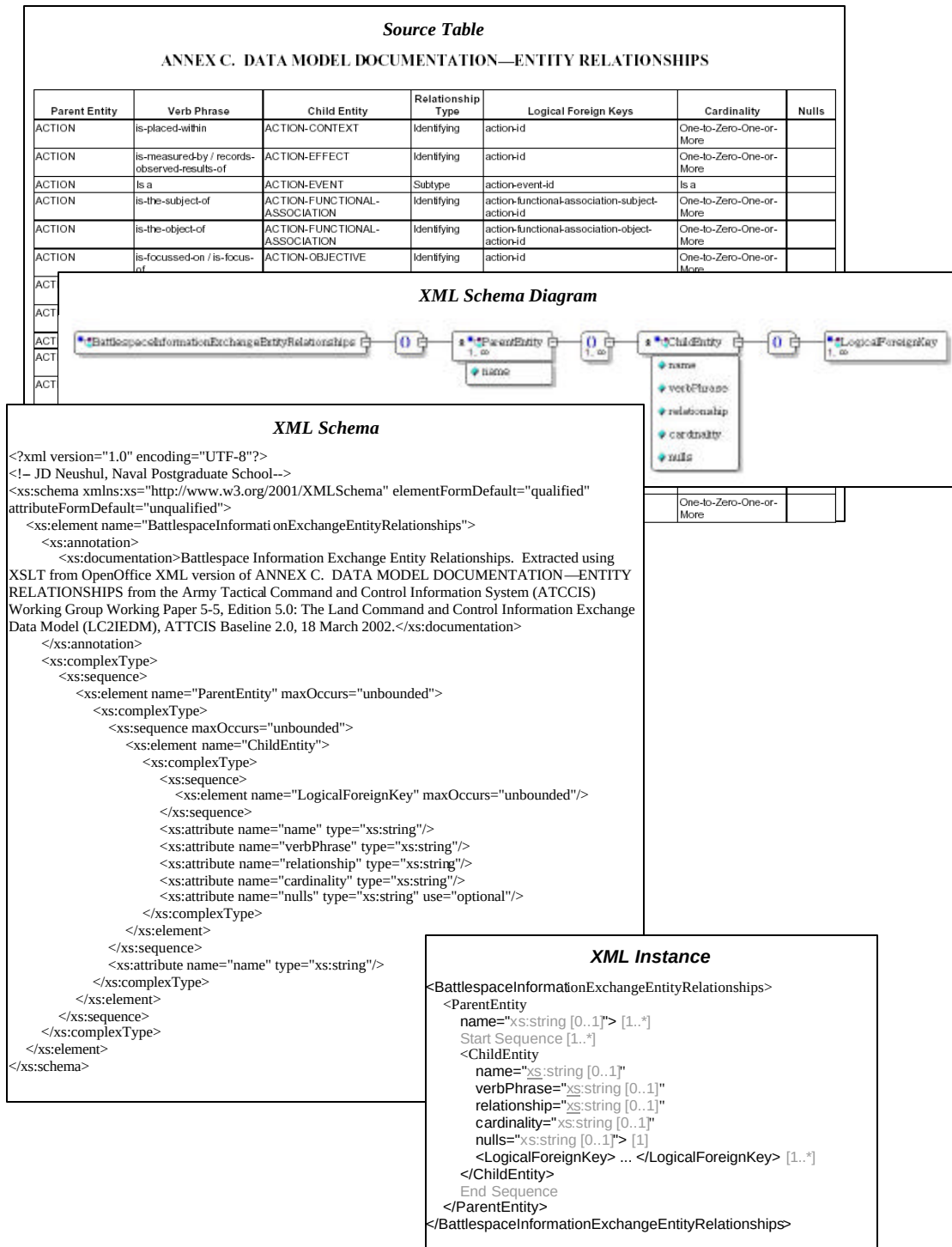
Figure 30. XML Schema Diagram Representation, XML Schema and XML Instance of Entity Relationships Table of the C2IEDM Annexes.
