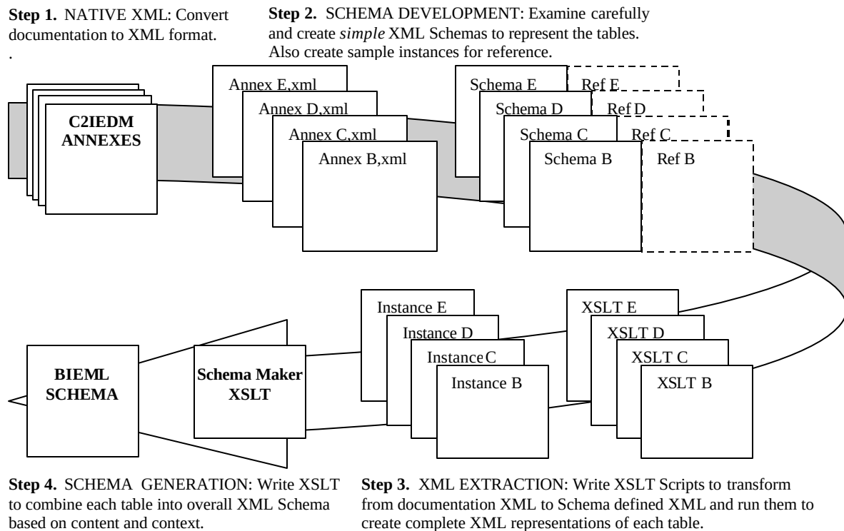
Figure 28. Creating an XML Schema From Source Documentation
