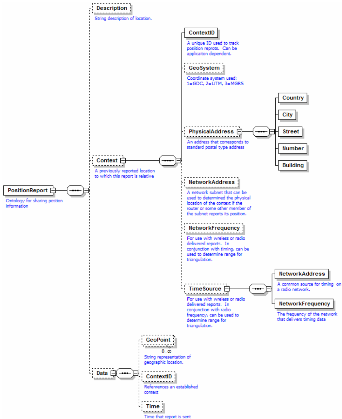
Figure 19. Position Reporting Language XML Schema Architecture
