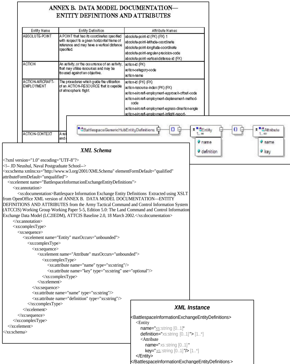
Figure 29. XML Schema Diagram Representation, XML Schema and XML Instance of Entity Definitions and Attributes Table of the C2IEDM Annexes.
