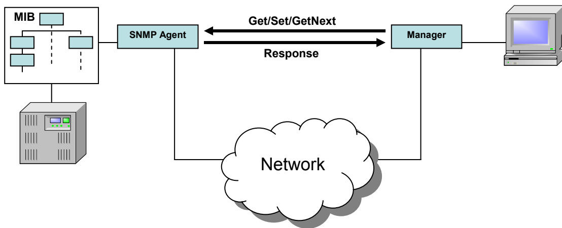
Figure 28. SNMP Components
