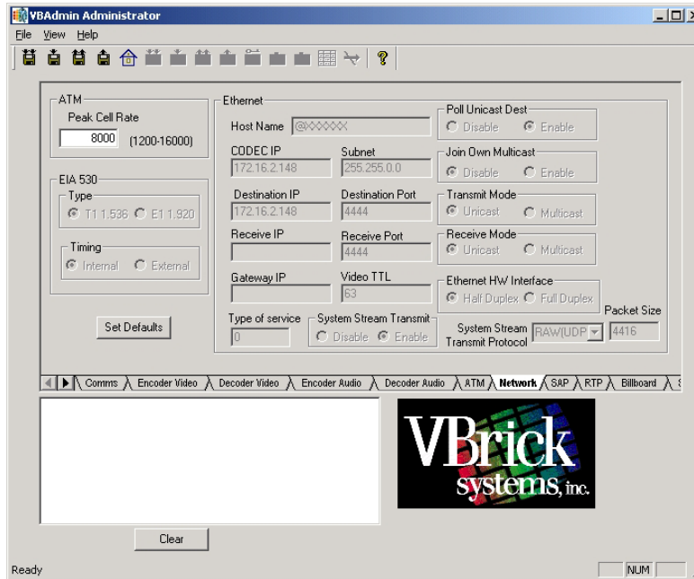
Figure 16. VAdmin Administrator Utility: Network
