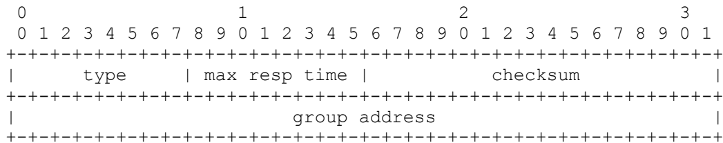
Figure 11. IGMPv2 Message Format [15]
