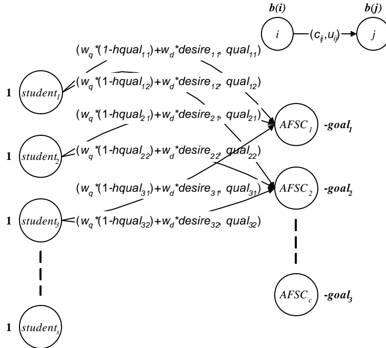
Figure 1. Directed network with students and specialty codes
