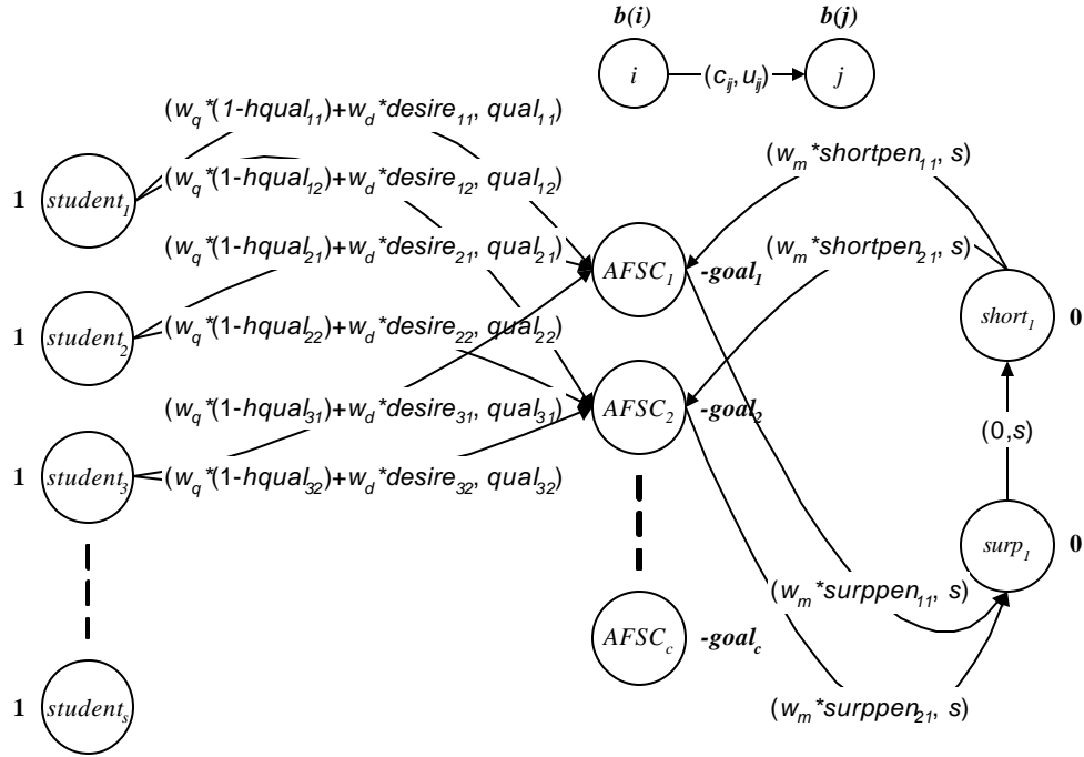
Figure 2. Network with shortage and surplus nodes
