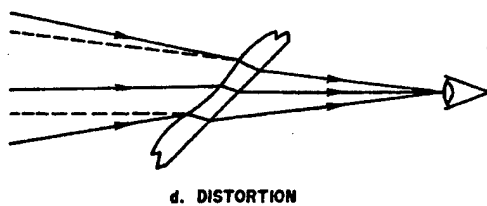
Figure 1. Optical effects related to aircraft windshield design.
