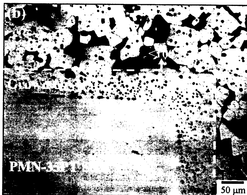
Figure 6. Comparison of \{100\} single crystal growth in PMN-35PT with (a.) 5 vol.% PbO and (b.) 5 vol.% P_2A -PbO eutectic additions.
