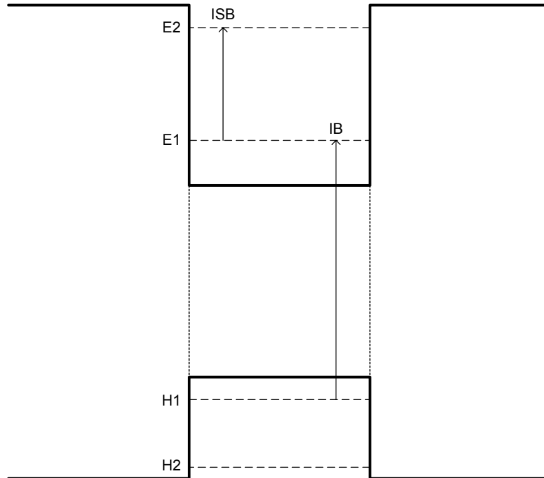
Figure 5. Drawing of interband (IB) and intersubband (ISB) transitions in a square quantum well.
