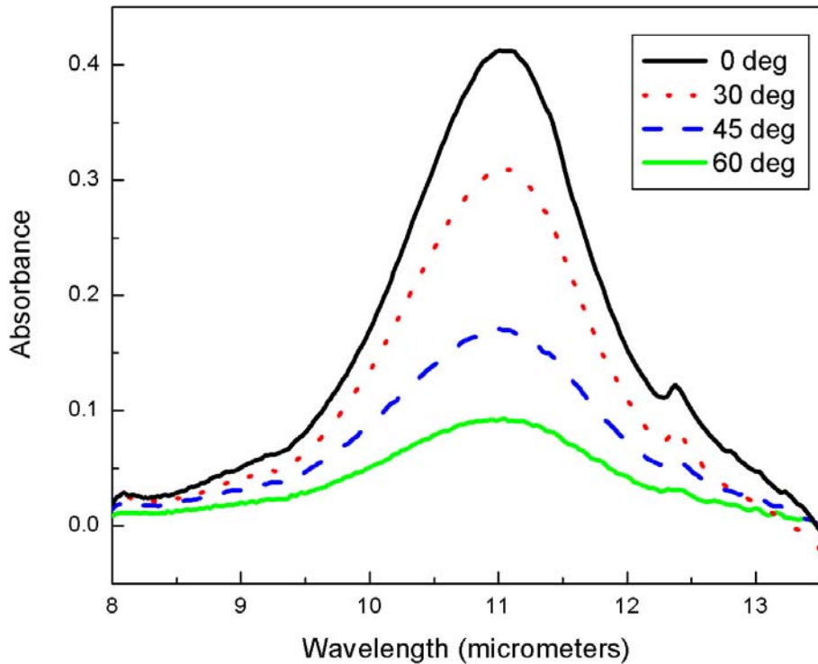
Figure 12. Polarization dependence of absorbance of 25 InGaAs quantum step wells. Peak absorbance is 0.41 at 900\text{ cm}^{-1} ( 11.1\ \mu\text{m} wavelength).
