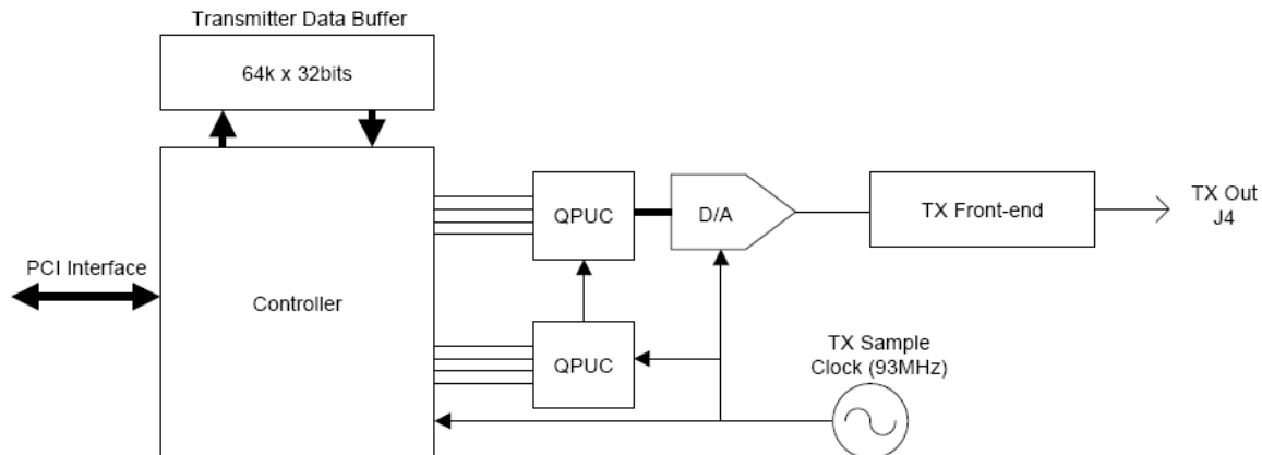
Figure 3-3. WaveRunner 253 Plus Transmitter datapath (From Ref. 7).
