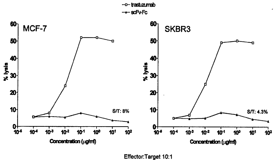
Fig. 8. scFv-Fc does not enhance ADCC. ^{51} Cr-labeled MCF-7 or SKBR3 cells were mixed with human NK cells at a ratio of 1:10 and incubated with various concentrations of scFv-Fc ( \blacktriangle ) or trastuzumab ( \square ) for 4 h. Cells were harvested, and cpm of ^{51} Cr released by lysis was counted using a \gamma -counter. Percentage of lysis of cells was calculated using Sp-S/T-S, where Sp is the specific lysis caused by antibody, S is the spontaneous lysis of cells in the absence of antibody, and T is the total lysis of cells by Triton X-100. Spontaneous lysis of cells was <8%. The results are plotted as percentage of lysis against the concentration of antibody. The data shown is representative of three experiments with similar results.
