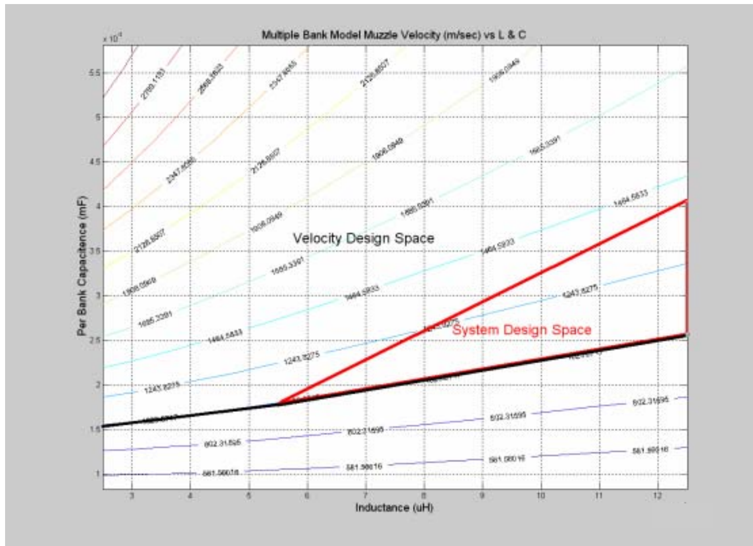
Figure 19. Multiple-bank muzzle velocity contour plots and system design space.
