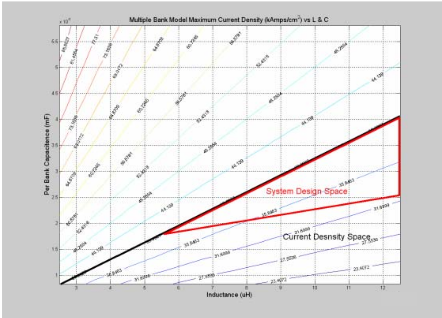
Figure 20. Multiple-bank maximum current density plots and system design space.
