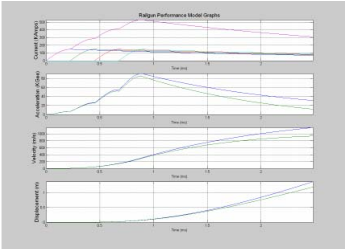
Figure 39. MATLAB performance model graphs for the PSpice current pulse.
