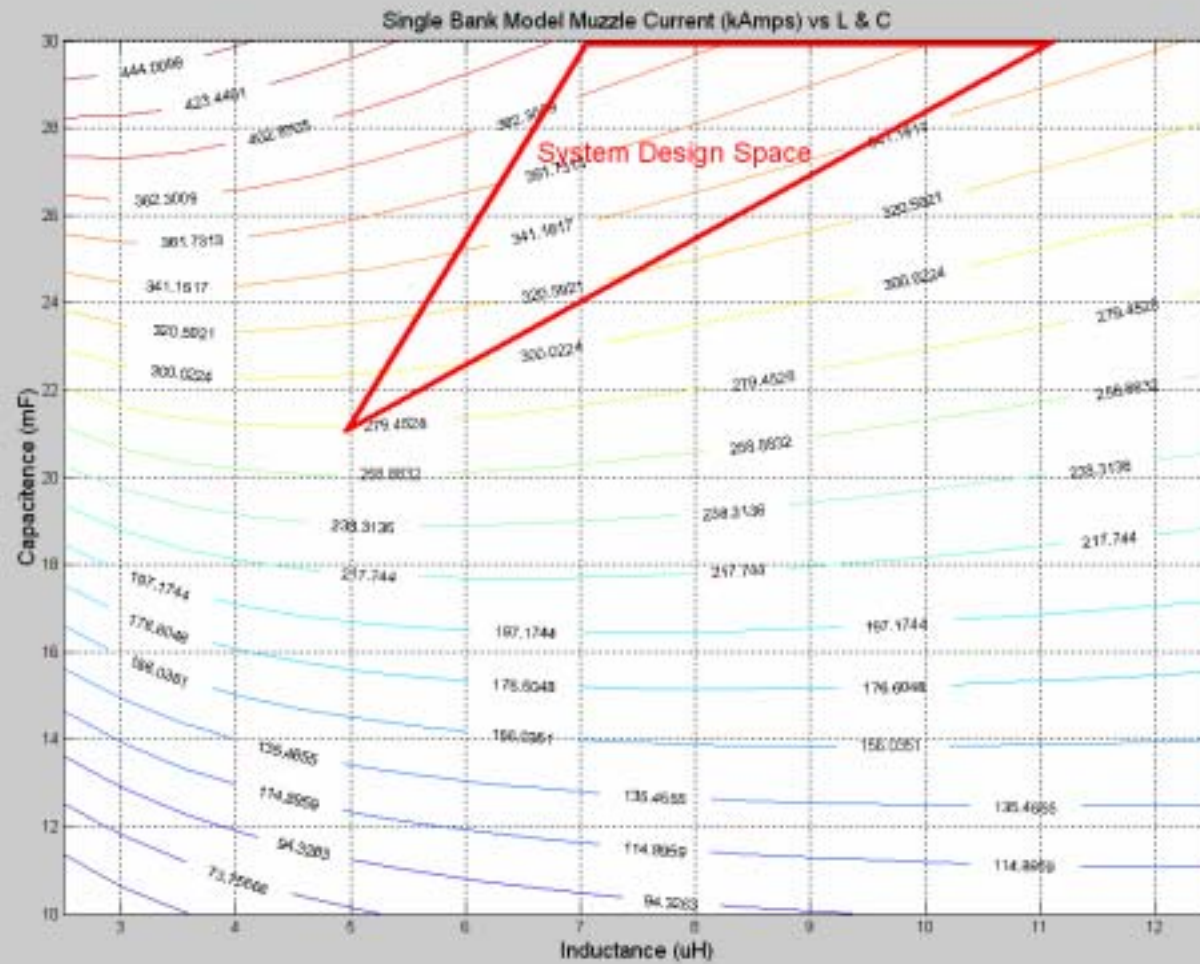
Figure 45. Single-bank muzzle current contour plot.
