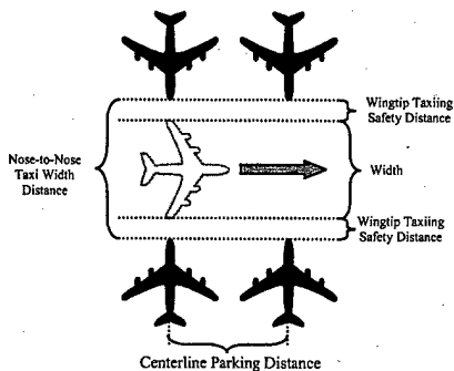
Figure 3. Nose-To-Nose Taxiway
