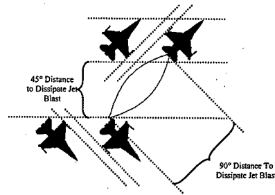
Figure 4. Tail-To-Tail Taxiway
