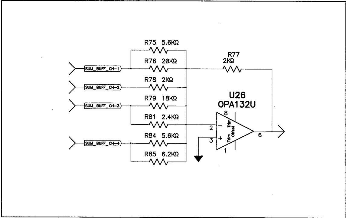
Figure 2-7: Preamplifier Summing Stage
