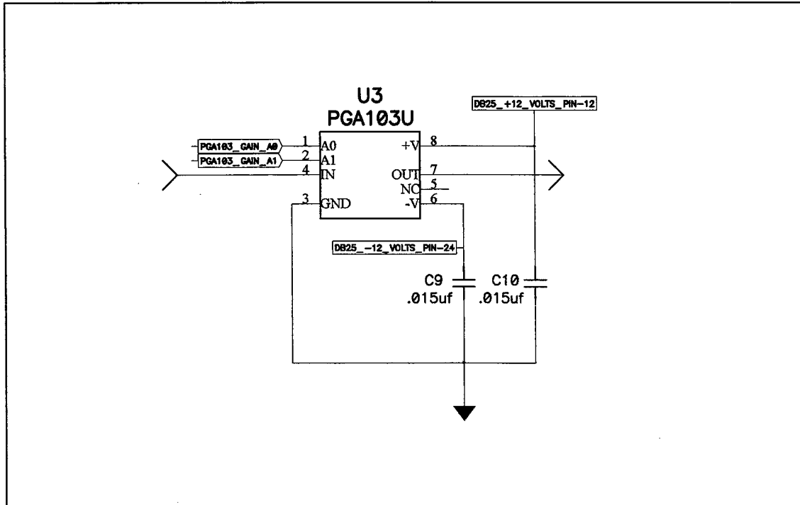
Figure 2-5: Preamp Second Stage
