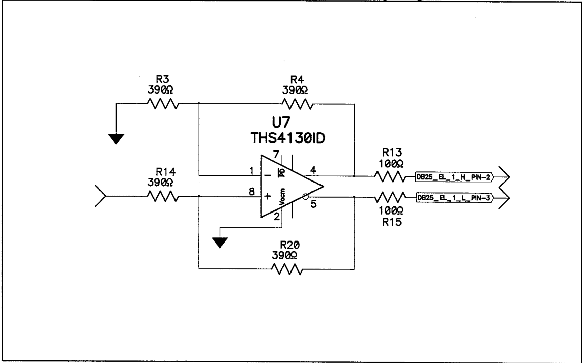
Figure 2-8: Preamplifier Output Stage
