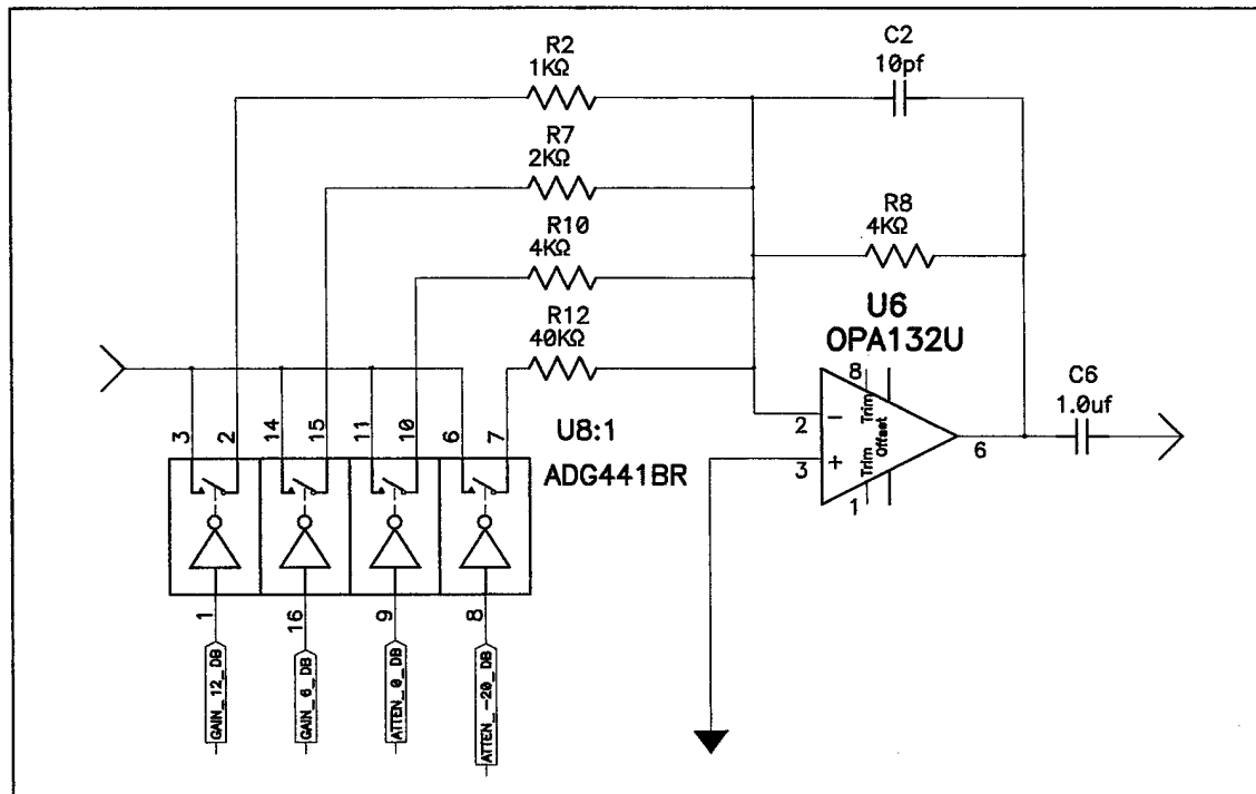
Figure 2-6: Preamp Third Stage
