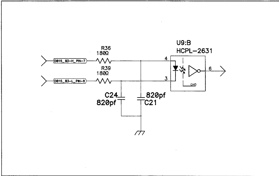
Figure 2-9: Remote Programmable Gain Circuit
