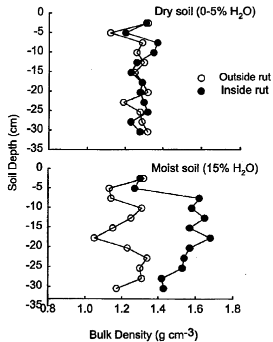
Figure 11. Soil compaction measurements on dry and moist soils at Yakima Training Center. Higher bulk density values indicate greater compaction.
