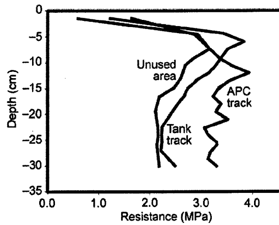
Figure 10. Soil compaction measurements at Fort Carson. Higher resistance values indicate greater compaction.
