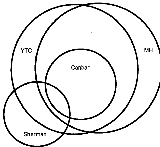
Figure 6. Venn diagram representation of genetic variation in Sandberg bluegrass populations collected near Mountain Home (MH), Idaho, and Yakima Training Center (YTC), and the cultivars Canbar canby bluegrass and Sherman big bluegrass.
