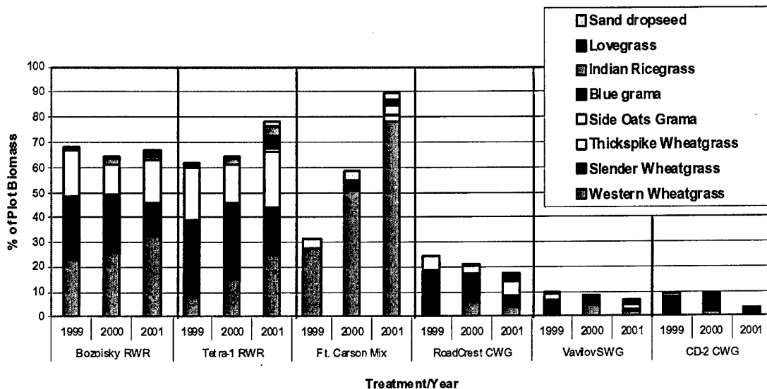
Figure 17. Percent native grasses in Turkey Creek plots planted with the standard Fort Carson mix or with a core native mix plus an introduced grass (as named on the treatment axis). RWR = Russian wildrye, CWG = crested wheatgrass, SWG = Siberian wheatgrass.
