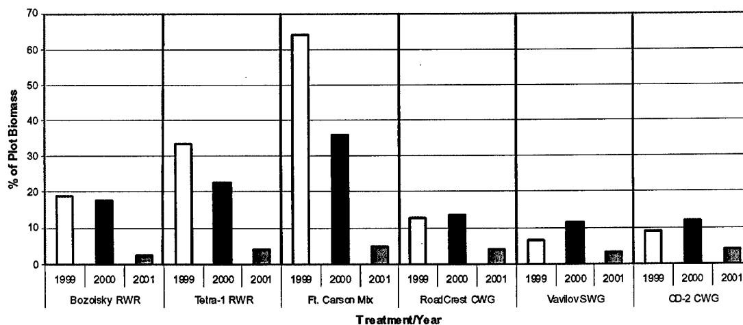
Figure 16. Percent annual and biennial weeds in Turkey Creek plots planted with the standard Fort Carson mix or with a core native mix plus an introduced grass (as named on the treatment axis). RWR = Russian wildrye, CWG = crested wheatgrass, SWG = Siberian wheatgrass.
