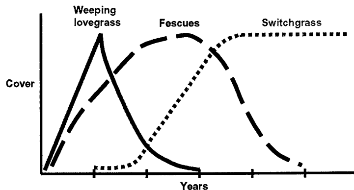
Figure 15. Ecological bridge concept. Weeping lovegrass acts as a nurse crop on sandy soils at Fort Drum, allowing fescues and eventually the desired native grass, switchgrass, to become established.
