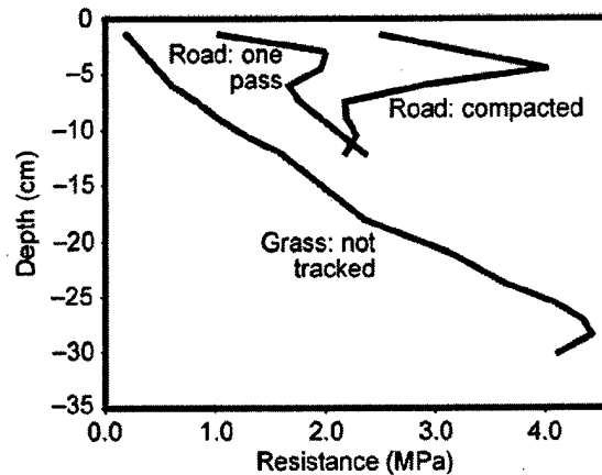
Figure 8. Soil compaction measurements at Fort Drum. Higher resistance values indicate greater compaction.
