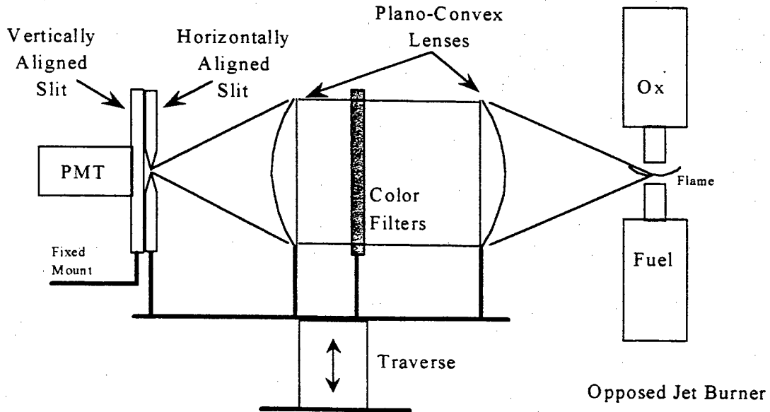
Configuration of Collection Optics
