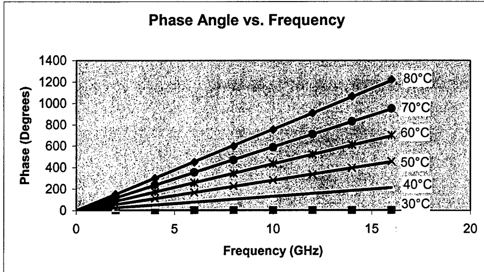
Figure 15: Measurement results showing the phase angle as a function of the frequency. Steeper lines represent larger amounts of time delay as the temperature increases.
