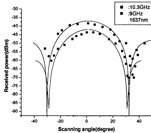
Figure 4(a) Measured radiation patterns at 9GHz and 10.3GHz for \lambda = 1537\text{nm} .
