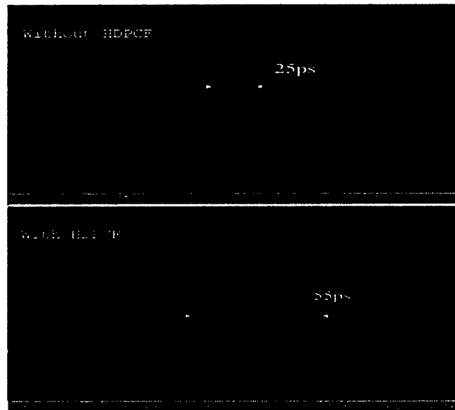
Figure 4 Chromatic dispersion of 3m of the fabricated HDPCF is measured by pulse broadening effect. The calculated result is 1219 ps/nm·km at 1550 nm.
