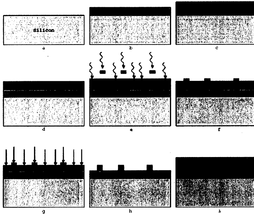
Figure 5: Schematic of the buried channel waveguide processing steps.
