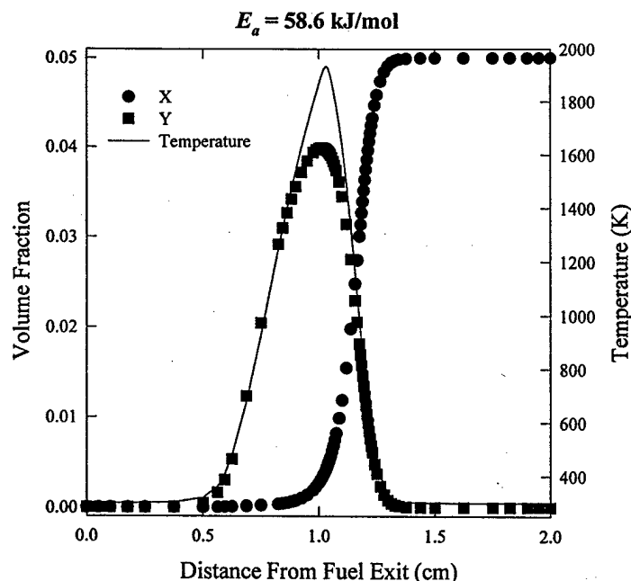
Figure 56. The volume fractions of X and Y are plotted as a function of distance from the fuel exit for a methane flame burning in air with 5 % added X. X reacts to form Y with E_a = 58.6 \text{ kJ/mol} and \Delta H_{X-Y} = 96.1 \text{ kJ/mol} . The spatial variation of temperature is also shown as the solid line. Methane and oxidizer exit velocity magnitudes are 25 cm/s.
