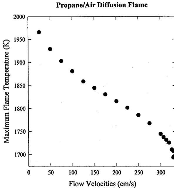
Figure 17. Maximum flame temperatures are plotted as a function of the equal fuel and air velocity magnitudes for a propane/air opposed-flow diffusion flame.
