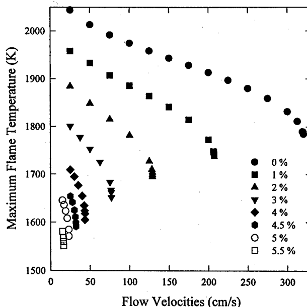
Figure 63. Maximum calculated flame temperatures are plotted against methane and oxidizer exit velocity magnitudes for a series of methane/air opposed-flow diffusion flames diluted with C_4F_9OCH_3 . Symbols correspond to the volume fractions of added C_4F_9OCH_3 .
