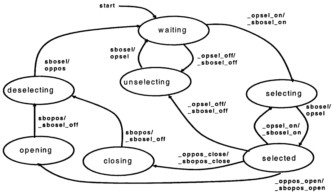
Figure 18: CSWI State Machine
