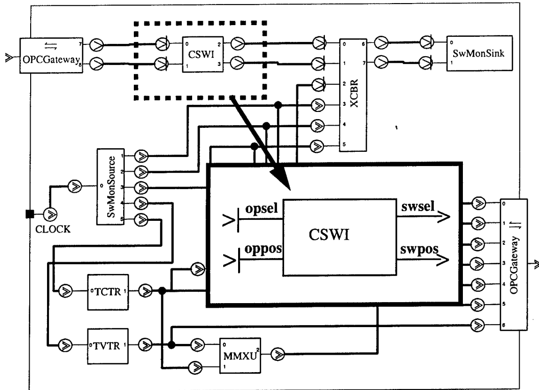
Figure 16: Controller System Diagram
