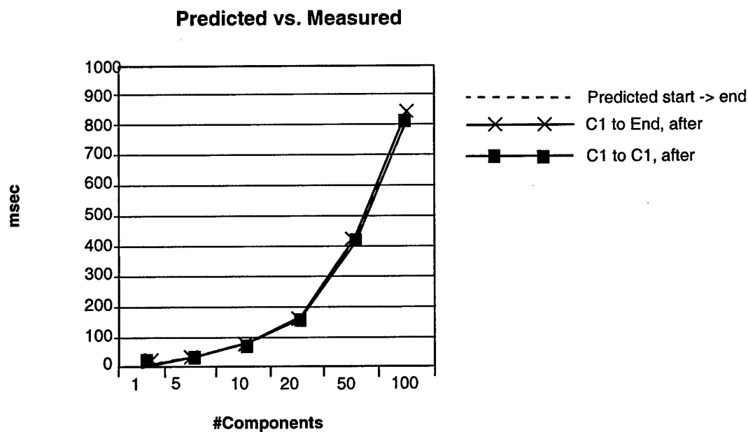
Figure 21: Results of Spot Validation of Operator PECT Latency Theory
