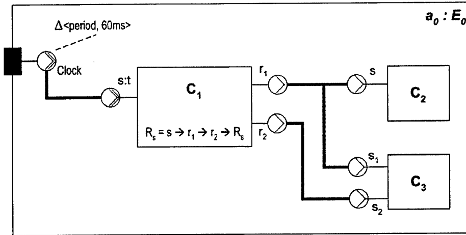
Figure 33: Assembly with Synchronous Pins and Non-Linear Topology
