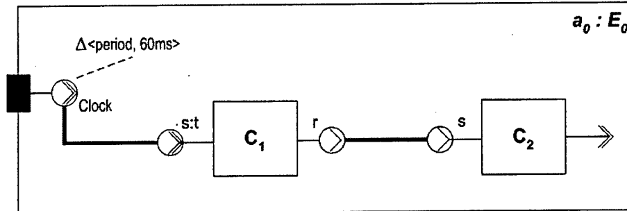
Figure 30: Simple Constructive Assembly
