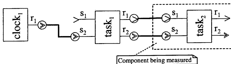
Figure 52: General Assembly Topology for Benchmarking Synthetic Components
