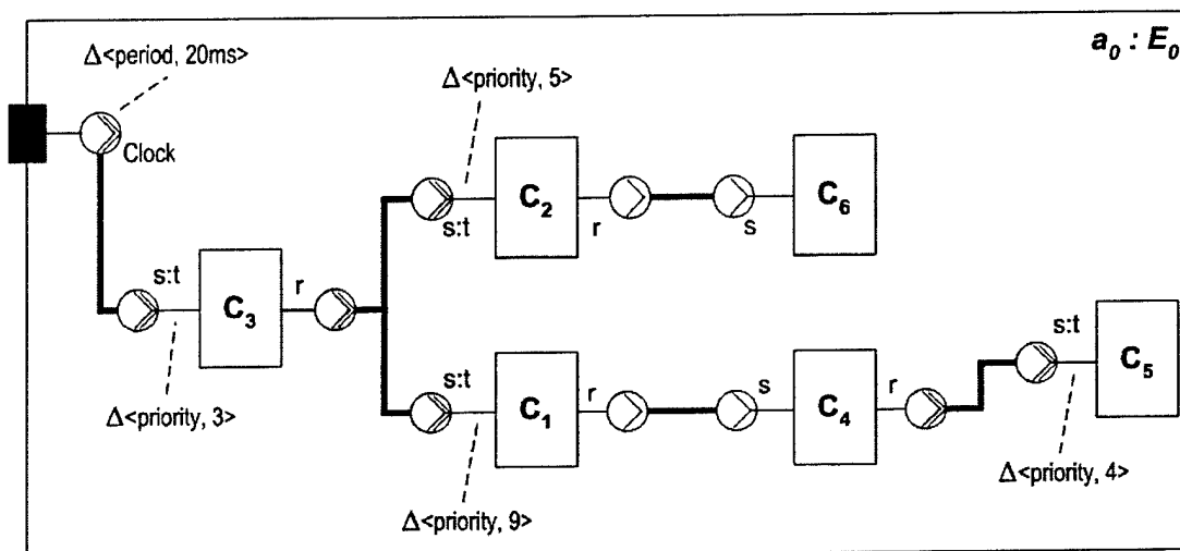
Figure 39: Multiple Synchronous Connections Problem
