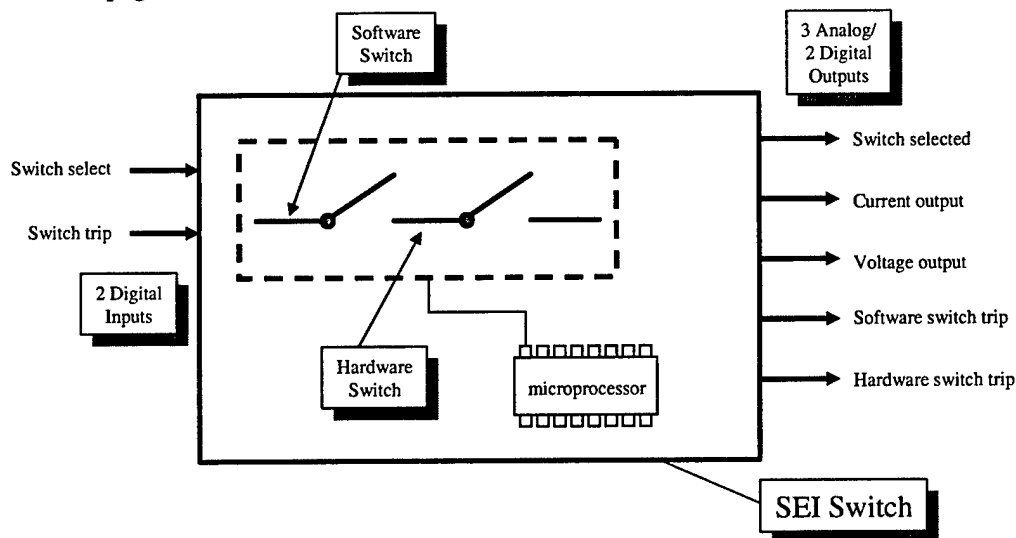
Figure 3: SEI Switch Abstraction
