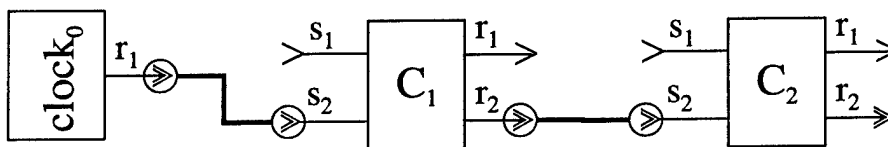
Figure 56: Topology of an Example of a Randomly Selected Assembly
