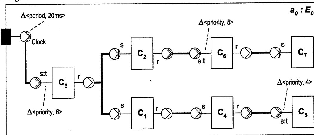
Figure 37: Asynchronous Connections Following Synchronous Connections
