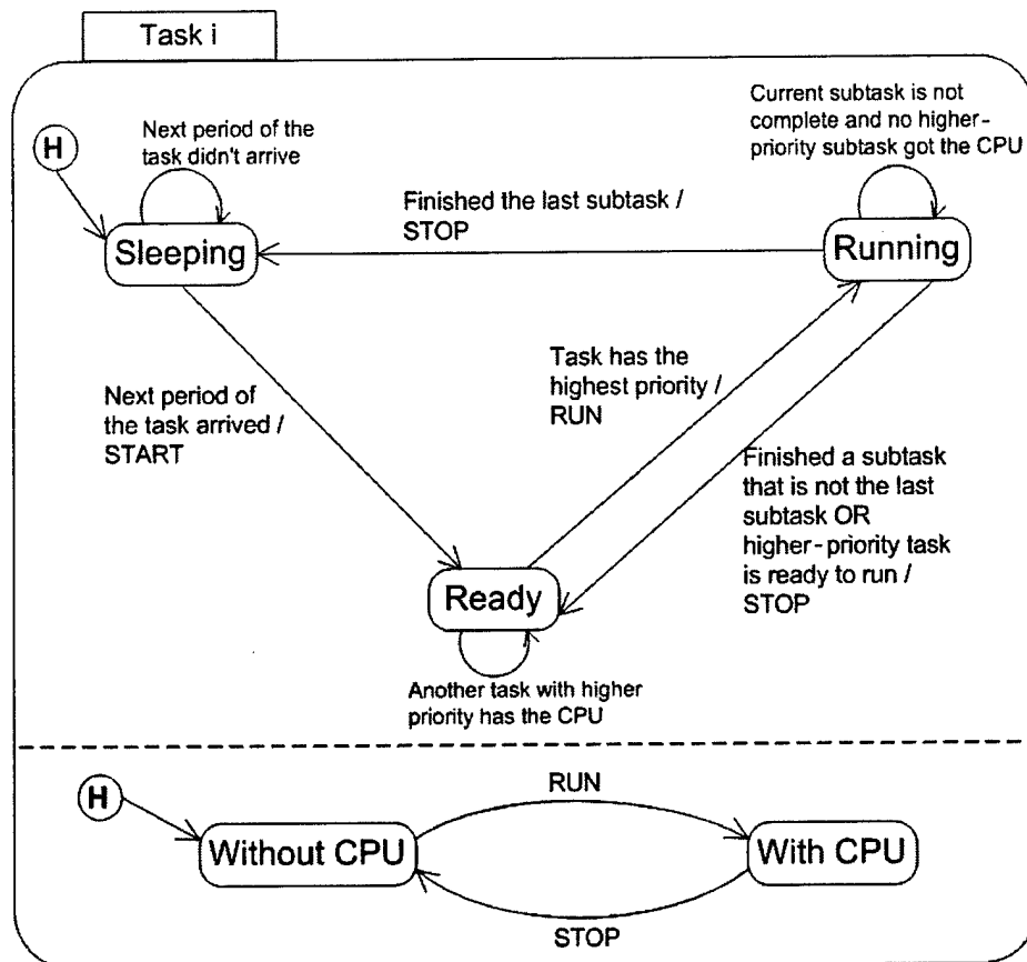
Figure 28: Task Statechart Diagram
