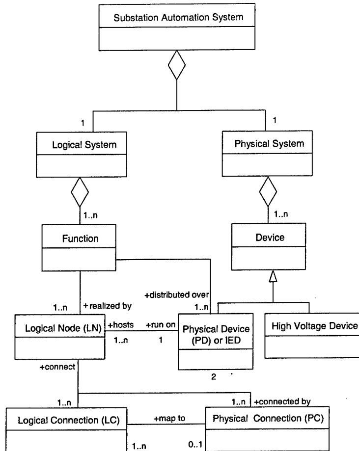
Figure 2: Key Concepts of the IEC 61850 Standard for a SAS Model Problem
