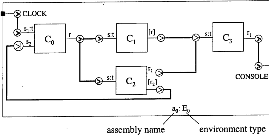
Figure 7: A Simple Assembly
