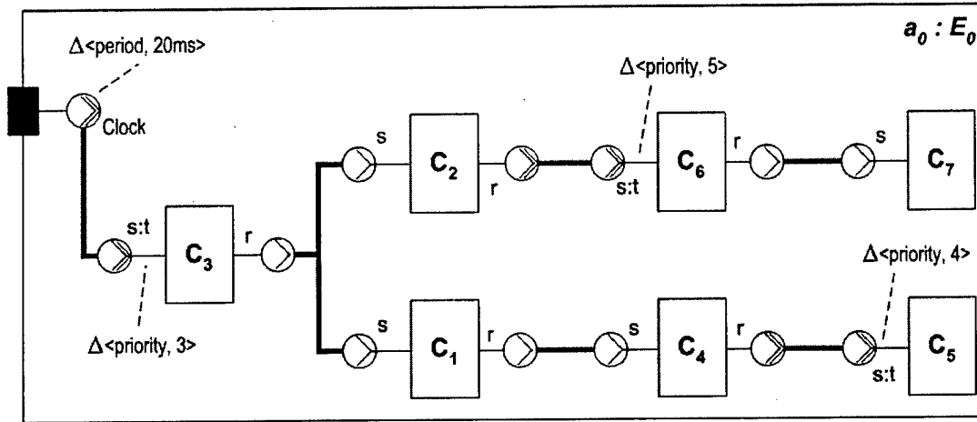
Figure 38: Asynchronous Connections and Reentrant Synchronous Connections
