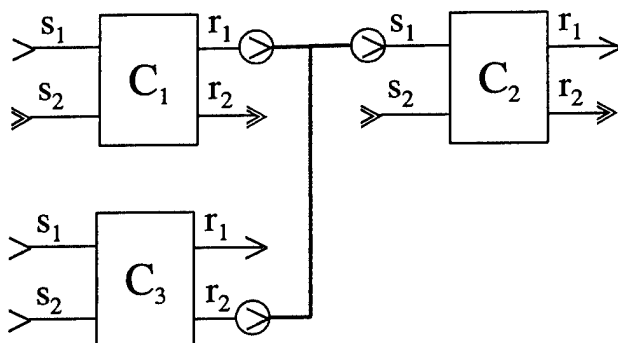
Figure 47: A Simple Many-to-One Interaction
