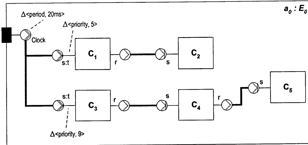
Figure 36: Synchronous Connections Following Asynchronous Connections
