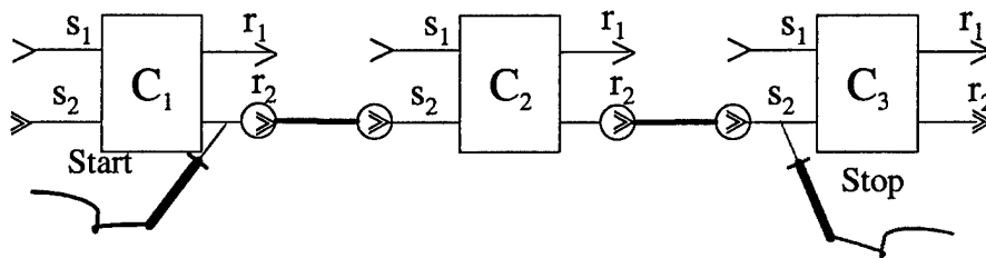
Figure 49: Measuring the Latency for a Simple Assembly
