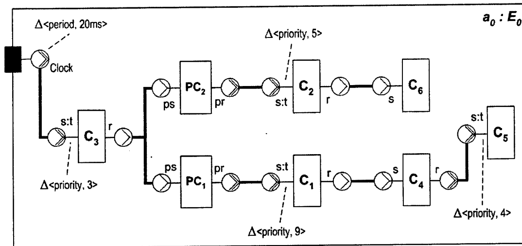
Figure 40: Multiple Asynchronous Connections Rewrite Rule Using Proxy Components
