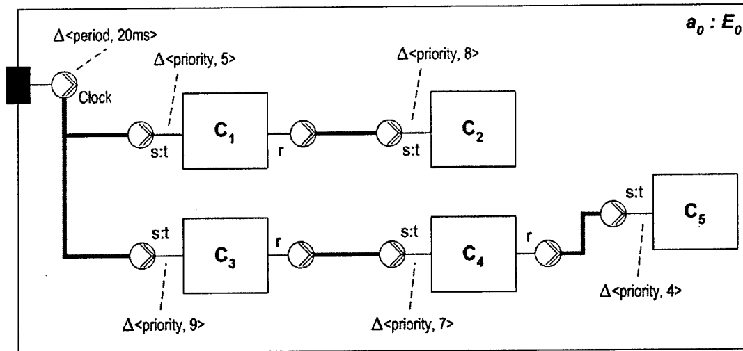
Figure 35: Constructive Assembly with Asynchronous Connections
