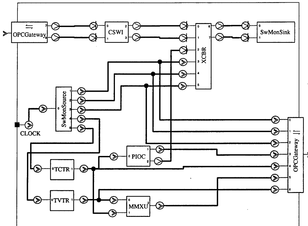
Figure 9: SAS Software Controller in Pin 17
