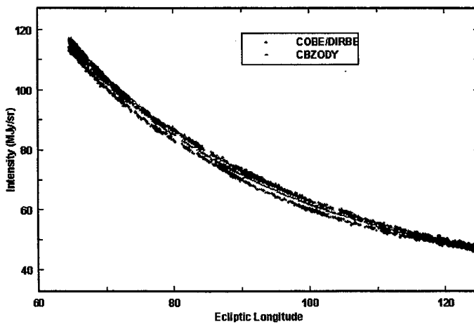
Figure 61: In-plane fits to the CIO data.
