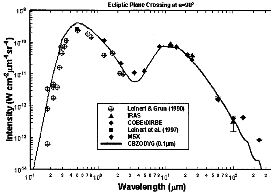
Figure 51: Similar to Figure 50 the zodiacal spectrum out to 300\mu m . The deviations at 140\mu m and 230\mu m between the model and COBE/DIRBE data are due to the lack of a galactic dust (cirrus) model and not errors in the zodiacal dust model.
