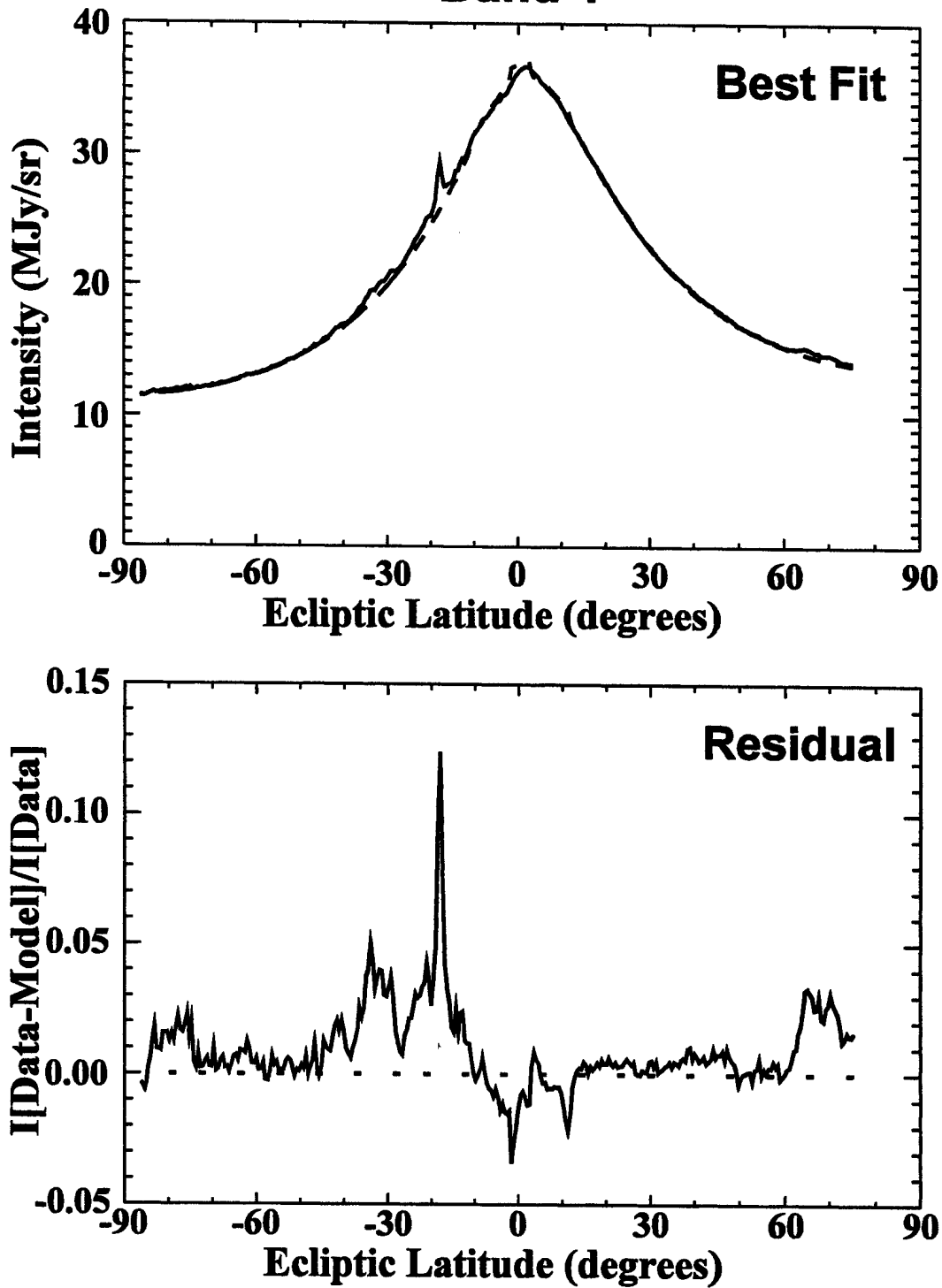
Figure 13: NLS fit to an IRAS scan. This fit is typical of the NLS fits to the IRAS data. Top, the solid line shows the IRAS observations and the dashed line is the CBZODY fit. Bottom, the residual in the sense IRAS-CBZODY (solid line) with a 0 MJy/sr reference line (dashed).
