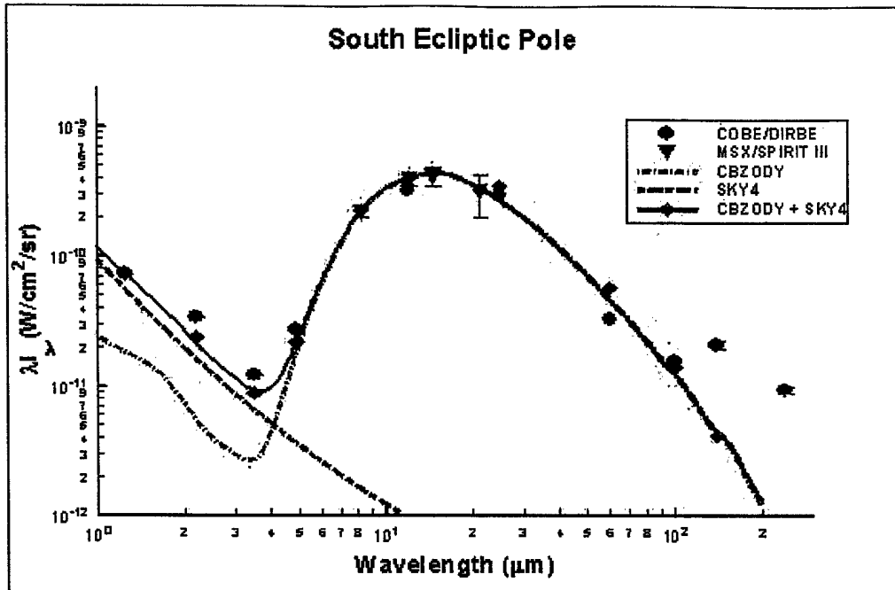
Figure 39: CBZODY and SKY4 over the DIRBE bands. The averaged COBE/DIRBE observations of the SEP compared to CBZODY6, SKY4, and a combined CBZODY/SKY4 model.
