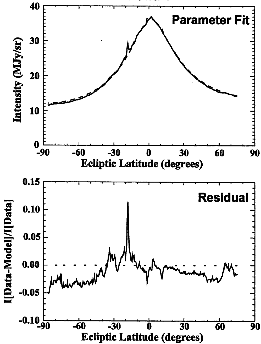
Figure 14: Fit to an IRAS scan using the generalized parameter set. Like figure 13, this fit is typical of the generalized parameter set fits to the IRAS data.
