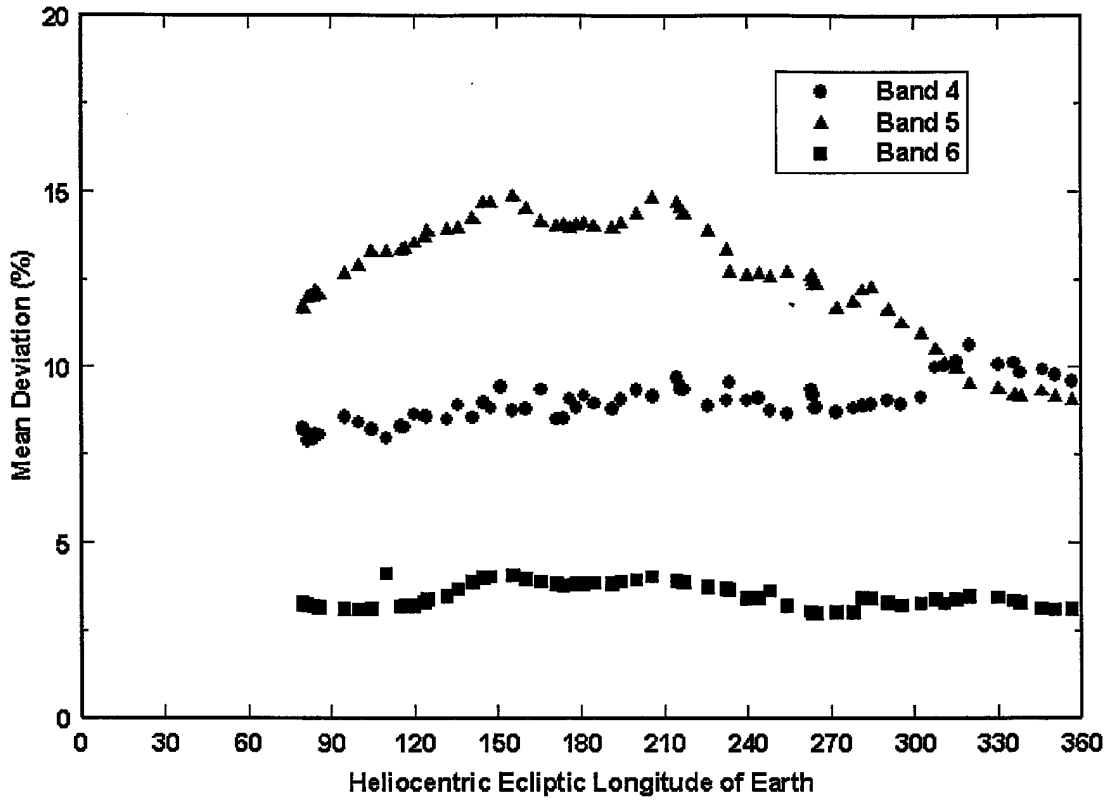
Figure 56: Mean deviation errors versus Heliocentric ecliptic longitude of Earth. The three COBE/DIRBE bands are plotted with the mean error for one CIO day versus heliocentric ecliptic longitude of Earth. Band 5 shows the highest deviation as expected from the fit to the ISO spectrum of Figure 48.
