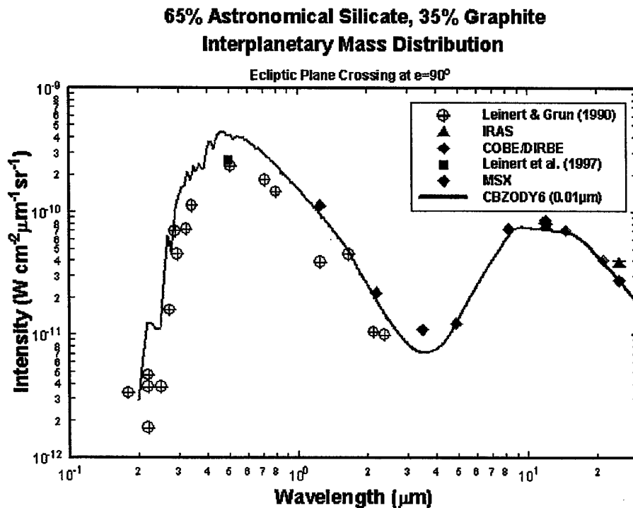
Figure 50: Zodiacal spectrum, solid line, compared to a variety of data sets for a 90° elongation. Between 1 and 3μm, discrepancies appear between the Leinert and Grün data and the COBE/DIRBE data. We chose to weight the COBE/DIRBE data more heavily in the fit.
