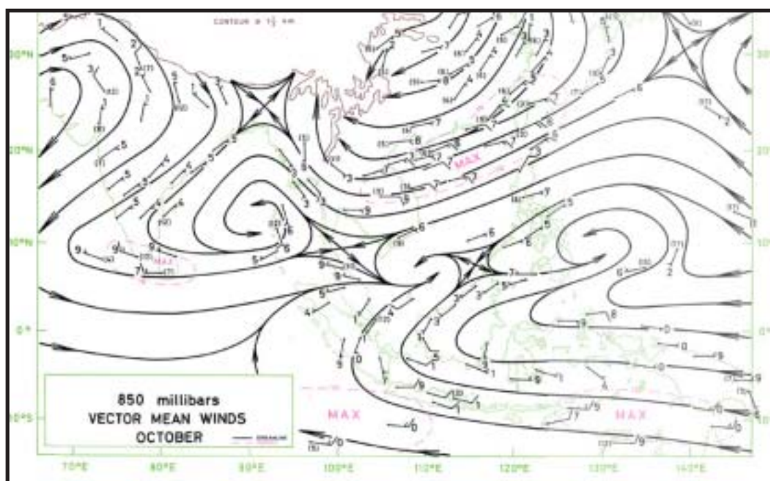
Figure 2-26d-1. Streamline Analysis at 850 mb for October. The full solid lines depict streamlines (arrowheads indicate direction).
