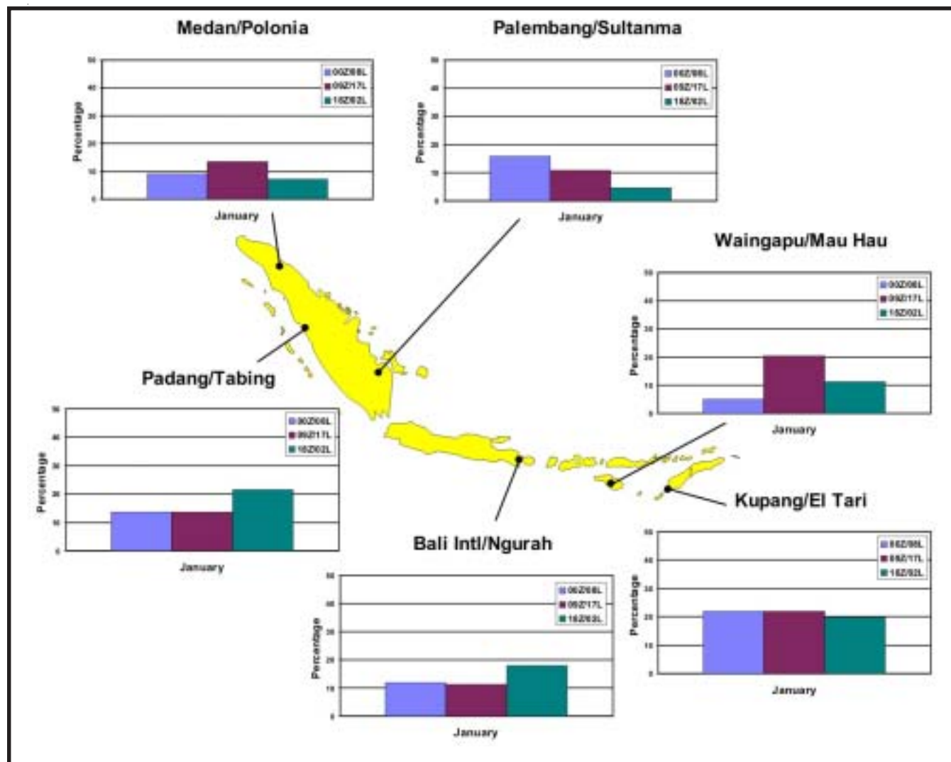
Figure 3-3. Northeast Monsoon Season Percent Frequency of Ceilings below 3,000 Feet. The graphs show a monthly breakdown of the percent of ceilings below 3,000 feet based on location and diurnal influences.
