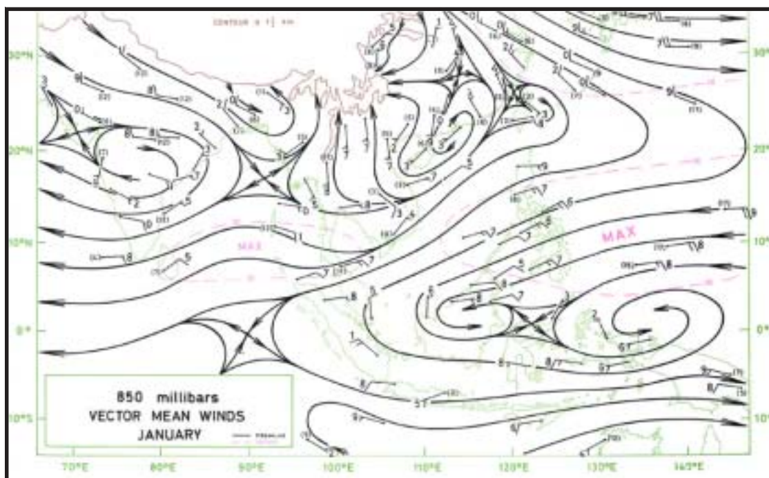
Figure 2-26a-1. Streamline Analysis at 850 mb for January. The full solid lines depict streamlines (arrowheads indicate direction).
