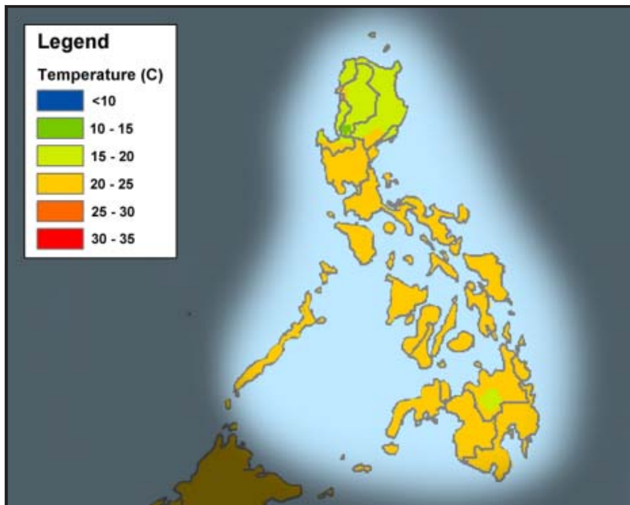
Figure 6-10. January Mean Minimum Temperatures (°C). Mean minimum temperatures represent the average of all daily low temperatures for the coldest month of the northeast monsoon. Daily low temperatures are often lower than the mean.
