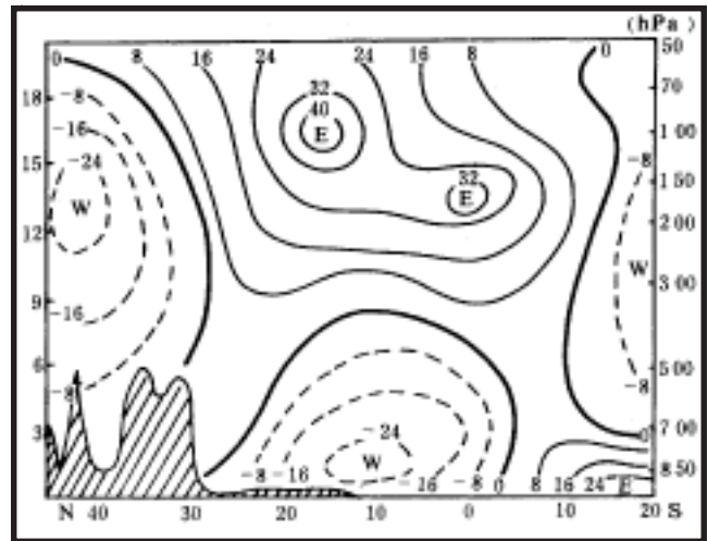
Figure 2-24. Cross-Section of the Mean Zonal Wind Component along 80E in July. Solid (dashed) lines denotes isotach of easterly wind (westerly wind). Units: m/s. (From Yihui, 1994).
