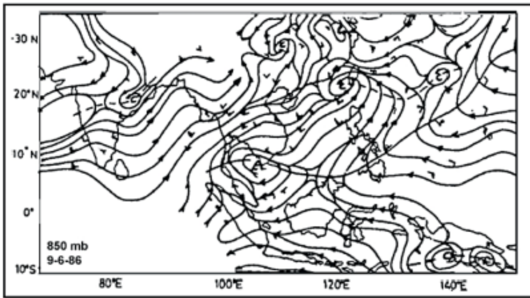
Figure 2-14. Streamline Analysis (850 mb) from 9 June 1986. This analysis shows presence of an equatorial anticyclone over the Gulf of Thailand. This anticyclone migrated northward to cause a “monsoon break” to occur. (From Cheang and Tan, 1988).
