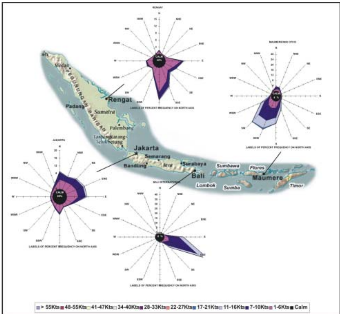
Figure 3-13. July Surface Wind Roses. The figure shows the prevailing wind direction and range of speeds based on frequency and location.
