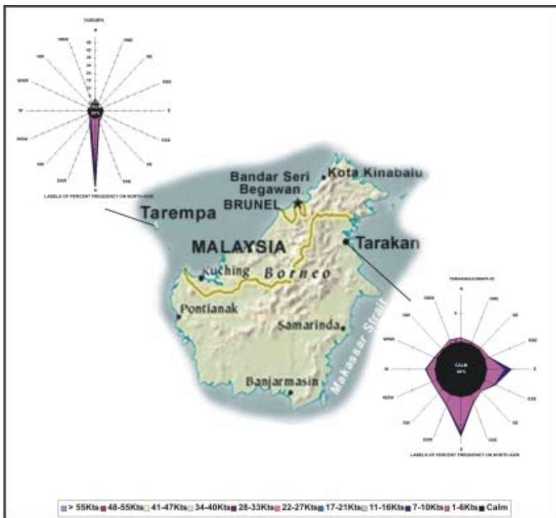
Figure 4-13. July Surface Wind Roses. The figure shows the prevailing wind direction and range of speeds, based on frequency and location.
