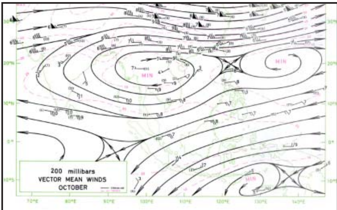
Figure 2-26d-4. Streamline Analysis at 200 mb for July. The full solid lines depict streamlines (arrowheads indicate direction).
