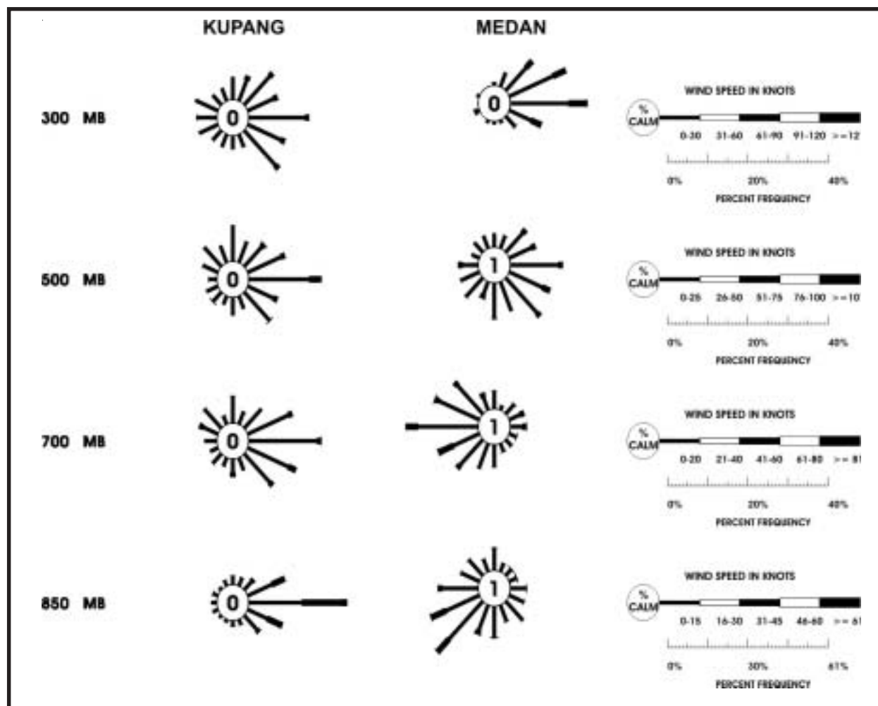
Figure 3-14. July Upper-Air Wind Roses. The wind roses depict wind speed and direction for standard pressure surfaces between 850 and 300 mb for selected locations.
