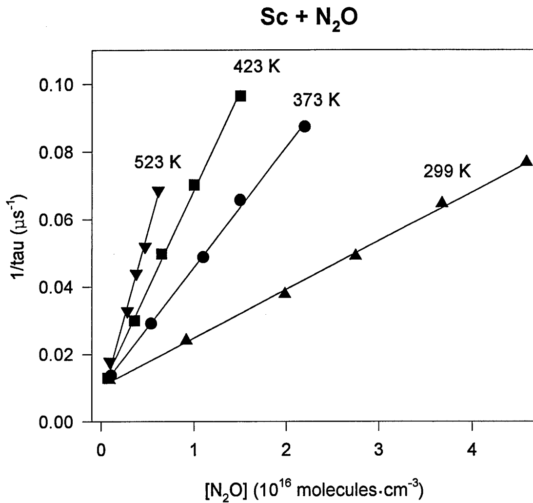
Figure 11. Plot for determining the second-order rate constant, k_{2\text{nd}} , for Sc + N 2 O. The slope of the regression line yields k_{2\text{nd}} in \text{cm}^3\text{s}^{-1} .
