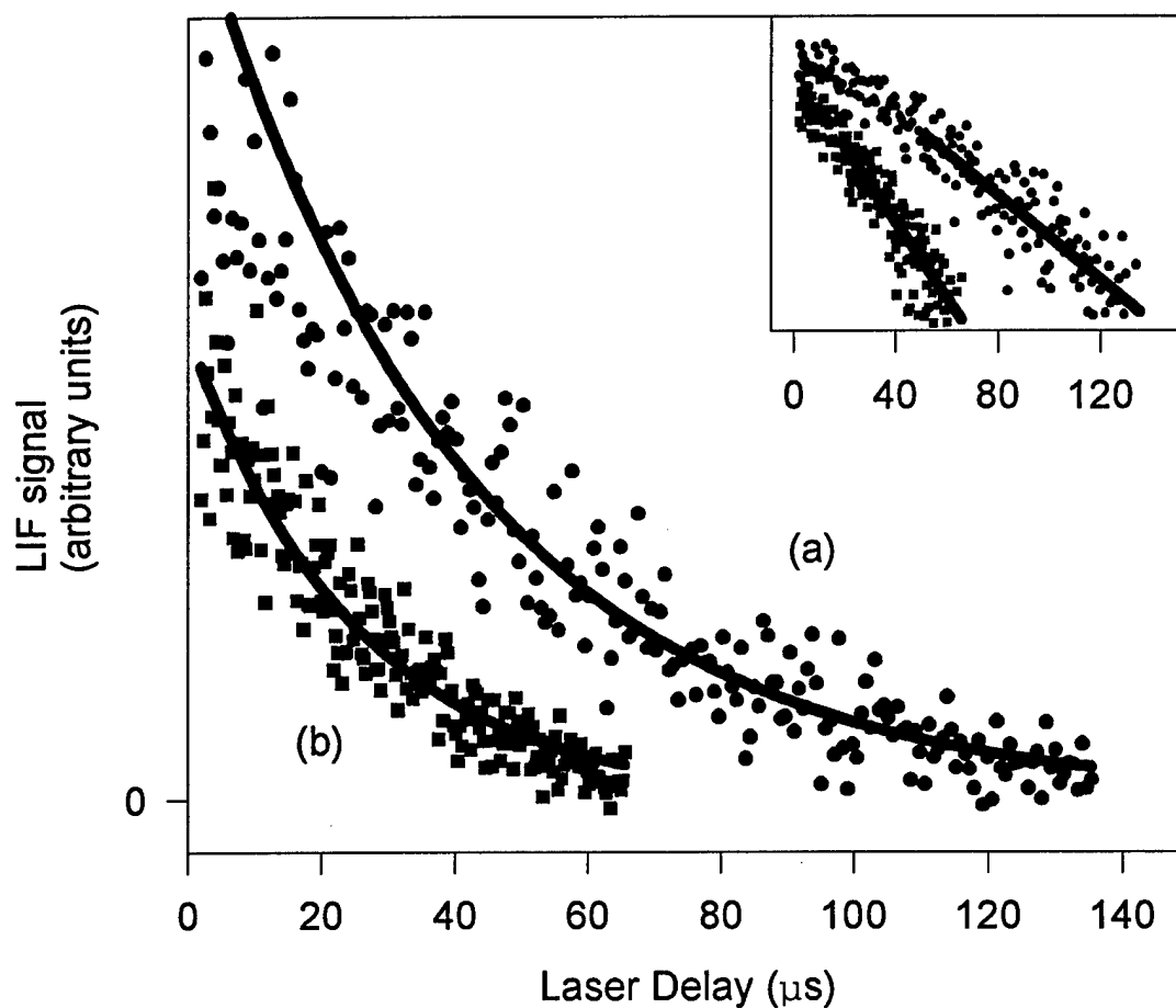
Figure 7. Decay profile for \text{Cr}(\text{CO})_6 . T = 473\text{K} , P_{\text{total}} = 20\text{ Torr} . Solid lines are exponential fits to the data. (a) P(\text{N}_2\text{O}) = 2.44\text{ Torr} , \tau = 61\ \mu\text{s} and (b) P(\text{N}_2\text{O}) = 8.63\text{ Torr} , \tau = 22.9\ \mu\text{s} . The inset plot is a log fit to the data.
