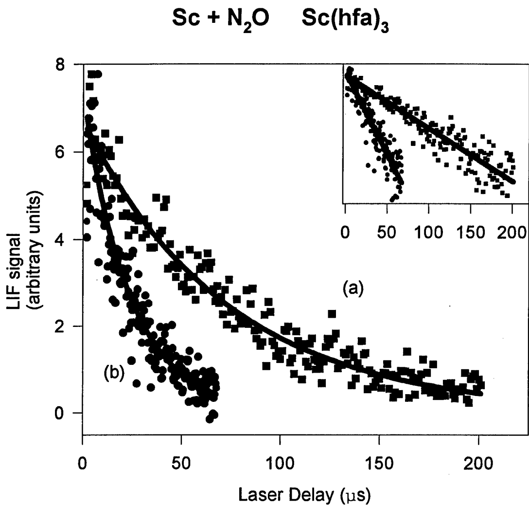
Figure 5. Decay profile for Sc(hfa) 3 , T = 299\text{K} , P_{\text{total}} = 20\text{ Torr} . Solid lines are exponential fits to the data. (a) P(\text{N}_2\text{O}) = 0.0516\text{ Torr} , \tau = 72.1\ \mu\text{s} and (b) P(\text{N}_2\text{O}) = 0.723\text{ Torr} , \tau = 23.1\ \mu\text{s} . The inset plot is a log fit to the data.
