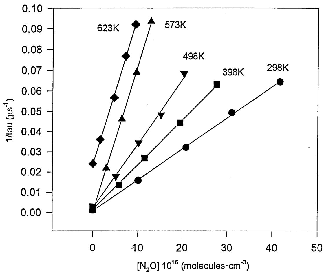
Figure 14. Plot for determining the second-order rate constant, k_{2\text{nd}} , for Ni + N 2 O as a function of temperature. The slope of the regression line yields k_{2\text{nd}} in \text{cm}^3\text{s}^{-1} .
