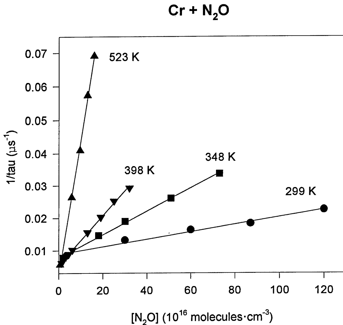
Figure 12. Plot for determining the second-order rate constant, k_{2\text{nd}} , for Cr + N 2 O. The slope of the regression line yields k_{2\text{nd}} in \text{cm}^3\text{s}^{-1} .
