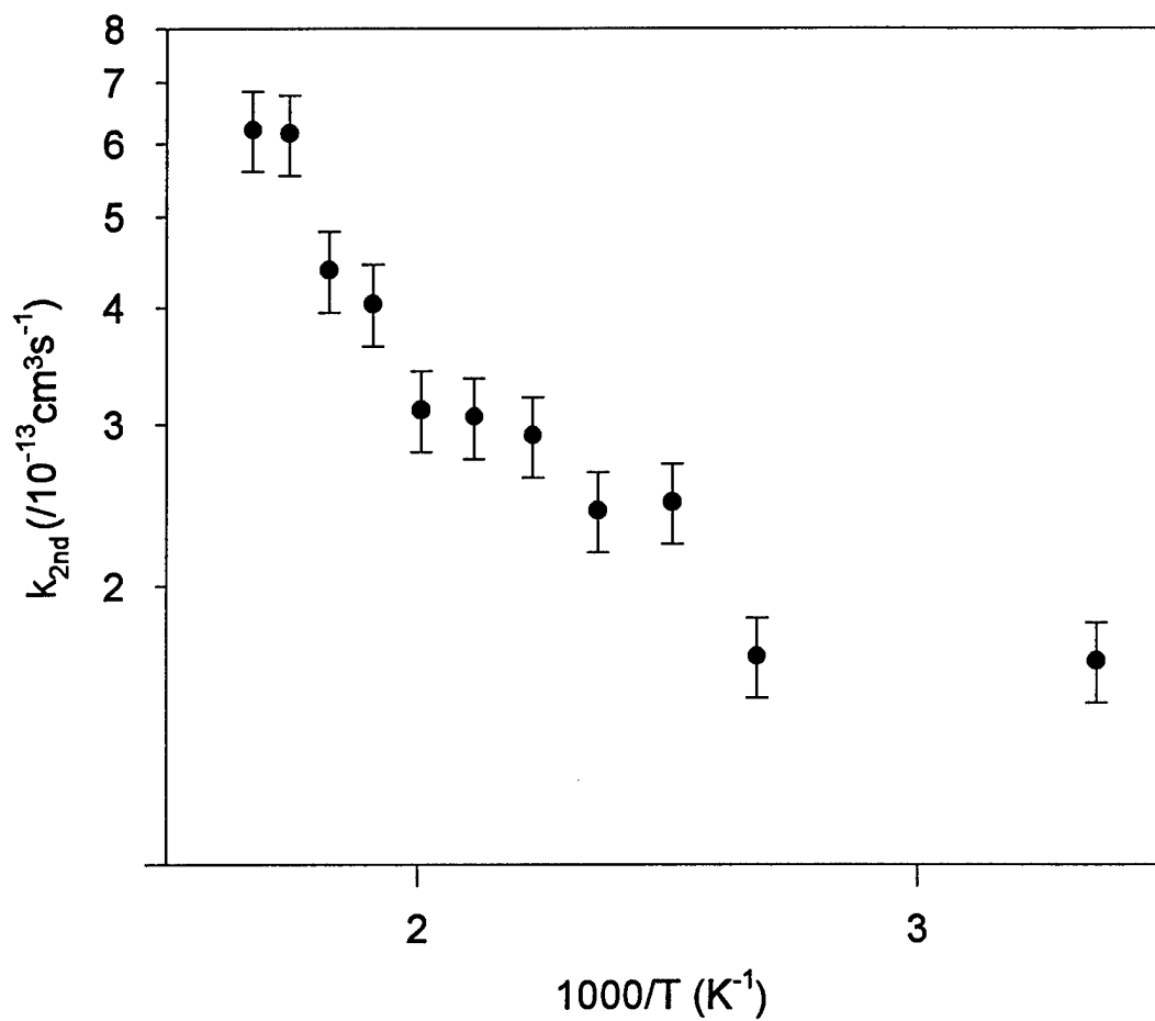
Figure 17. Arrhenius plot for Ni + N 2 O showing pressure dependence at low temperatures. Error bars represent \pm 10\% uncertainty.
