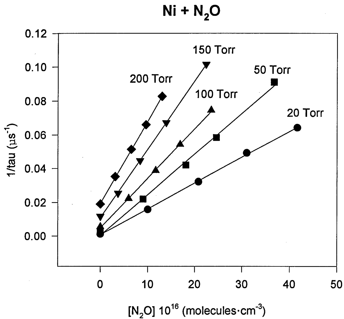
Figure 15. Plot for determining k_{2\text{nd}} as a function of pressure. As shown in the graph, Ni + N 2 O was found to be pressure dependent. Data shown is for T = 298K. The slope of the regression line yields the second-order rate constant for each pressure.
