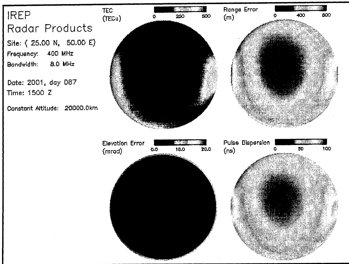
Figure 20. An Example of the IREP Graphical Display for a Hypothetical Radar Sited at (25 N, 50 E) Operating at a Frequency of 400 MHz with a Bandwidth of 8 MHz on 28 March 2001 (day 87) at 1500 UT. The display shows TEC, range error, elevation error, and pulse dispersion. The display is normally in color, but is reproduced here in gray scale.
