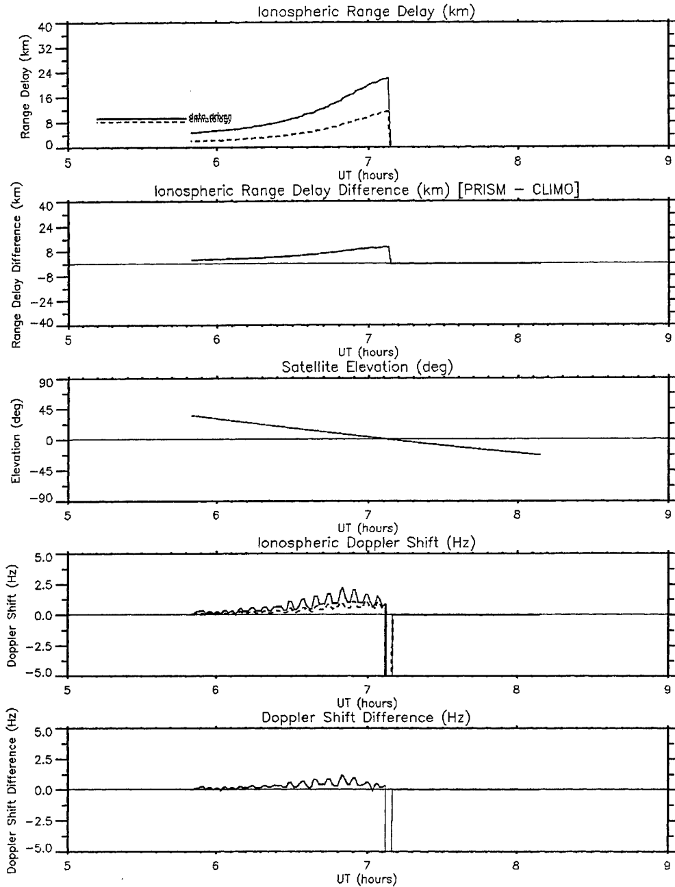
Figure 25. Comparison of PRISM Climatology and Data Assimilation Runs for 24 October 2002 Using the Full Data Set Supplied by Dr. Borer and a Simulated HEO Satellite. The top panel shows range delay from PRISM climatology (dashed) and PRISM data assimilation (solid). The next panel shows the difference between the two. The middle panel shows the satellite elevation, which shows that the satellite passed below the horizon shortly after 0700 UT. The next panel shows the ionospheric contribution to the Doppler shift for climatology and data assimilation. Finally the bottom panel shows the difference between the two.
