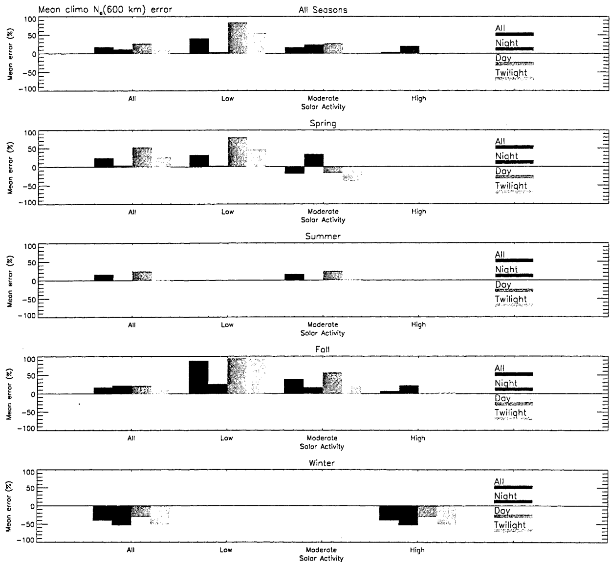
Figure 12. Mean Climatological n_e(600 \text{ km}) Error for Each Combination of Season, Solar Activity, and Local Time. Although the overall bias is positive (but very small at night) the climatological error shows considerably more variability than the corresponding PRISM error. The winter bias is negative for all local times (although that is based on a miniscule number of profiles).
