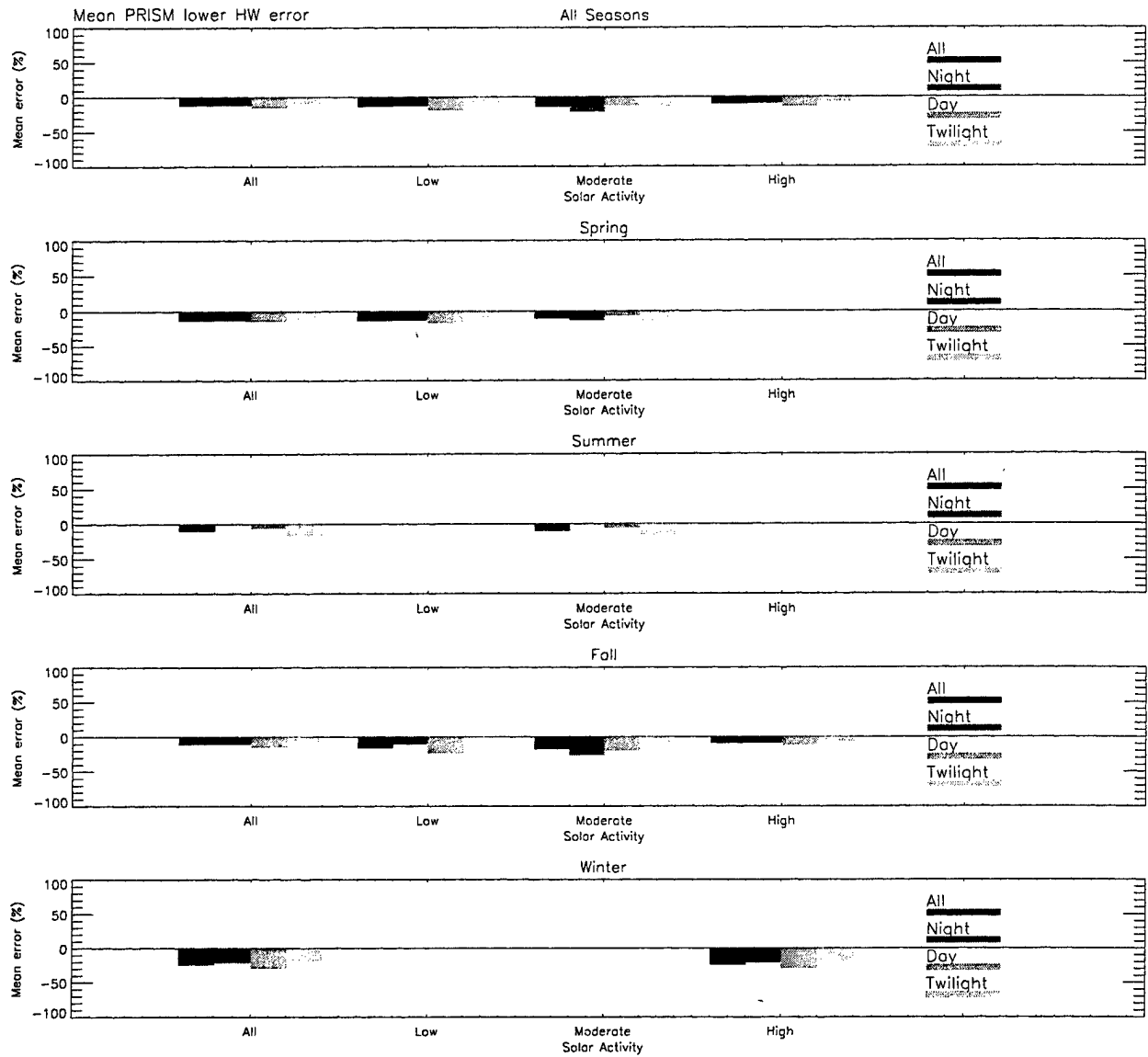
Figure 8. Mean Lower Half-Width Error for Each Combination of Season, Solar Activity, and Local Time. As expected from the behavior of the bottomside TEC, the bottomside half-width also displays a generally negative bias with very little difference between day and night.
