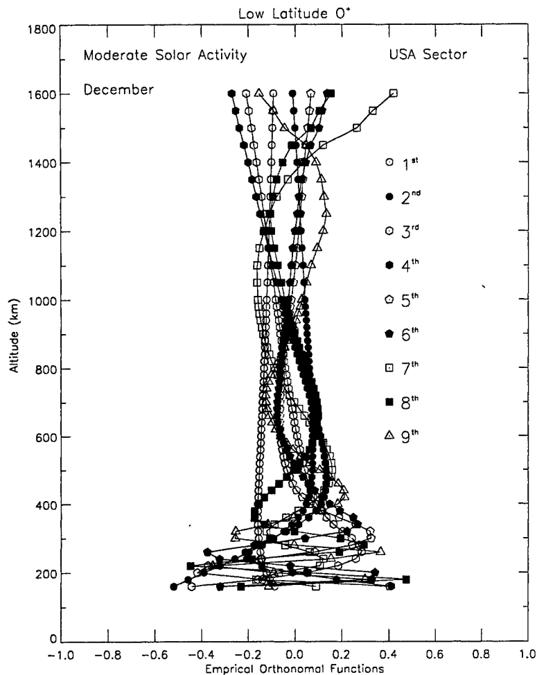
Figure A1. The Empirical Orthonormal Functions (EOF's) for low latitude \text{O}^+ derived from the LOWLAT output databases for the USA longitude sector, December solstice, moderate magnetic activity, and moderate solar activity. Only the first nine EOF's are plotted because these are the ones used in PRISM.
