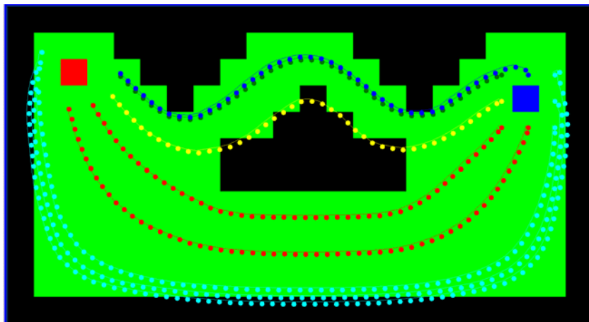
Figure 8. Edge Effects.
