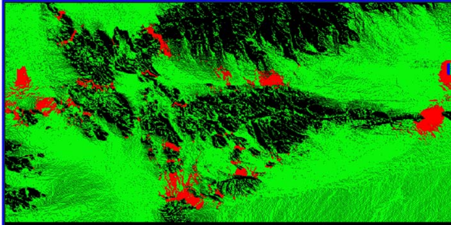
Figure 11. Chokepoints.
