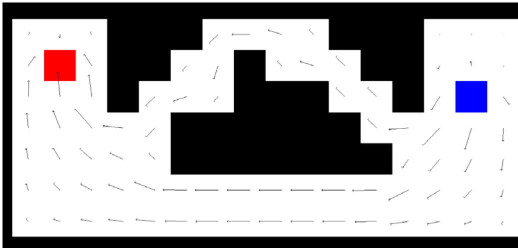
Figure 5. Gradient Vectors.
