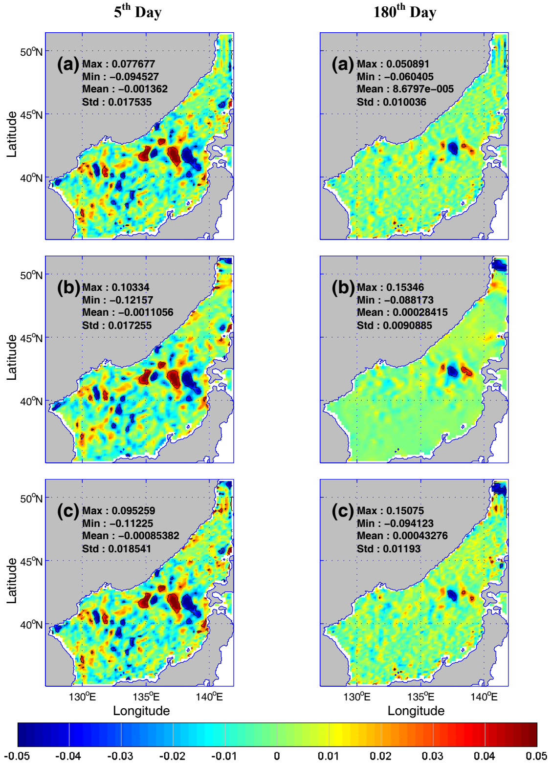
Figure 31. Vertically averaged model error of (a) Run 0 – Run 9, (b) Run 0 – Run 10 and (c) Run 0 – Run 11 for v component of velocity field on both the 5 th and 180 th day after the model integration.
