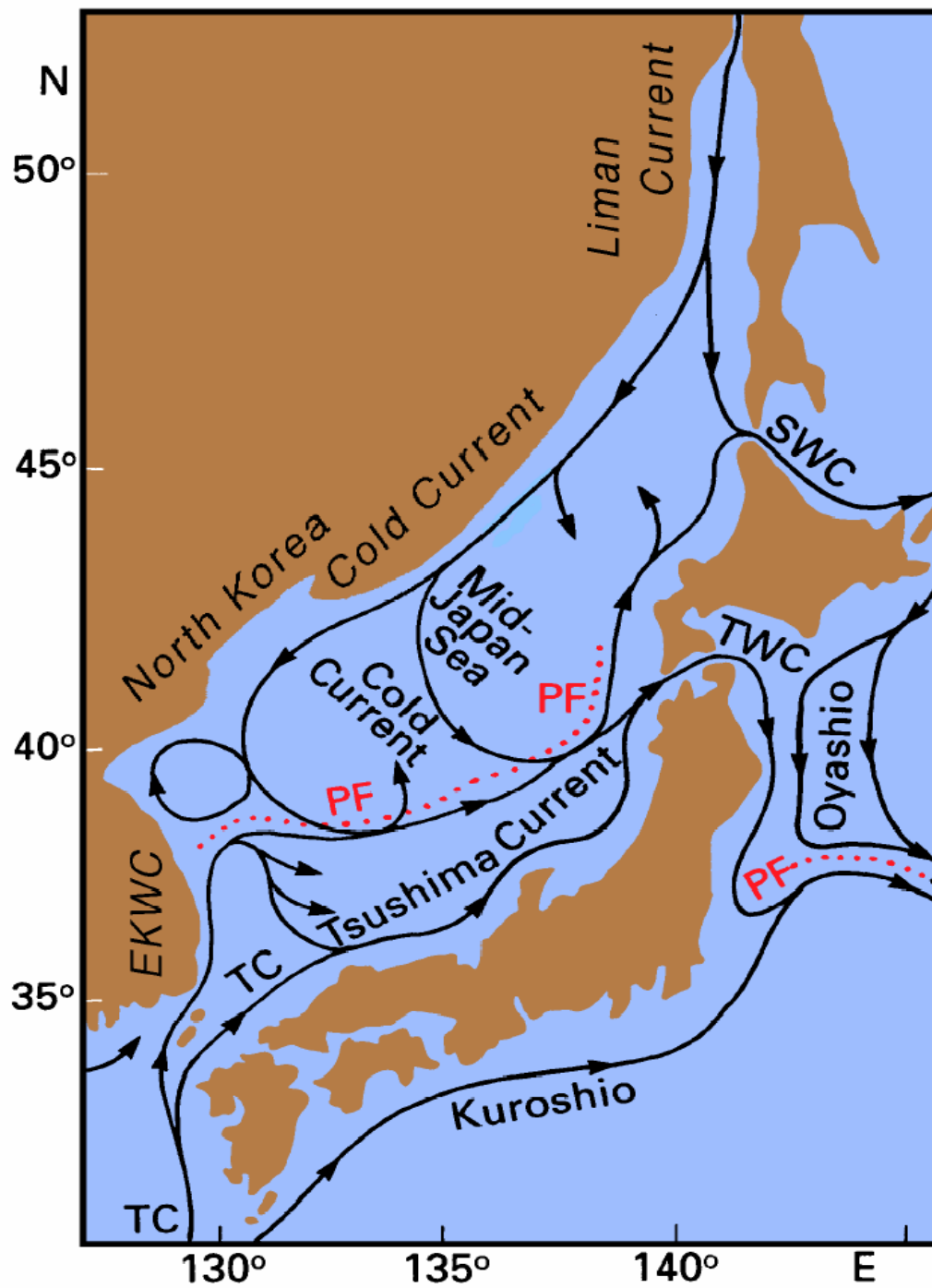
Figure 2. Current system in the Japan/East Sea (from Tomczak and Godfrey, 1994).
