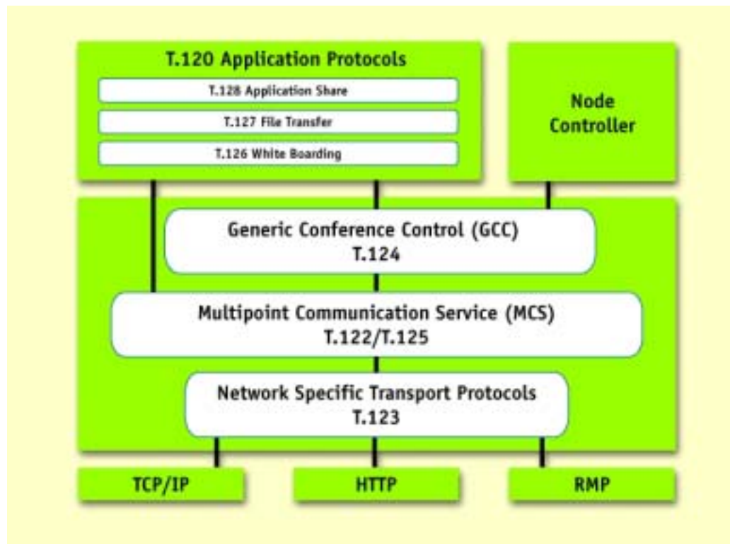
Figure 19. T.120 Application Protocols (from [31])
