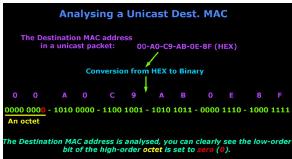
Figure 7. Analyzing a Unicast Destination MAC Address (from [3])
