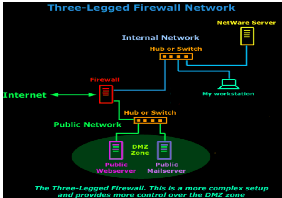
Figure 4. Three-Legged Firewall Network (from [6])
