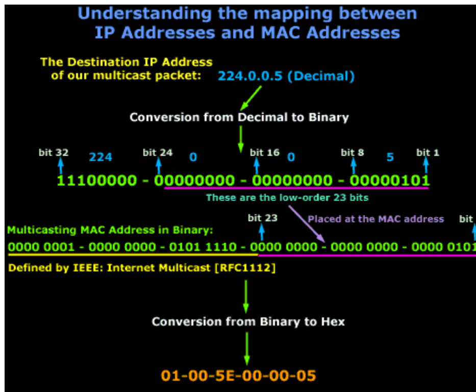
Figure 11. Mapping Between IP Addresses and MAC Addresses (from [3])
