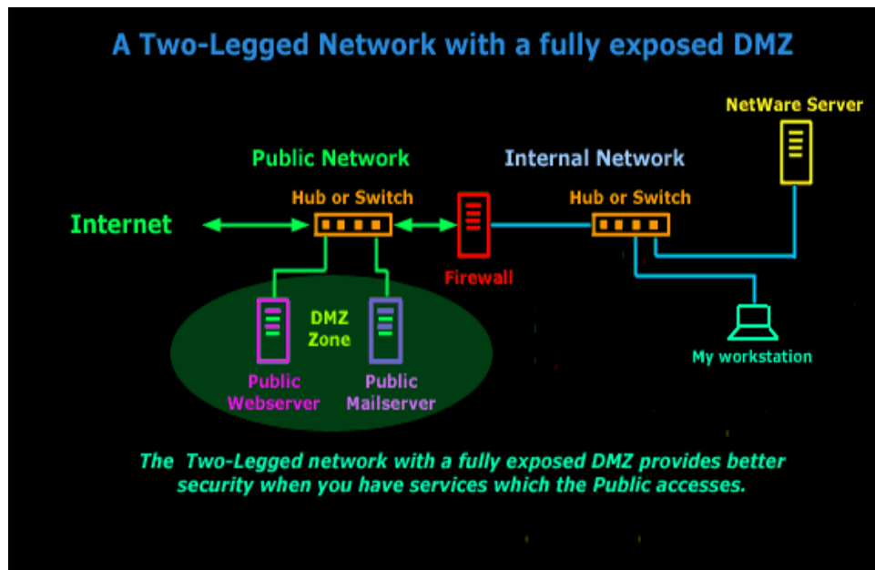
Figure 2. Two-Legged Network with exposed DMZ (from [6])
