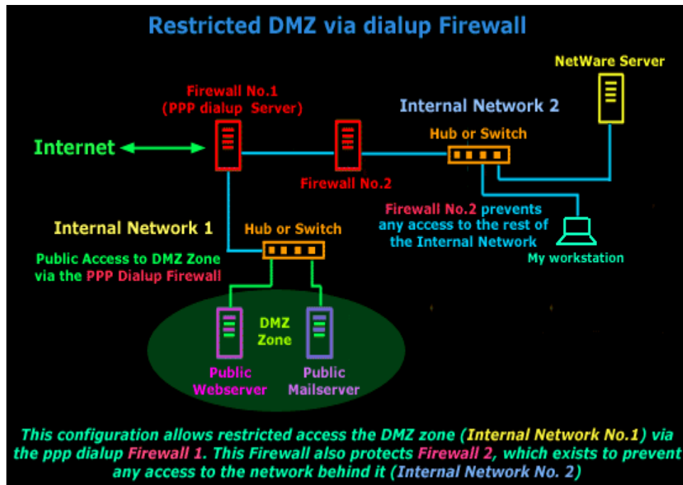
Figure 3. Restricted DMZ via dialup Firewall (from [6])
