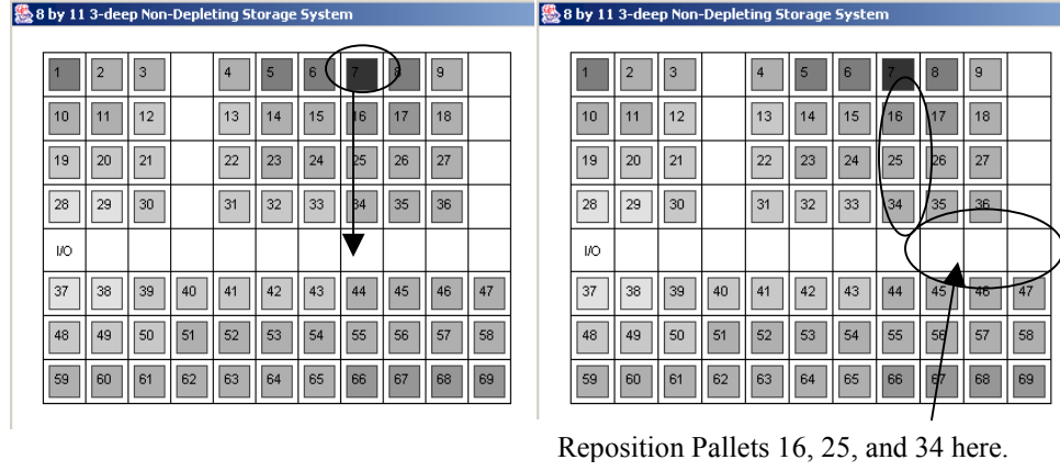
Figure 16 Illustration of a Better Pallet Repositioning Move
