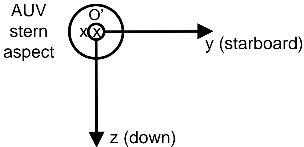
Figure 16. Stern view of the body fixed reference frame with origin O' and the x -axis going into the page.
