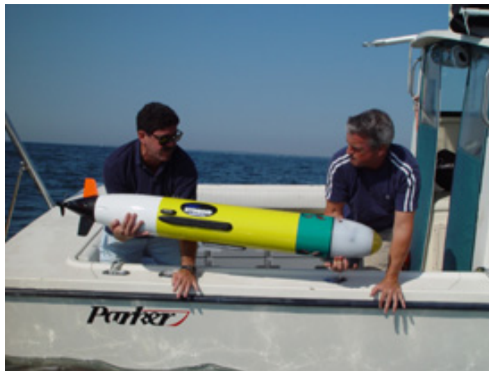
Figure 4. Hydroid’s Remote Environmental Measurement UnitS (REMUS) AUV is two-man portable and does not require specialized equipment or a crane for deployment or recovery (from Hydroid 2003).
