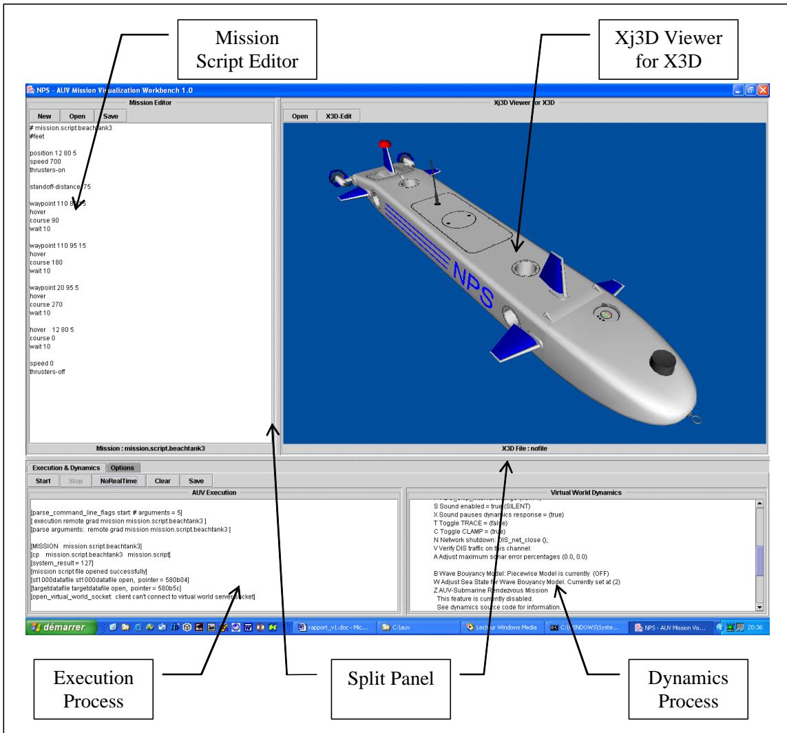
Figure 22. The graphical user interface (GUI) for the original AUV Workbench (from Grunesien 2002).
