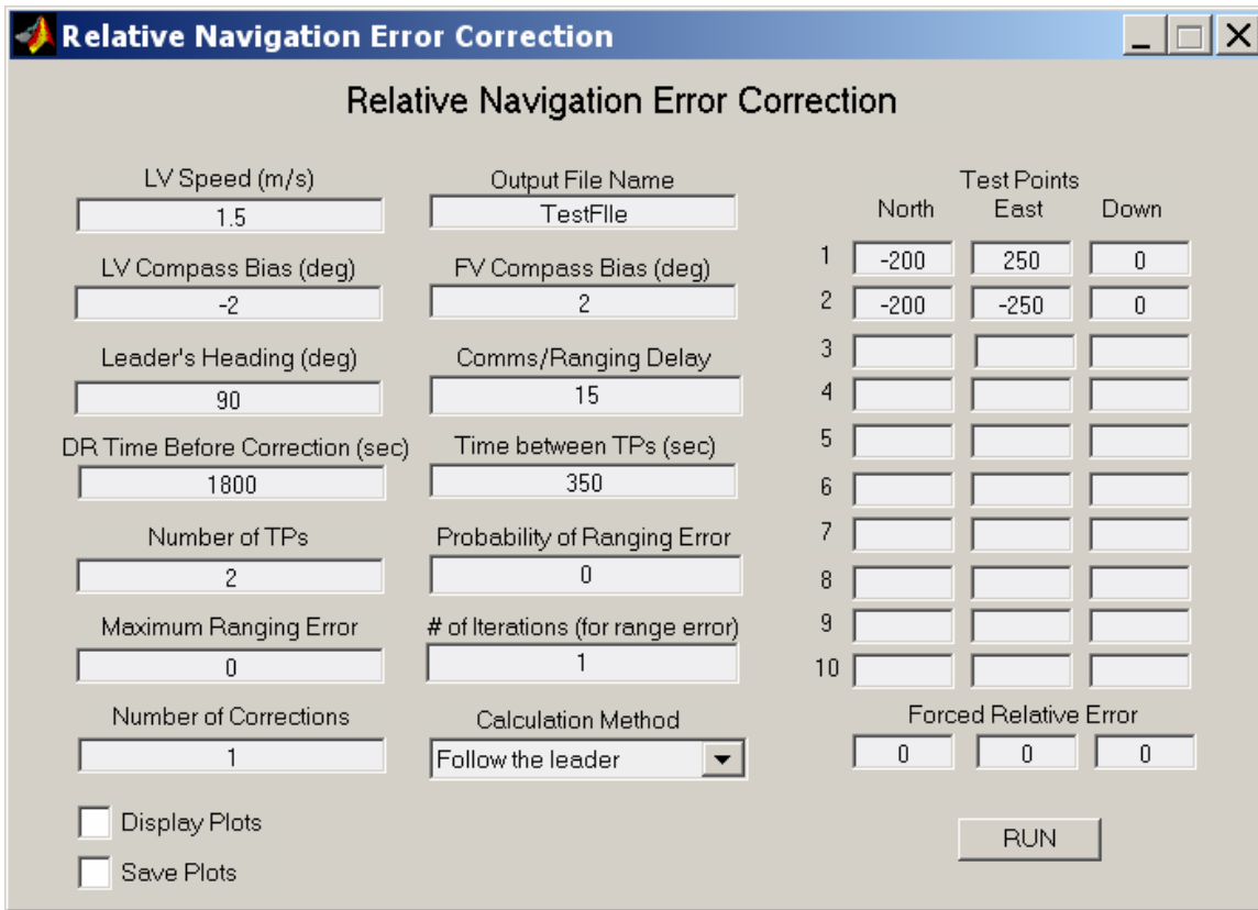
Figure 45. The graphical user interface (GUI) for the Matlab-based relative navigation error correction simulation.
