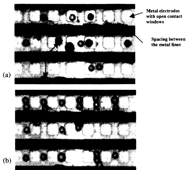
Figure 7 The movements of negatively charged polystyrene beads while the magnitude and the frequency of applied AC signal were changed. (a) No bias, random bead distribution, (b) 10V p-p and 10MHz, beads settle in middle of open windows within one electrode.
