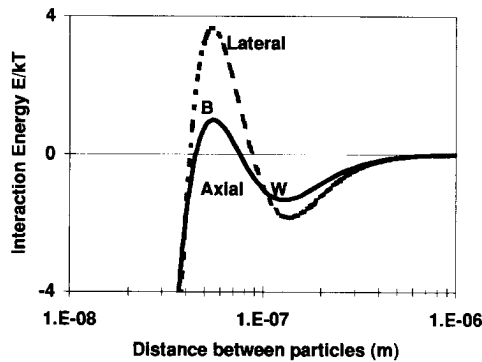
Figure 3. Graphs E_{AXI}/kT (solid line) and E_{LAT}/kT (dashed line) vs. distance between carbon plain blocks 200 \times 200 \times 400 nm in polyethylene at 190^\circ\text{C} , n = 1.5 \text{E}21 \text{ m}^{-3} , z = 4 , \gamma_0 = 1
