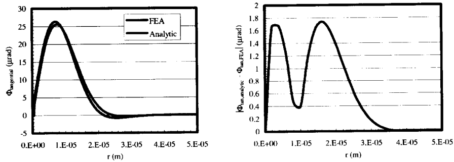
Figure 5. Simulated tangential beam deflection data and error between the FEA and analytical models.
