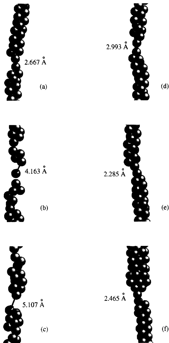
Figure 3. Snapshots of the morphologies of nanowires at the moments they break. The elongation speeds and temperatures are (a) 1.95m/s and 4K, (b) 1.95m/s and 300K, (c) 1.95m/s and 500K, (d) 0.391m/s and 4K, (e) 0.391m/s and 300K, and (f) 0.391m/s and 500K, respectively. The distances of the atoms at the points where breakings occur are indicated.
