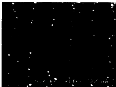
Figure 5. SEM micrograph of an ordered array of 150 nm diameter Ag "nano-bracelets" created with the FIB-PLD process. The individual particles making up the bracelets range from <10 nm to ~30 nm.
