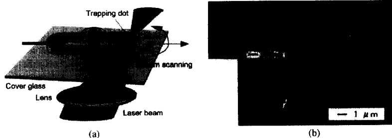
Fig. 10 Optically driven nanoneedle with 2 D.O.F. (a) Driving method (b) SEM image
