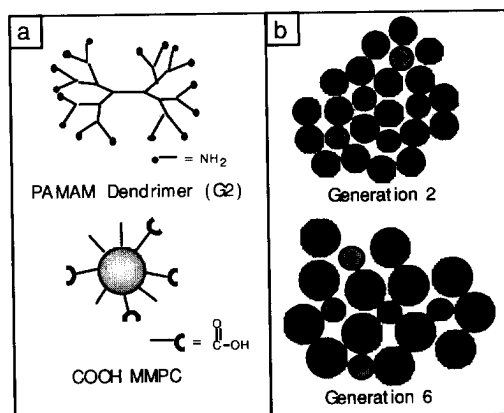
Figure 1. a) Each component of the assembly process possesses complementary bonding units b) As the generation of dendrimer is increased the average interparticle spacing should increase accordingly.
