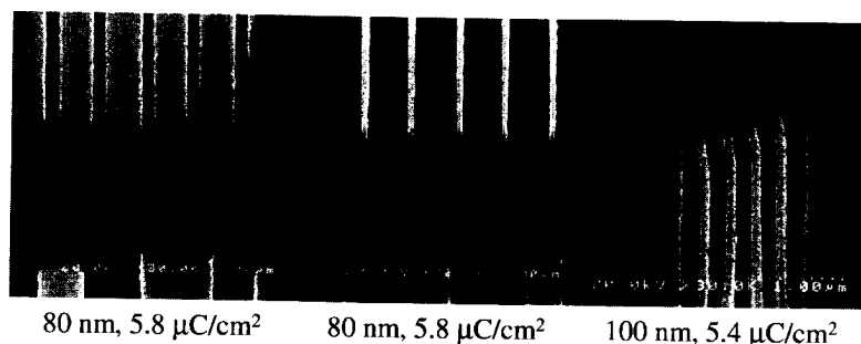
Figure 7. Results obtained from chemically amplified resist (TOK EP004, positive, and EN009, negative) exposed on the SCALPEL® system.
