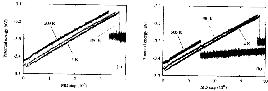
Figure 2. The transitions of the potential energies of the nanowires. The elongation speed is (a) 1.95 m/s, and (b) 0.391 m/s.
