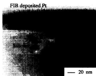
Figure 4. BF TEM image of a cross-section of a FIB milled line.
