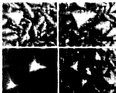
Fig.4 SEM plan view images of Co thin films, as a function of substrate bias (a)-30V (b)-40V (c)-50V (d)-60V.
