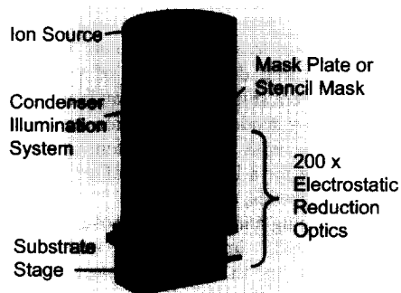
Figure 7 PROFIB principles
