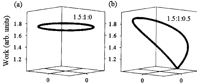
Figure 5. Work of adhesion ( W_A(R;p;\Delta) ) of a metal droplet to a nanowire as a function of droplet radius ( R ), nanowire radius ( p ), and the offset of the center of mass of the droplet from the axis of the nanowire ( \Delta ). The work of adhesion has been calculated for (a) (1.5:1.0:0.0), (b) (1.5:1.0:0.5), where all of the variables ( R;p;\Delta ) have been normalized to the radius of the nanowire.
