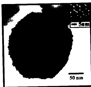
Figure 2. A representative TEM micrograph for a sample of a TTE-Au nm assembly cast on carbon-coated Cu-grid. Insert: TOA + Br - capped Au nm precursors.
