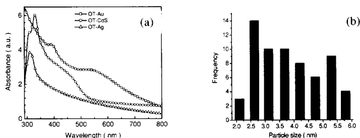
Figure 1. (a) UV-Visible spectra from OT-capped nanocluster assemblies of —△— Ag; —□— Au; and —○— CdS. (b) Particle size distribution obtained from transmission electron microscopy (TEM) measurements.
