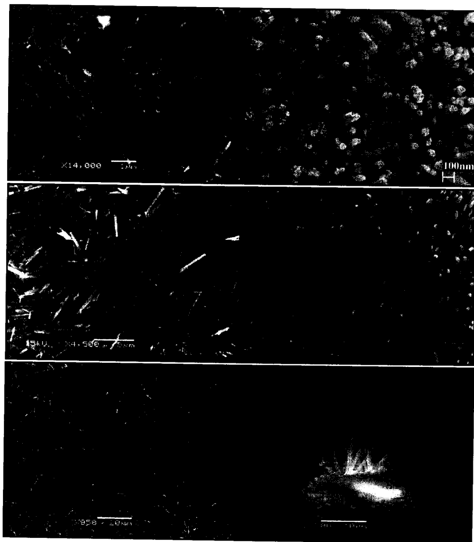
Figure 2. SEM pictures of 3-D arrays of \alpha\text{-Fe}_2\text{O}_3 (top), ZnO (center), and \gamma\text{-MnOOH} (bottom) grown by aqueous chemical growth. The arrays consist of 1-D nanorods oriented parallel (left) and perpendicular (right) onto the substrates.
