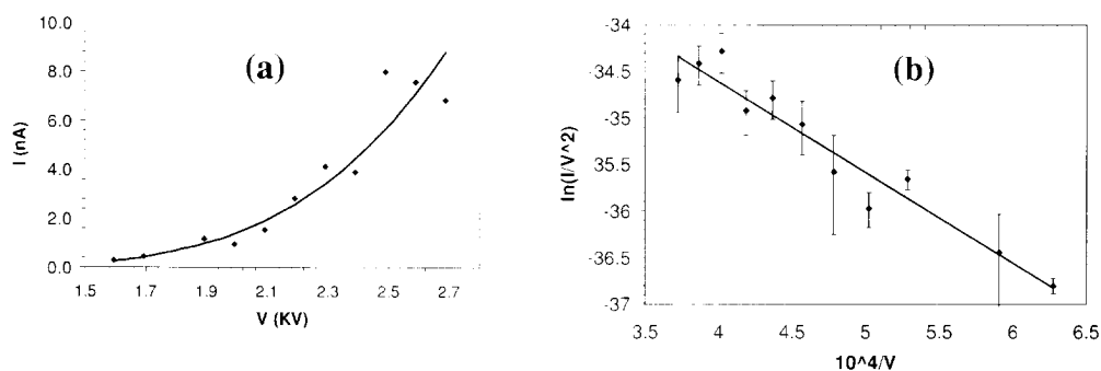
Figure 5. (a) shows the current-voltage behavior of a \text{SiO}_2 nanowire, (b) is its corresponding Fowler-Nordheim plot.
