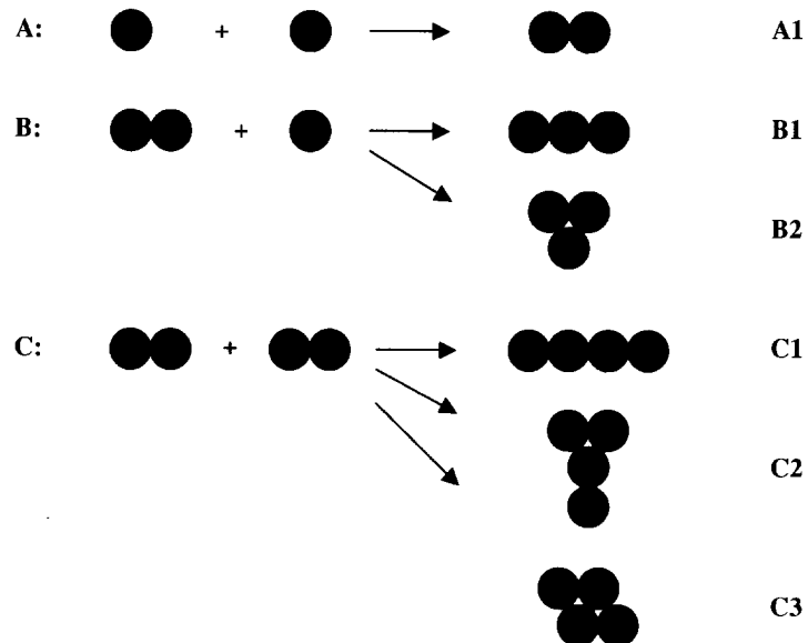
Figure 1. Model for the first steps of coagulation. The procedure leading to axial arrangement of doublets C; C1 represents the general tendency of 1D structure of particles formation. The procedure leading to lateral arrangement of doublets C; C3 represents the general tendency of 3D structure of particles formation.
