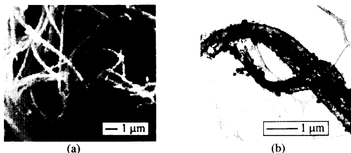
Fig. 2. SEM (a) and TEM (b) images of carbon tubes resulted from heat treatment of PPy/PMMA composite fibers.
