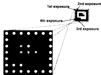
Figure 8 Electrostatic step exposure (ESE)
