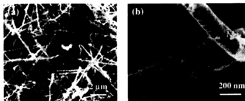
Figure 2. (a) is an SEM overview of \text{CdS/SiO}_2 composite nanowires. (b) is a high resolution SEM image of \text{CdS/SiO}_2 composite nanowires.
