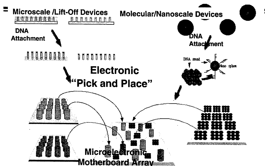
Figure 4.6. Directed nanofabrication on a chip (Nanogen, Inc.).
