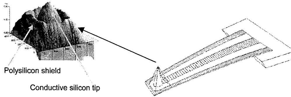
Figure 3.12. Near field antenna probe (after van der Weide and Neuzil 1996; reprinted by permission; ©1996 American Vacuum Society).
