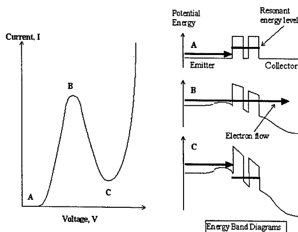
Figure 6.11. Resonant tunneling device (Moffat 1999).
