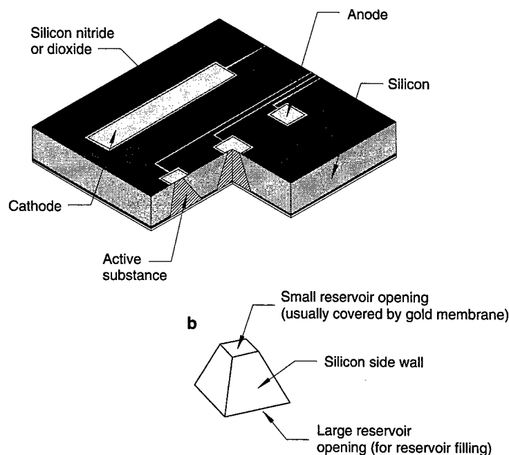
Figure 8.4. Prototype of a microchip device for drug delivery (reprinted by permission from Nature , Santini et al. 1999, ©1999, Macmillan Magazines Ltd.).
