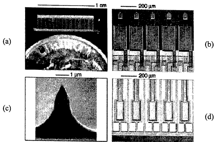
Figure 3.5. An array of cantilevers with integrated actuators and sensors with improved shielding between the actuator and sensor: (a) shows an entire array of 50 cantilevers spanning 1 cm next to a dime; (b) shows a detail of five cantilevers, spaced by 200 \mu\text{m} ; (c) is an SEM of a typical integrated single-crystal silicon tip (radius of curvature is below 10 nm); and (d) shows the corresponding electrical contact structure for the cantilevers. There are three leads per device: piezoresistor, ZnO, and tip bias (reprinted by permission from Minne et al. 1998; ©1998 American Institute of Physics).
