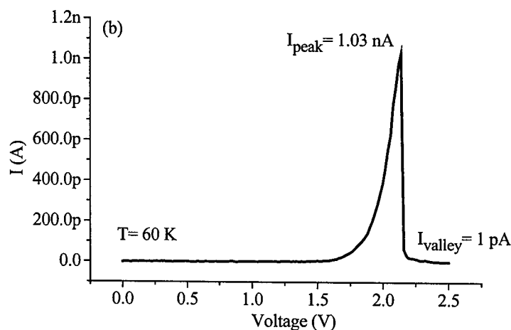
Figure 6.7. I-V characteristics of the Au-(2'-amino-4-ethynylphenyl-4'-ethynylphenyl-5'-nitro-1-benzenethiolate)-Au devices at 60 K. The peak current density is \sim 50\text{ A/cm}^2 , the NDR is \sim 400\text{ }\mu\Omega\text{-cm}^2 , and the PVR is 1030:1 (reprinted with permission from Chen et al. 1999, ©1999 American Association for the Advancement of Science).
