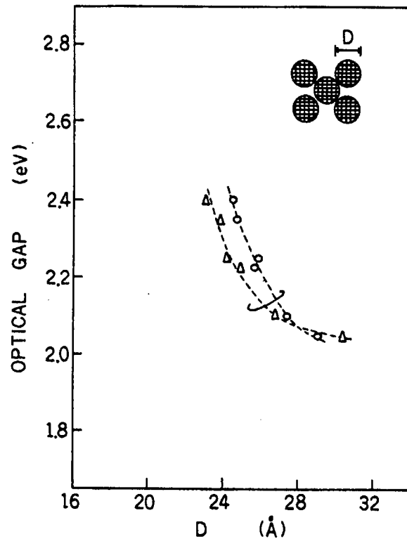
Figure 2.9. Experimental optical gaps for silicon quantum dots. D is the diameter of the dot. The results are from Furukawa and Miyasoto (1988). The two sets of experimental data represent different estimates for the size of the dots.
