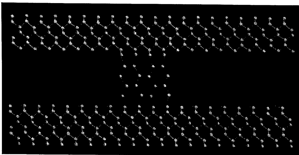
Figure 2.6. An atomistic \text{SiO}_2 quantum dot bridging between two silicon surfaces.
