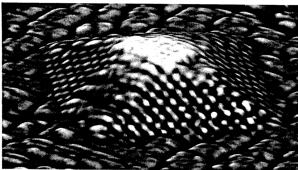
Figure 1.1. STM image of quantum dot formed by self-assembling (Ge “pyramid”) (courtesy Hewlett-Packard; image acquired by G. Medeiros-Ribeiro, Hewlett-Packard Labs).
