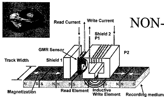
Magnetic recording process.
