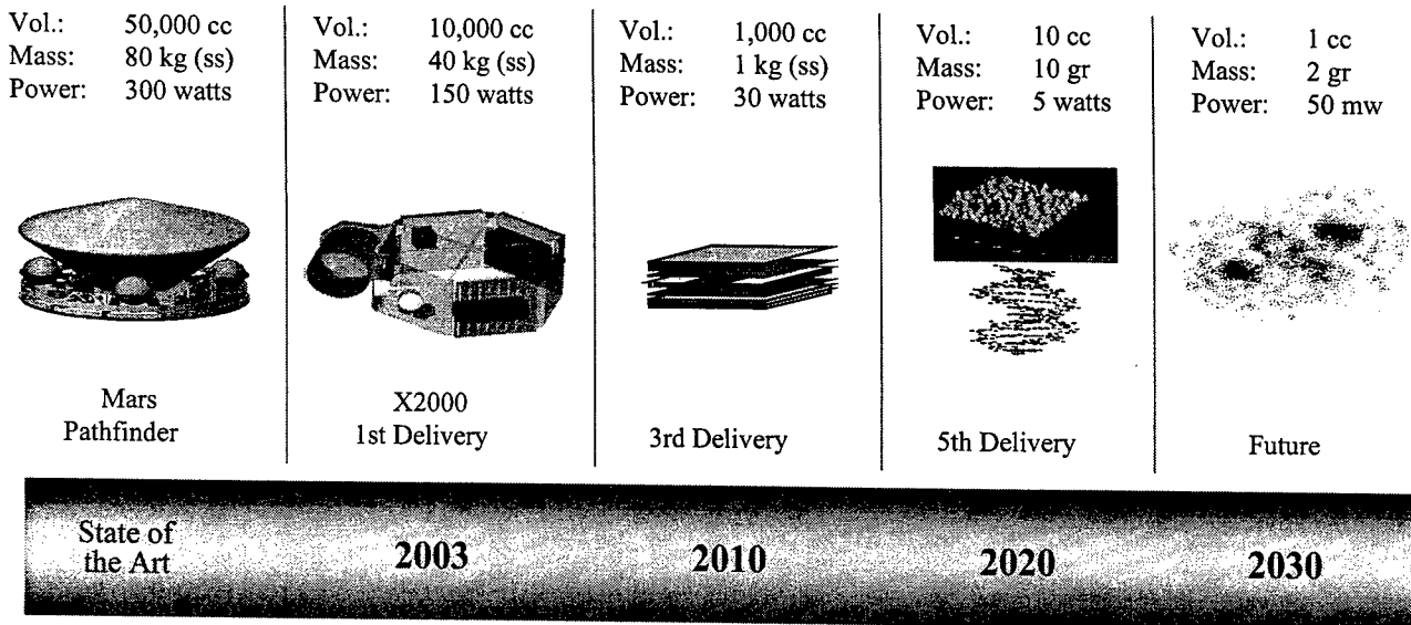
Figure 6.13. Avionics roadmap.
