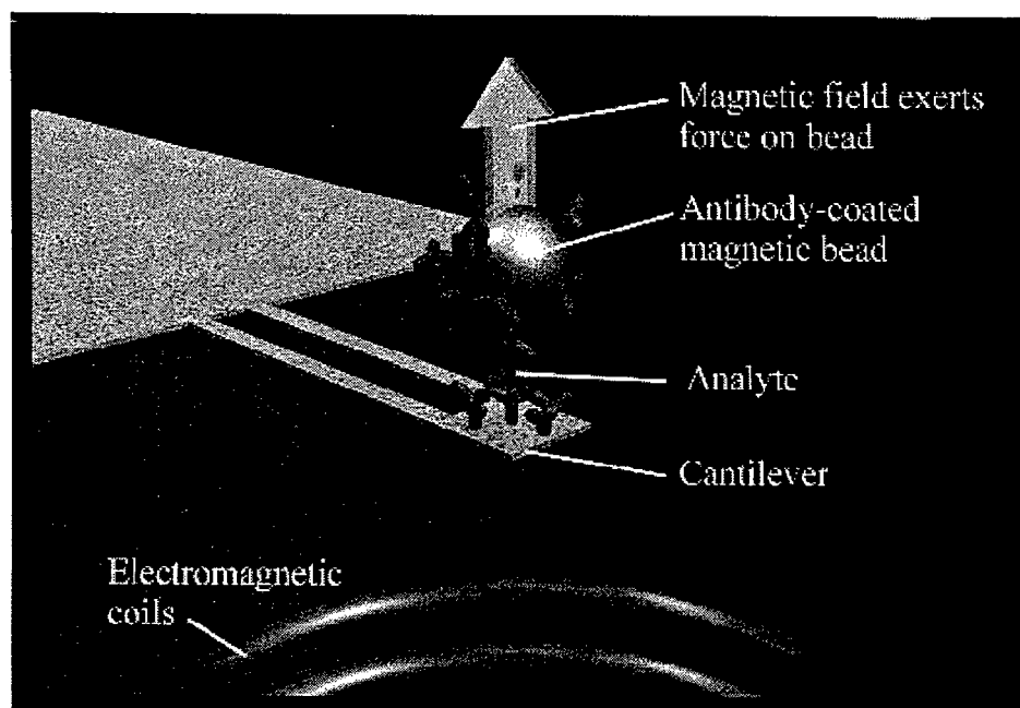
Figure 8.9. Atomic force microscope (AFM) immunoassay (courtesy Naval Research Laboratory; reprinted with permission from Baselt et al. 1996, ©1996 American Vacuum Society).
