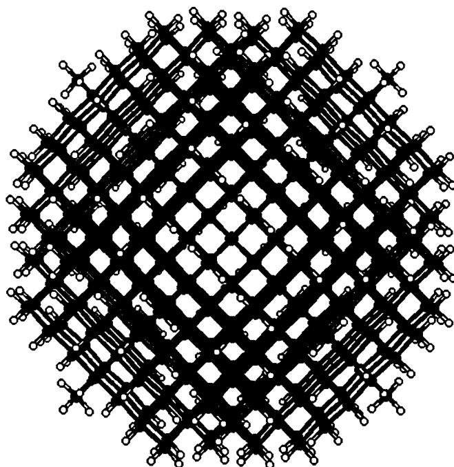
Figure 2.8. Ball and stick model of \text{Si}_{575}\text{H}_{276} . The white dots correspond to H atoms, which passivate the surface of the dot.
