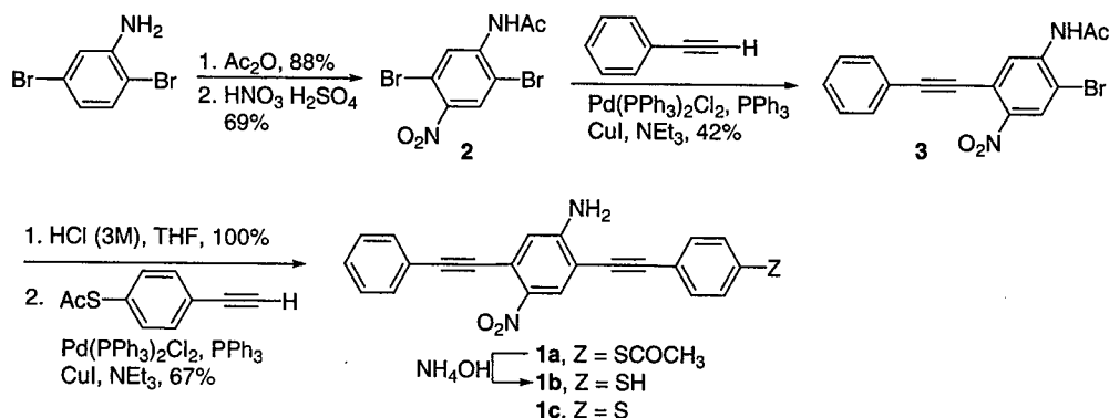
Figure 6.6. Schematic of the synthesis of the active molecular compound and its precursors ( 1a-c ).
