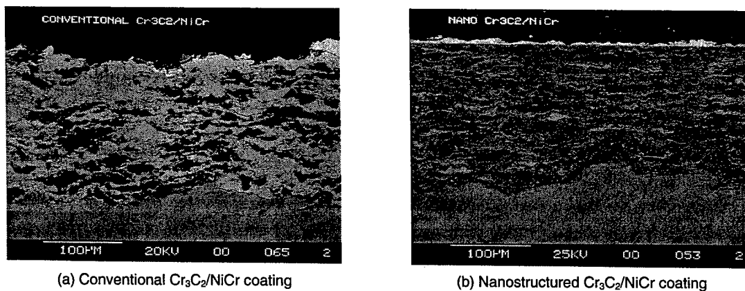
Figure 7.5. SEM morphology of conventional and nanostructured coatings.
