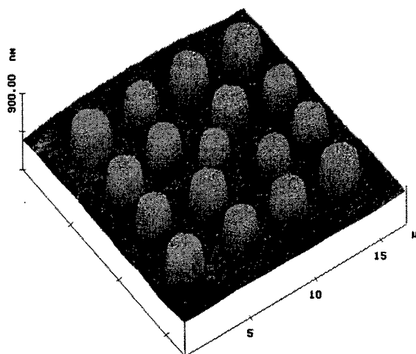
Figure 4.5. AFM image of PMMA LISA pillar array formed under a square pattern (reprinted with permission from Chou and Zuang 1999, ©1999 American Vacuum Society).
