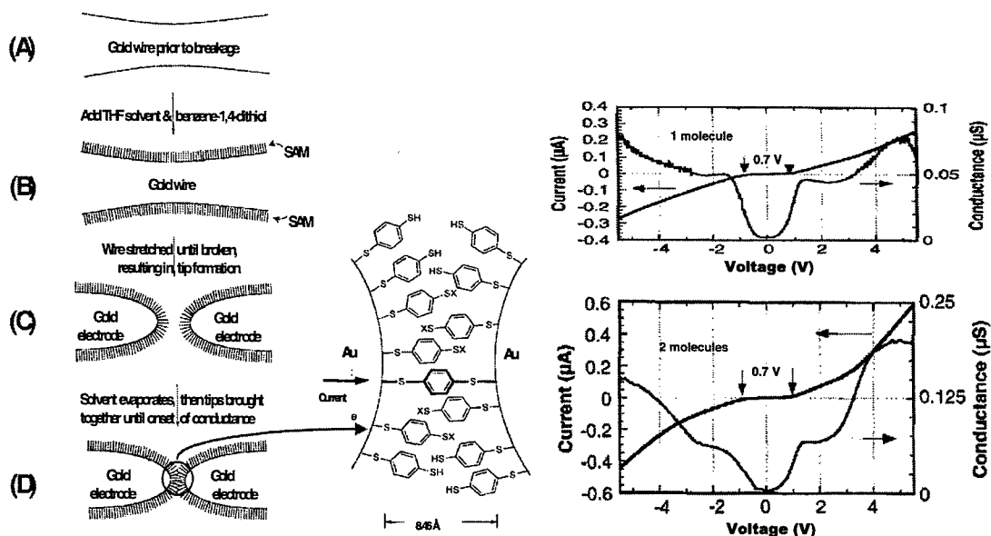
Figure 6.1. Organic nanostructures: on left, showing self-assembly of benzene-1,4-dithiol onto Au electrodes; on right, showing room-temperature I-V measurements suggesting presence of a Coulomb gap (reprinted with permission from Reed et al. 1997, ©1997 American Association for the Advancement of Science).
