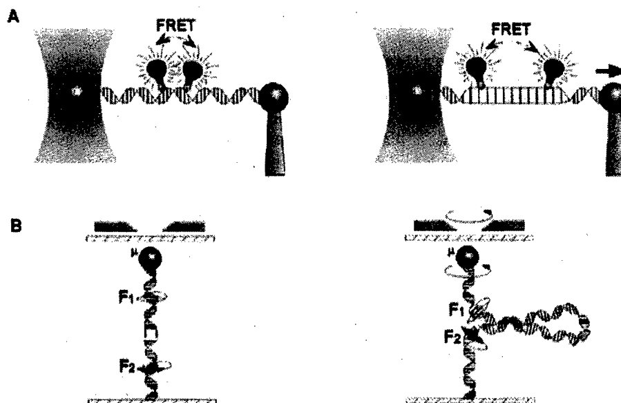
Figure 3.10. Optical tweezer and magnetic bead manipulation coupled with fluorescent probes (FRET) (reprinted with permission from Weiss 1999, ©1999 American Association for the Advancement of Science).
