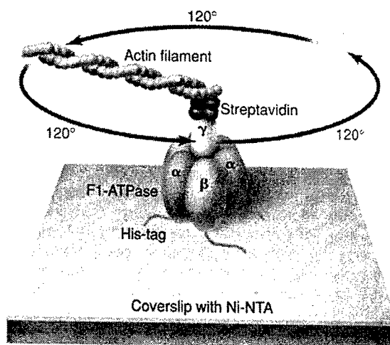
Figure 8.1. The molecular motor protein F1-ATPase. Illustrated here is an experiment reported in Science , in which an actin filament is attached to a motor protein to provide load to and allow visualization of the motor rotation (reprinted with permission from Noji 1998, ©1998 American Association for the Advancement of Science).
