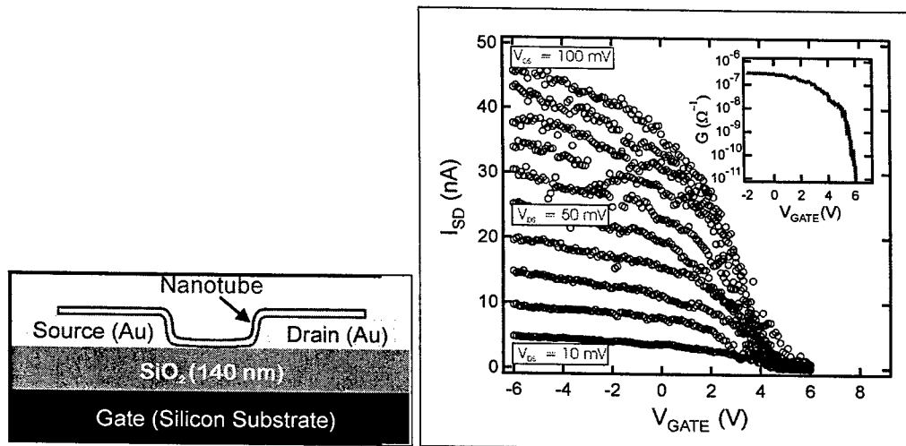
Figure 6.8. Field-effect transistor based on a single 1.6 nm diameter carbon nanotube (adapted from Martel et al. 1998, reprinted by permission; ©1998 American Institute of Physics).
