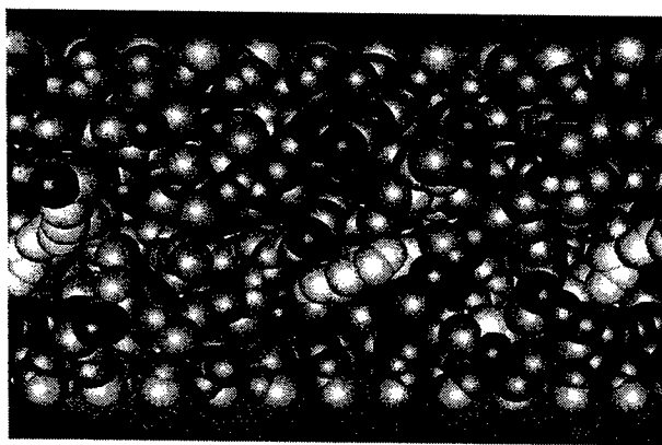
Figure 2.3. Snapshot of squalane under shear flow confined between two walls with tethered butane chains, with wall spacing of 3.6 nm, the same apparent shear rate as in Figure 2.2, core liquid density of 0.82 \text{ g cm}^{-3} , and temperature of 323 K. Sidegroups are shown in gray.
