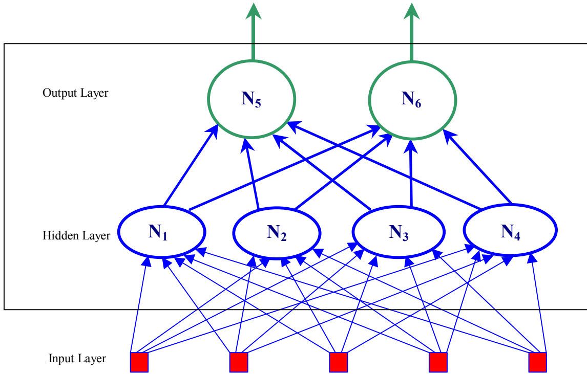
Figure 10. Neural network.
