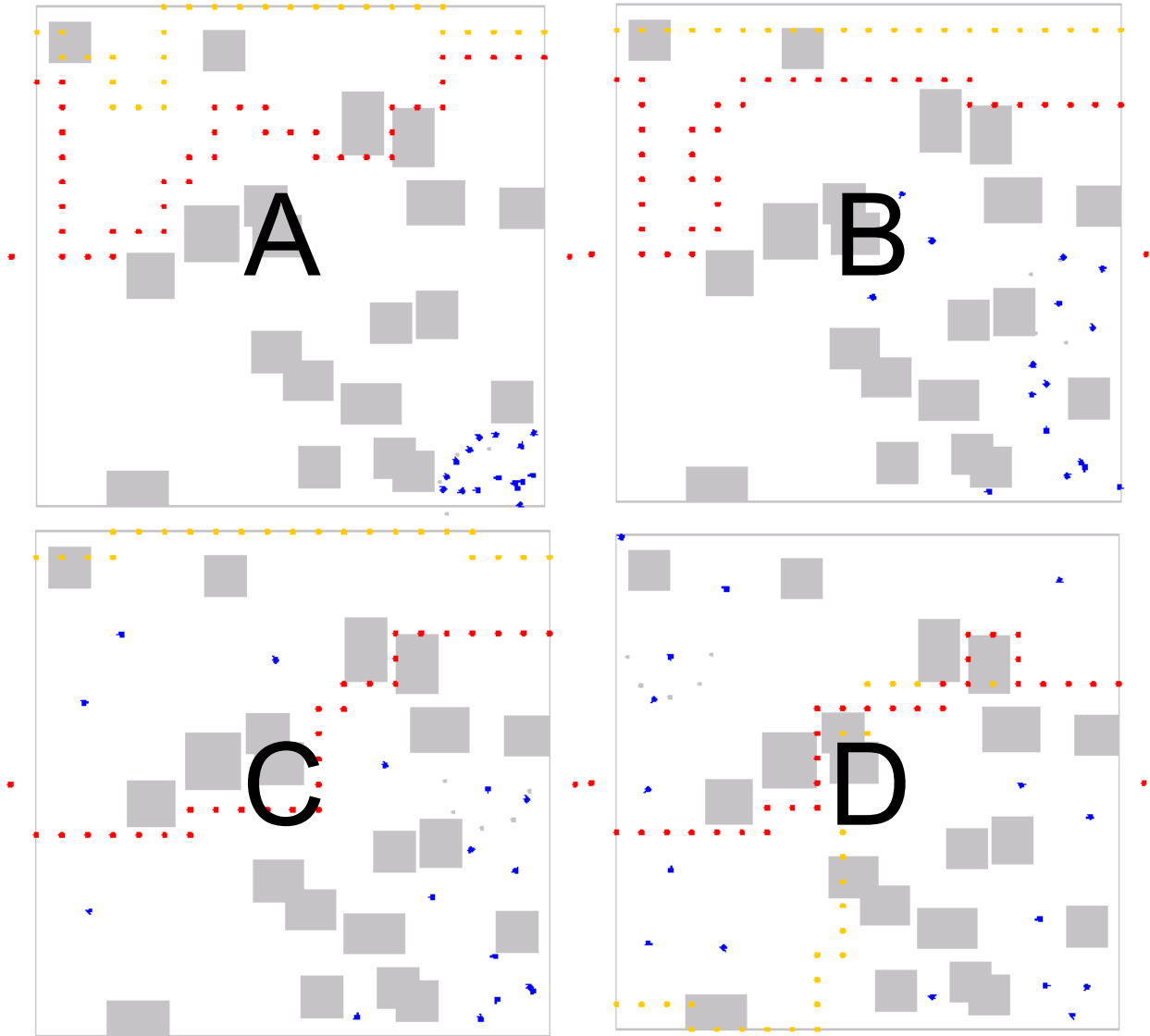
Figure 16. Autonomous deployment for area coverage with obstacles.
