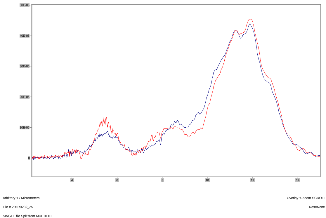
Graph III-5: RS-40 Open Burn IR Spectra
