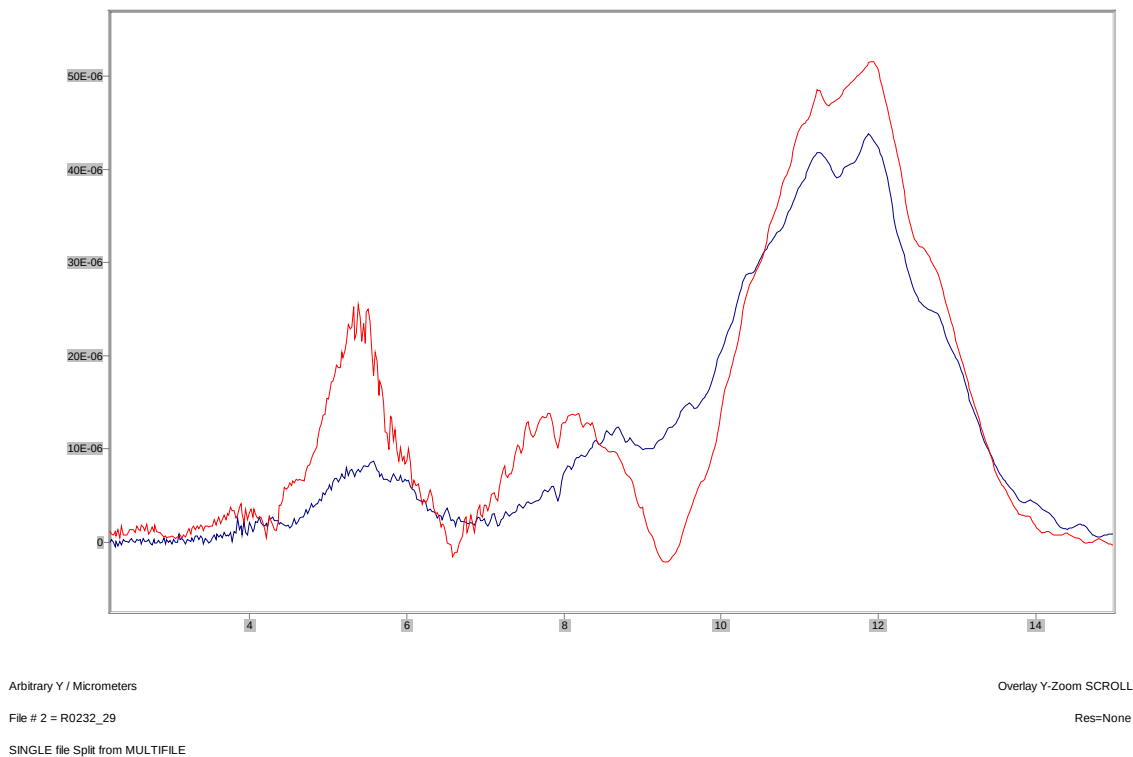
Graph III-6: RS-40 Open Burn IR Spectra
