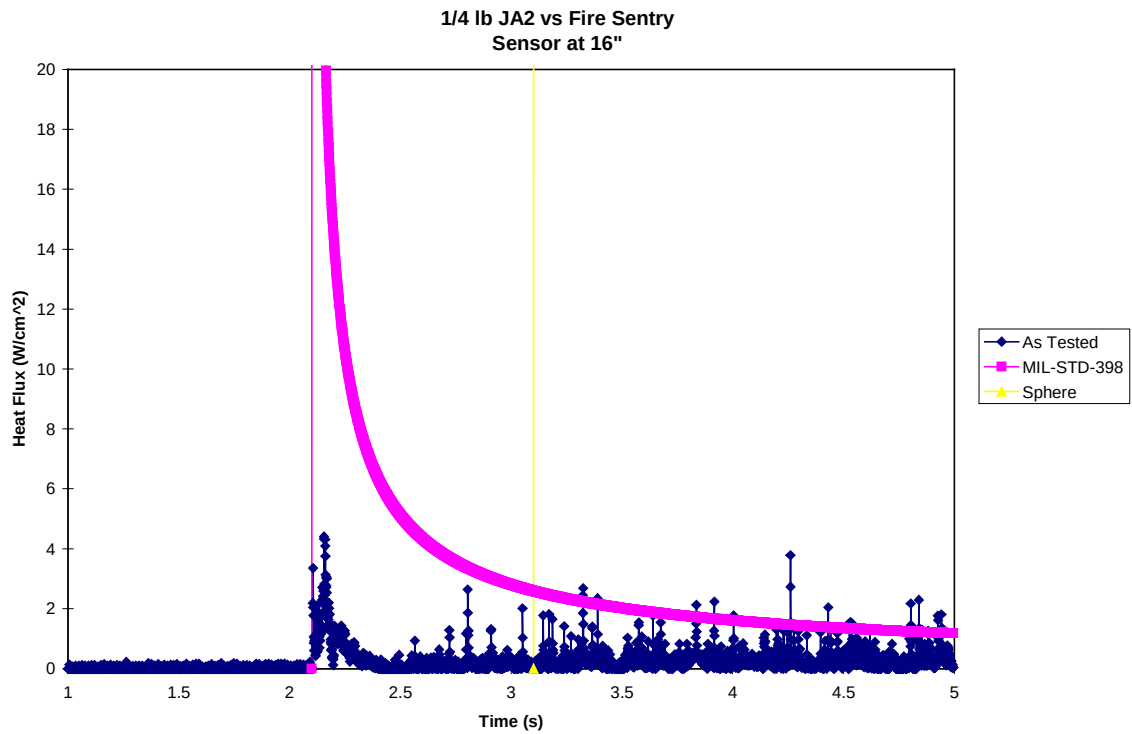
Graph II-29: ¼# JA2 vs Fire Sentry Detectors- Flux Sensor @ 16"
