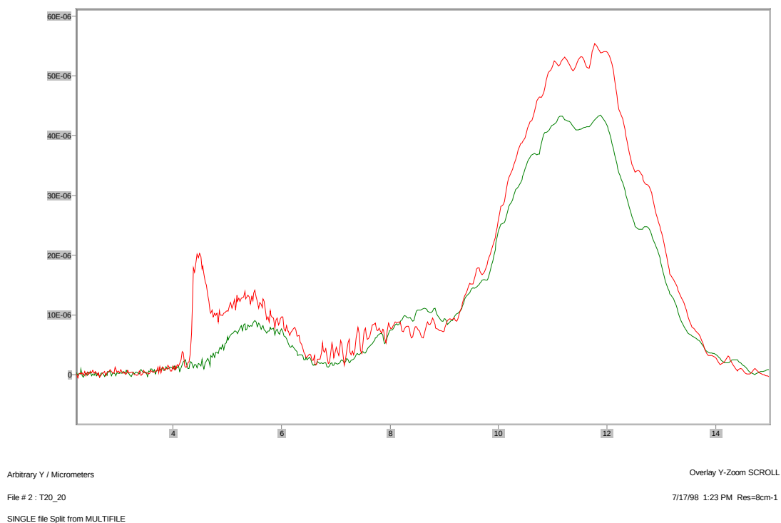
Graph III-83: UTP-31,500 Open Burn IR Spectra
