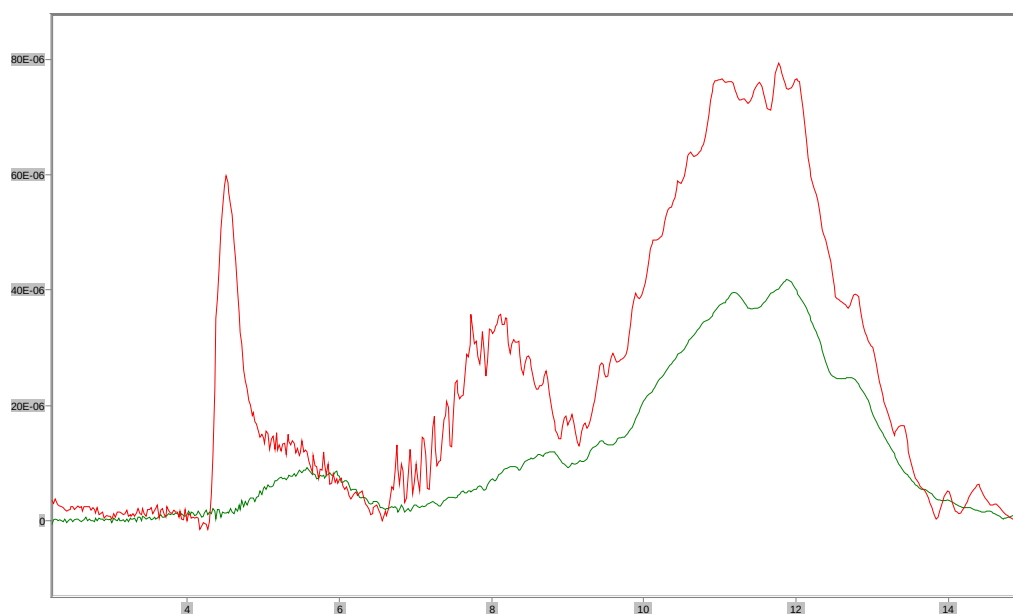
Graph III-79: UTP-25201C Open Burn IR Spectra
