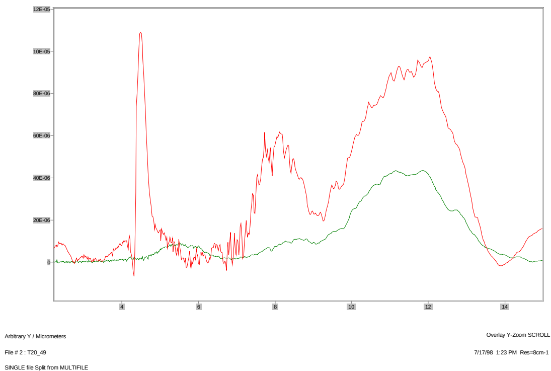
Graph III-84: UTP-31,500 Open Burn IR Spectra
