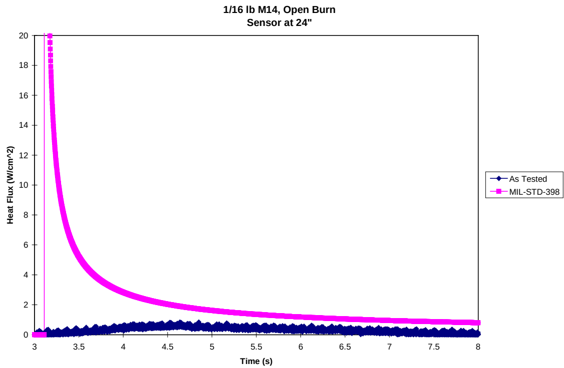
Graph II-10: 1/16# M14 Open Burn
