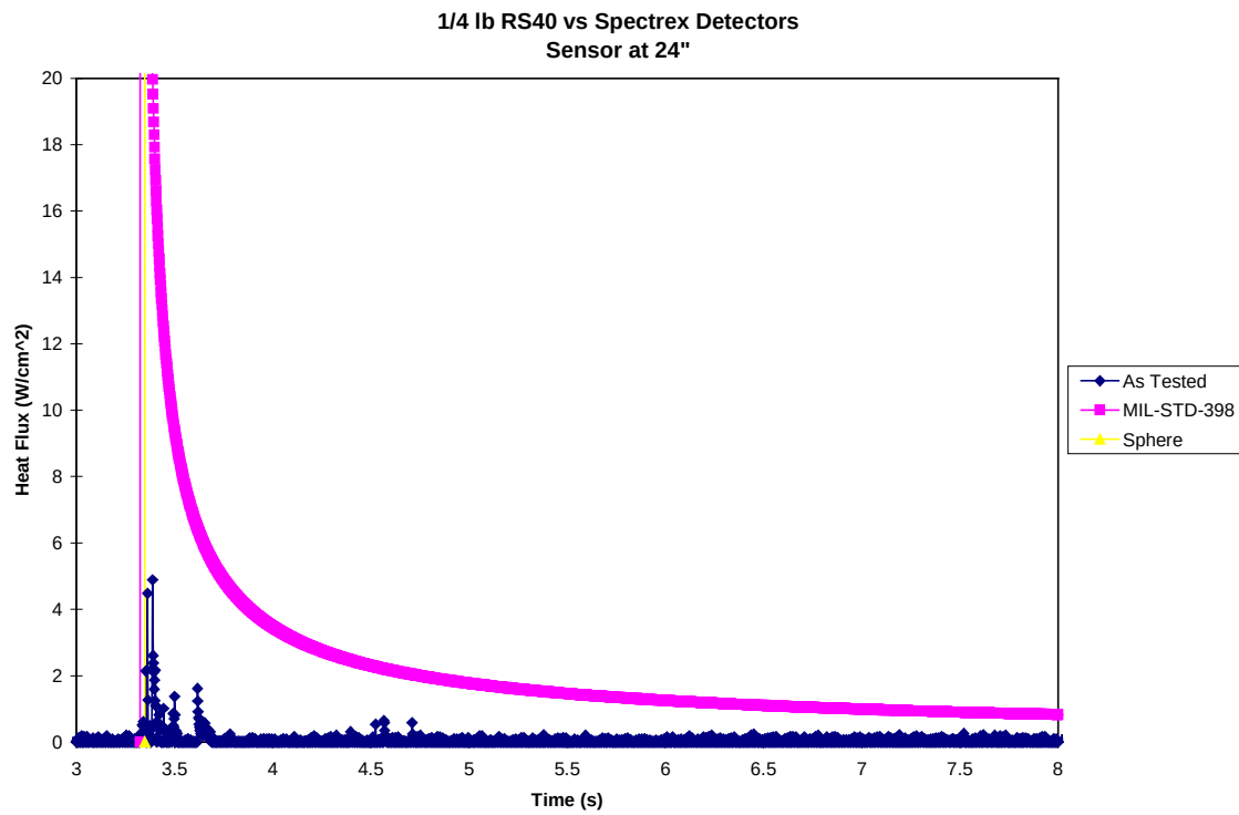
Graph II-23: ¼# RS-40 vs Spectrex Detectors - Flux Sensor @ 24”
