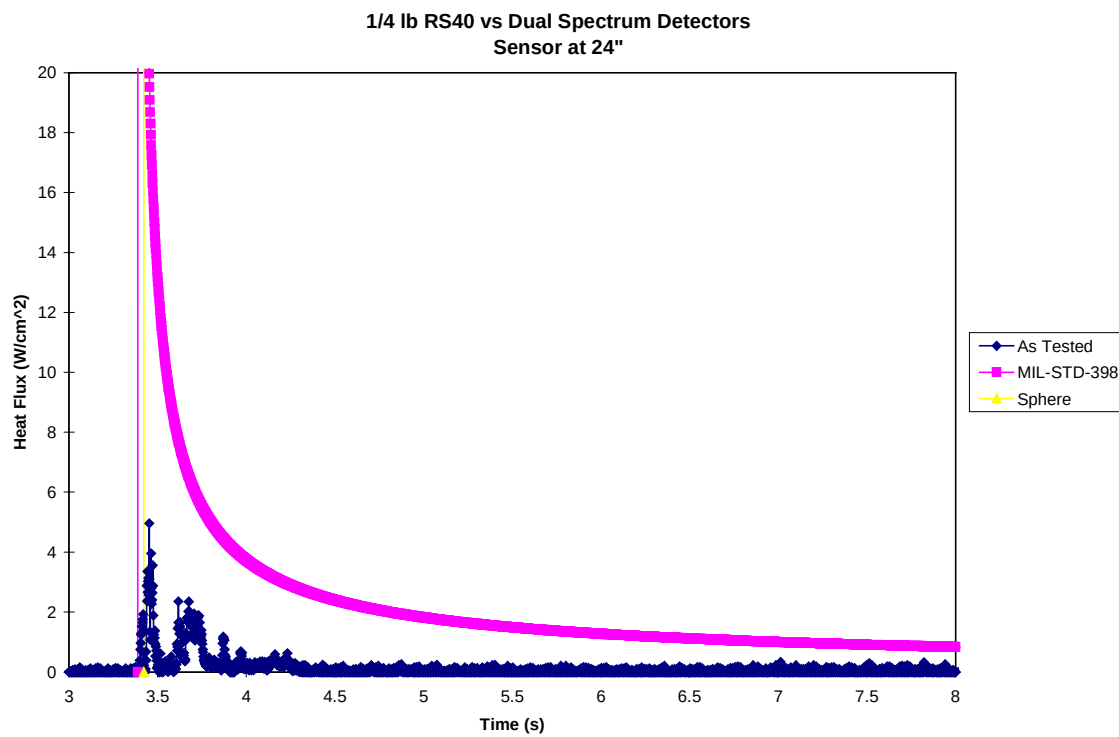
Graph II-24: ¼# RS-40 vs Dual Spectrum Detectors - Flux Sensor @ 24”
