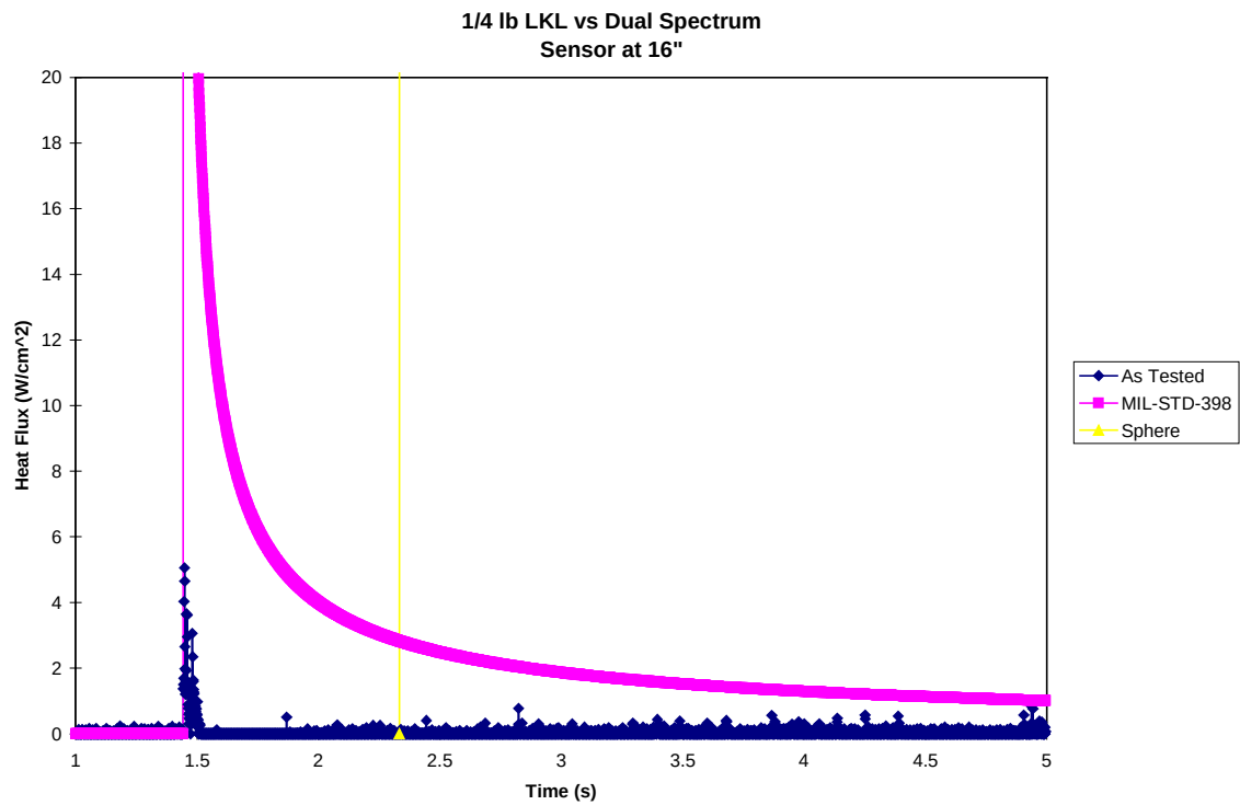
Graph II-30: ¼# LKL vs Dual Spectrum Detectors - Flux Sensor @ 16"
