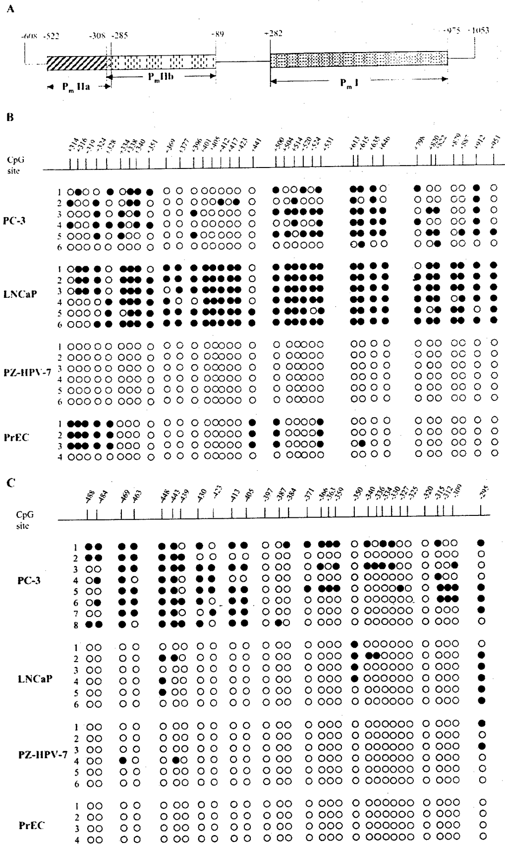
FIG. 6. Characterization of the methylation status of the hDAB2IP gene promoter in human prostatic epithelial cells. A, schematic representation of the three separated positions in the hDAB2IP locus subjected to bisulfite sequencing analysis. B and C, methylation patterns in the PmI (+282 to +975) and PmIIa (-522 to -285) regions in human prostatic epithelial cells. High molecular mass DNA isolated from each sample was modified with sodium bisulfite and amplified by PCR using the primer sets indicated in Table I. The PCR product was subcloned, and each individual clone (horizontal rows) from every sample was sequenced. The position of each CpG dinucleotide (vertical bars) is labeled with the number representing its location in the hDAB2IP gene. ○, unmethylated CpG; ●, methylated CpG.
