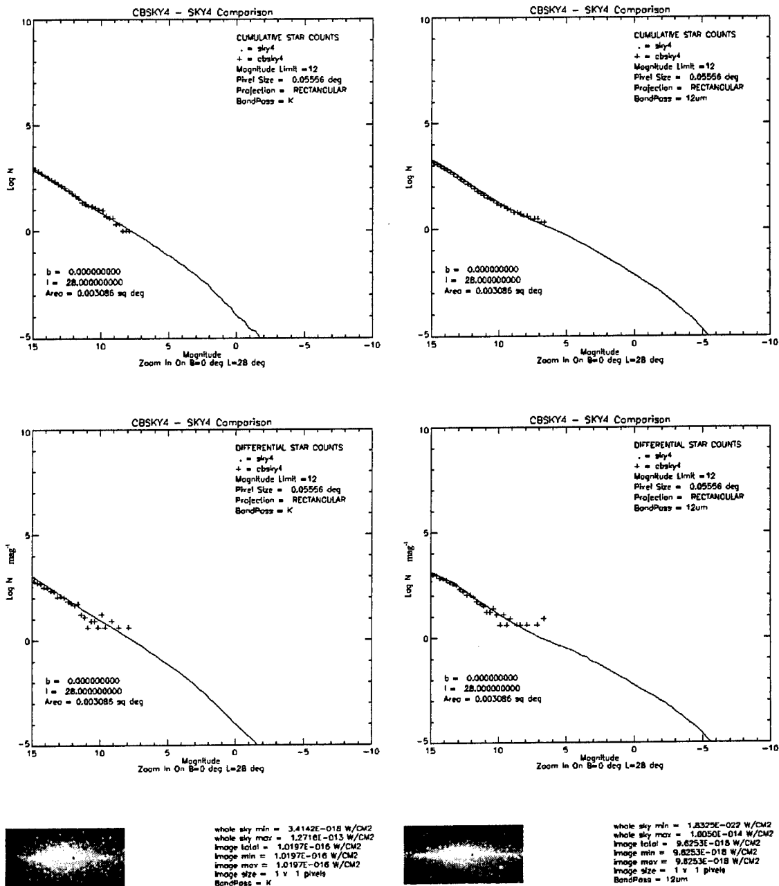
Figure C.46: SKY4 - CBSKY4 comparison for 0.0556 deg around l = 0.0 , b = 28.0 .
