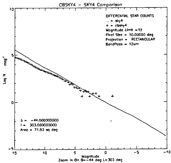
Figure E.8: SKY4 - CBSKY4 comparison for 10.0 deg around the SMC.
