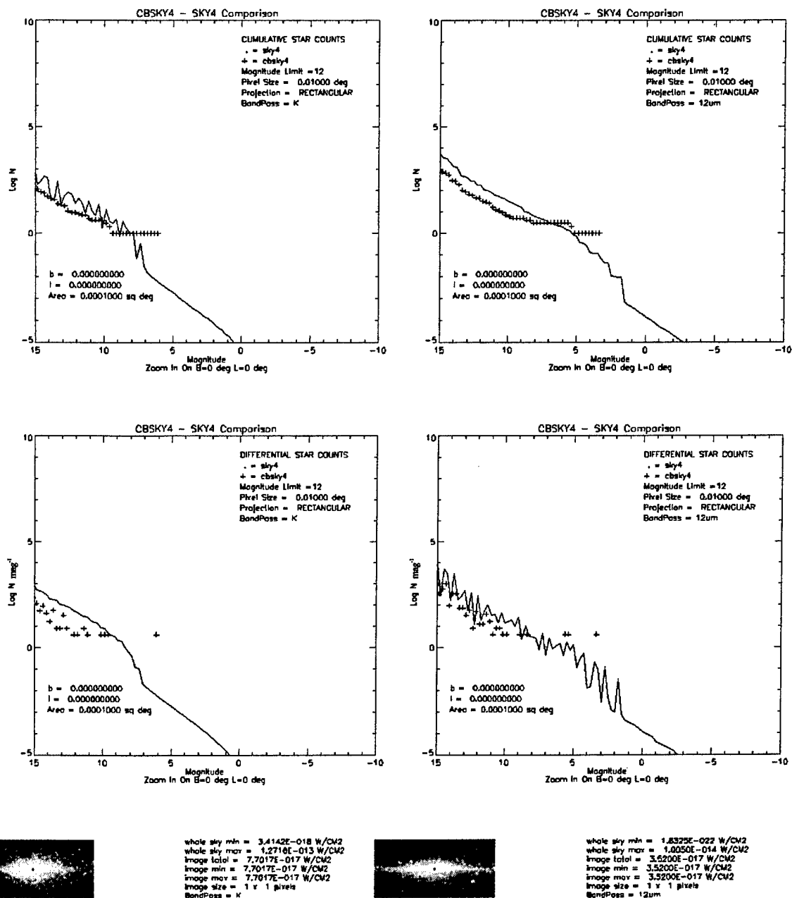
Figure 2: SKY4 - CBSKY4 comparison for l = 0.0 , b = 0.0 .
