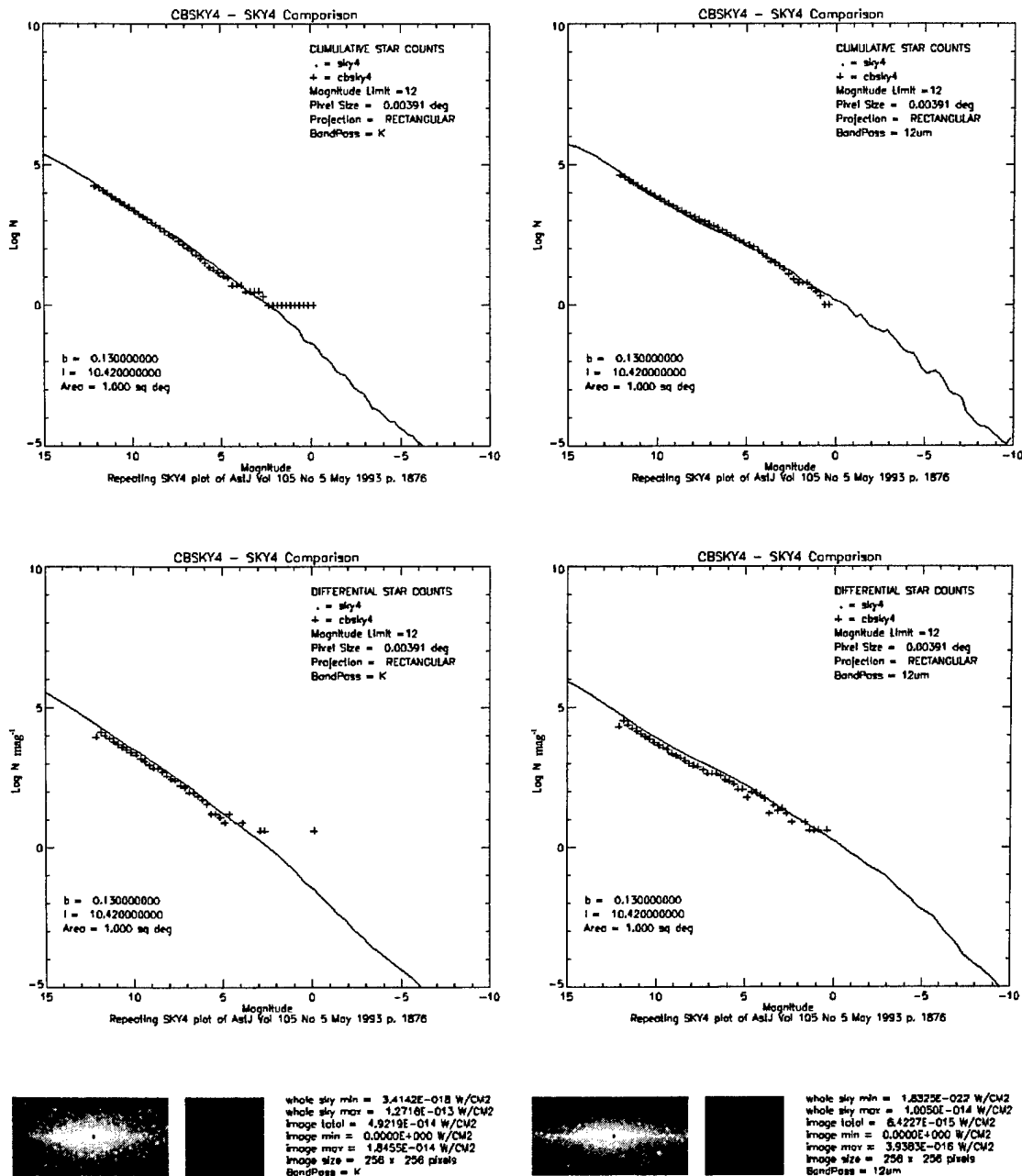
Figure A.3: SKY4 - CBSKY4 comparison for l = 10.42 , b = 0.13 .
