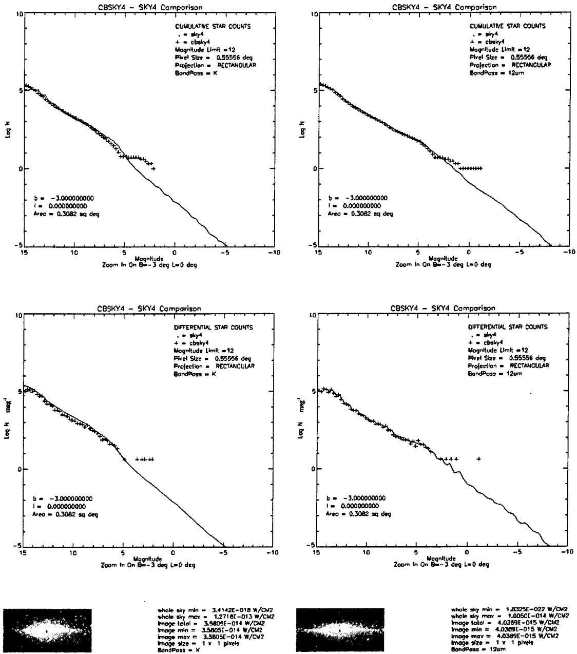
Figure C.4: SKY4 - CBSKY4 comparison for 0.556 deg around l=3.0 , b = 0.0 .
